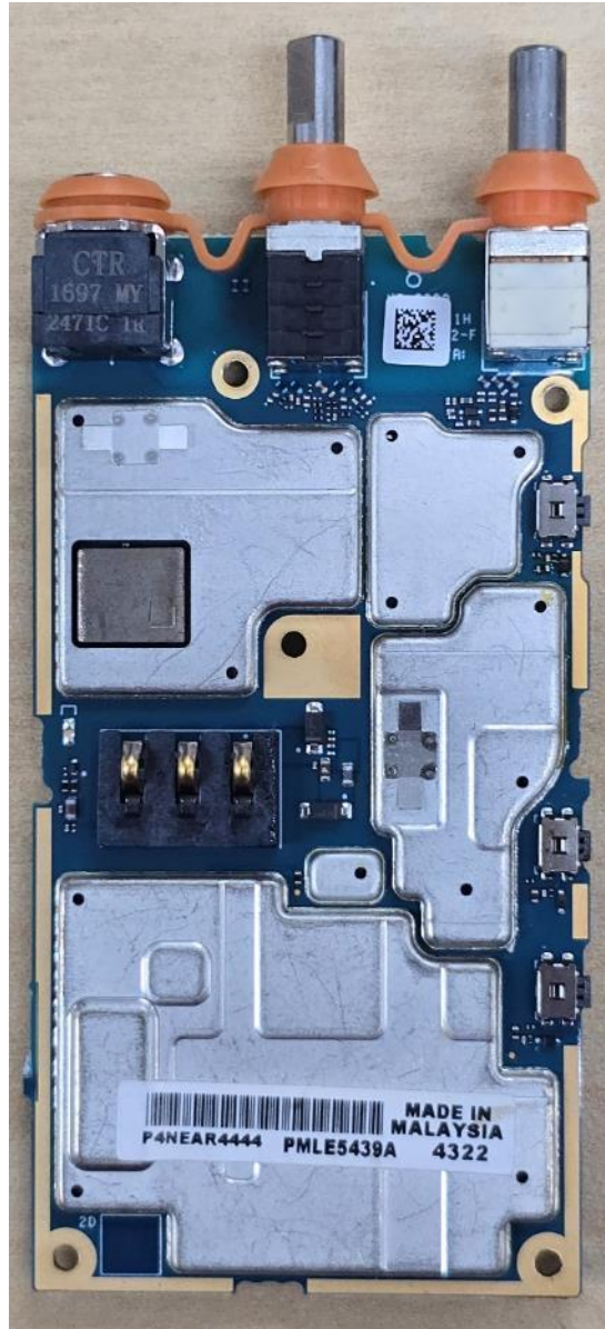
RF board with Shields (Bottom) of NKP Model
