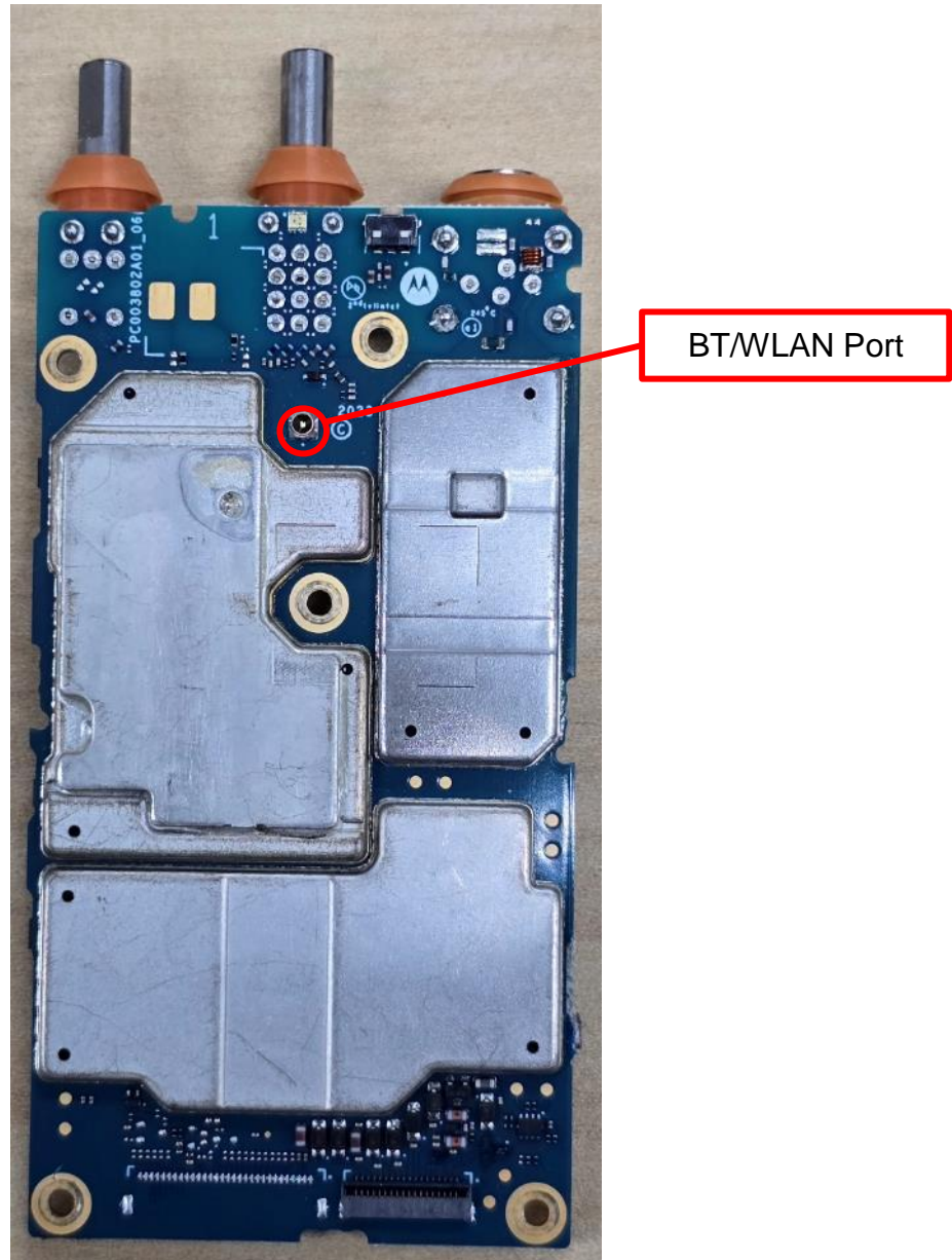
RF board with Shields (Top) of NKP Model
