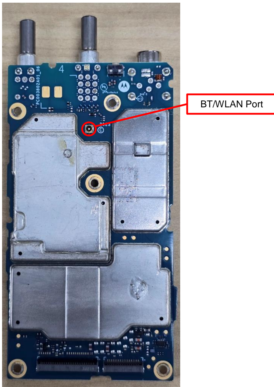
RF board with Shields (Top) of LKP Model
