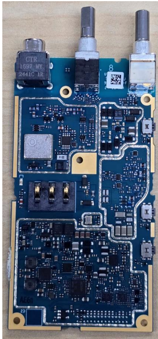
RF board without Shields (Bottom) of NKP Model
