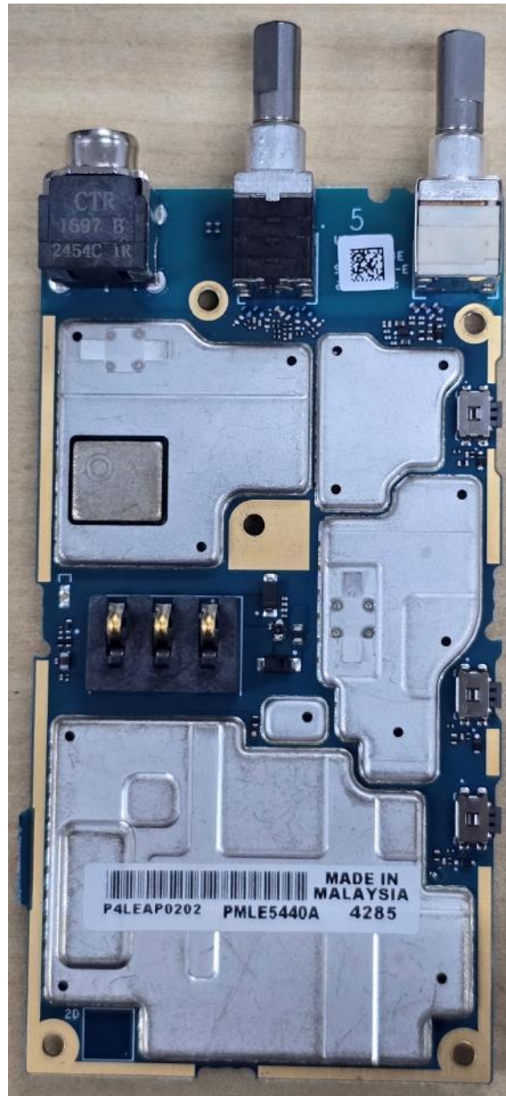
RF board with Shields (Bottom) of LKP Model
