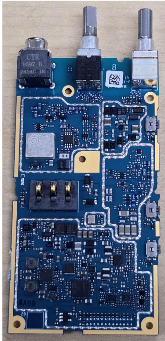
RF board without Shields (Bottom) of LKP Model
