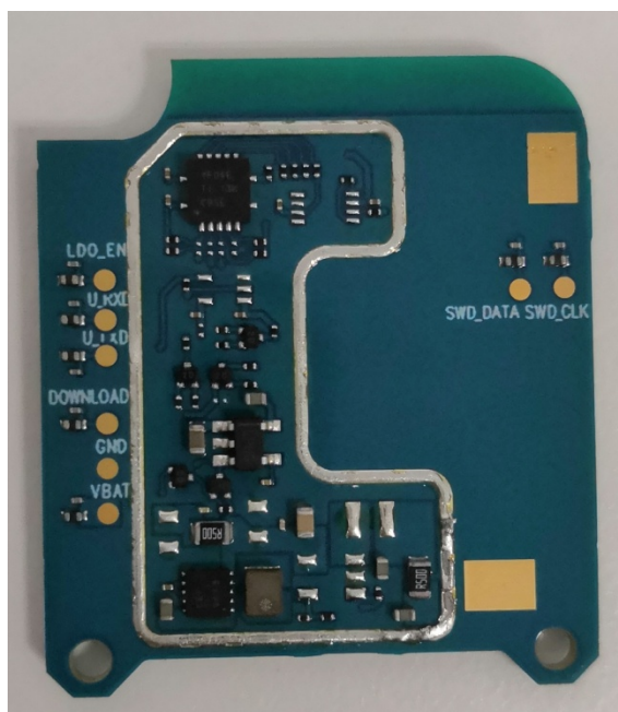
EXHIBIT 9H - WIFI board without Shields (Top)
