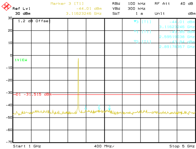
Date: 29.AUG.2019 03:35:25 Conducted Emissions. 802.11n, Frequency 2437 MHz Emission Level, 1 GHz -> 5 GHz
