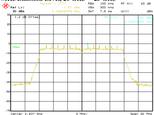
Date: 29.AUG.2019 03:33:37 Conducted Emissions. 802.11n, Frequency 2437 MHz Reference Level
