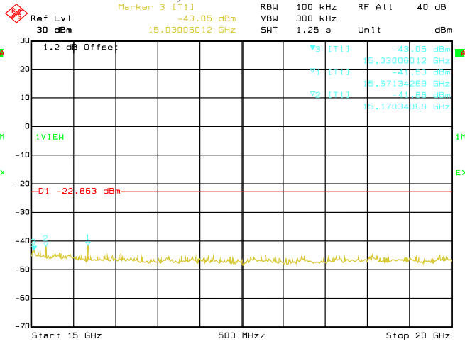
Date: 29.AUG.2019 02:48:20 Conducted Emissions. 802.11b, Frequency 2462 MHz Emission Level, 15 GHz -> 20 GHz
