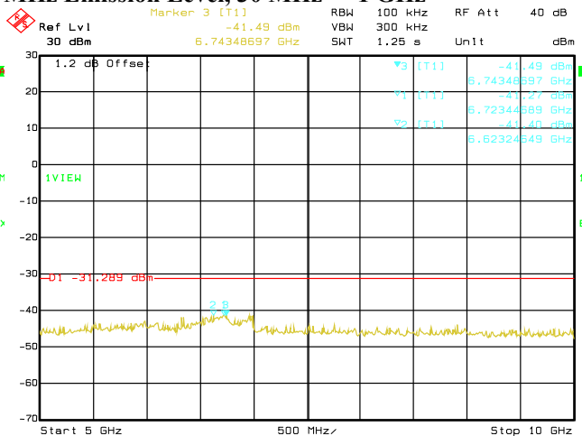
Date: 29.AUG.2019 03:44:00 Conducted Emissions. 802.11n, Frequency 2462 MHz Emission Level, 5 GHz -> 10 GHz
