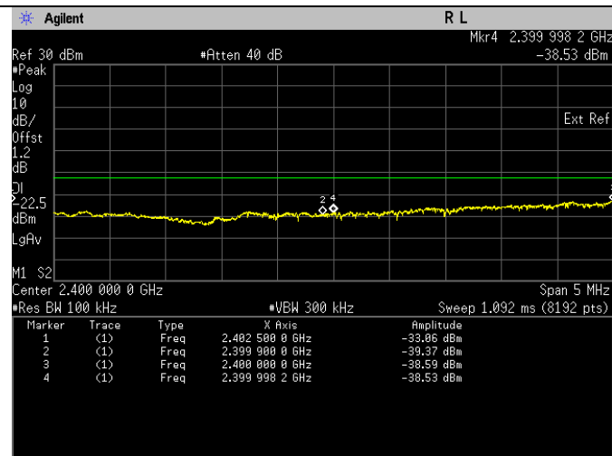
Band Edge. 802.11b Frequency 2412 MHz Band Edge
