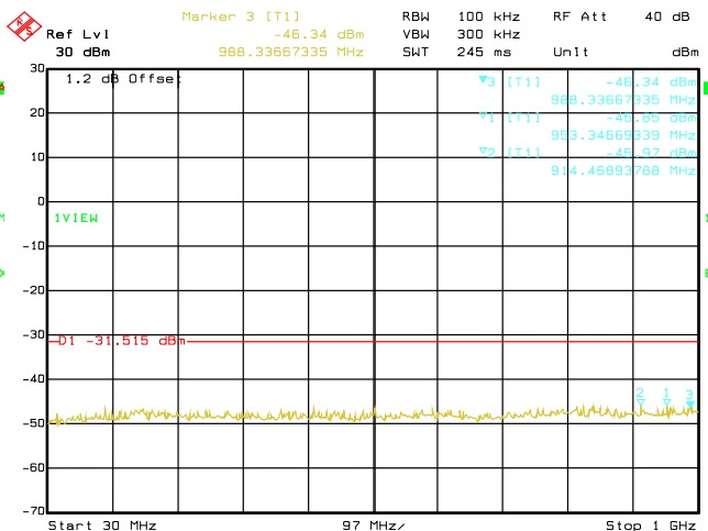
Date: 29.AUG.2019 03:34:31 Conducted Emissions. 802.11n, Frequency 2437 MHz Emission Level, 30 MHz -> 1 GHz
