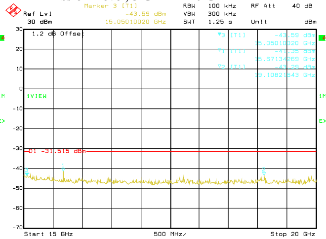
Date: 29.AUG.2019 03:38:05 Conducted Emissions. 802.11n, Frequency 2437 MHz Emission Level, 15 GHz -> 20 GHz
