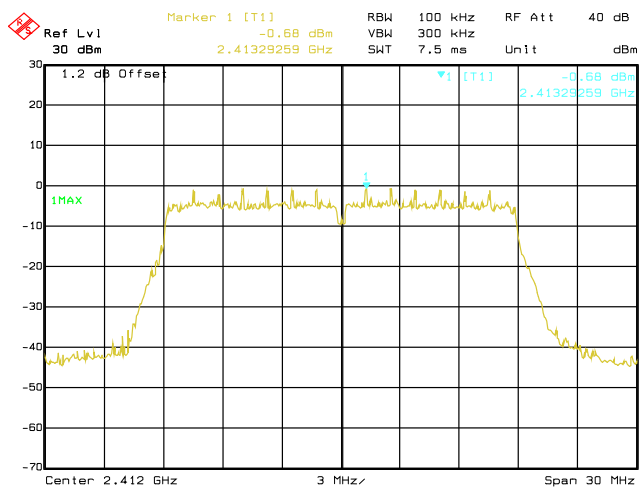
Date: 29.AUG.2019 03:21:32 Conducted Emissions. 802.11n, Frequency 2412 MHz Reference Level
