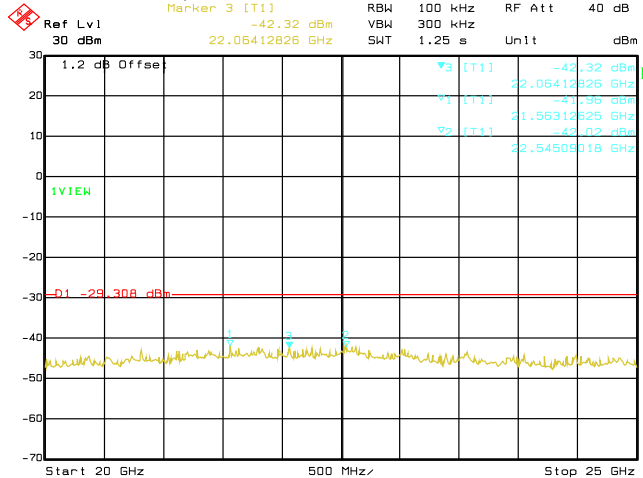
Date: 29.AUG.2019 03:04:44 Conducted Emissions. 802.11g, Frequency 2437 MHz Emission Level, 20 GHz -> 25 GHz
