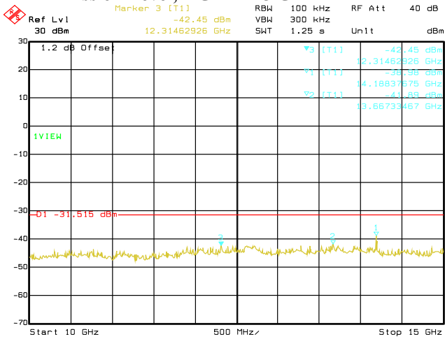
Date: 29.AUG.2019 03:37:11 Conducted Emissions. 802.11n, Frequency 2437 MHz Emission Level, 10 GHz -> 15 GHz
