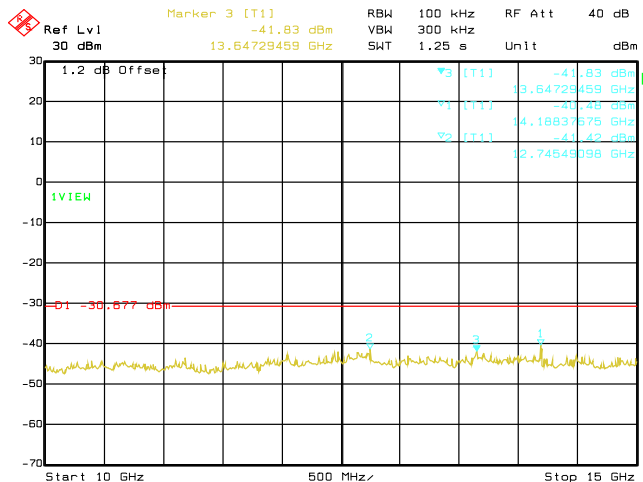
Date: 29.AUG.2019 03:25:07 Conducted Emissions. 802.11n, Frequency 2412 MHz Emission Level, 10 GHz -> 15 GHz
