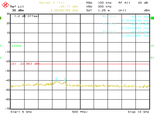
Date: 29.AUG.2019 02:46:34 Conducted Emissions. 802.11b, Frequency 2462 MHz Emission Level, 5 GHz -> 10 GHz
