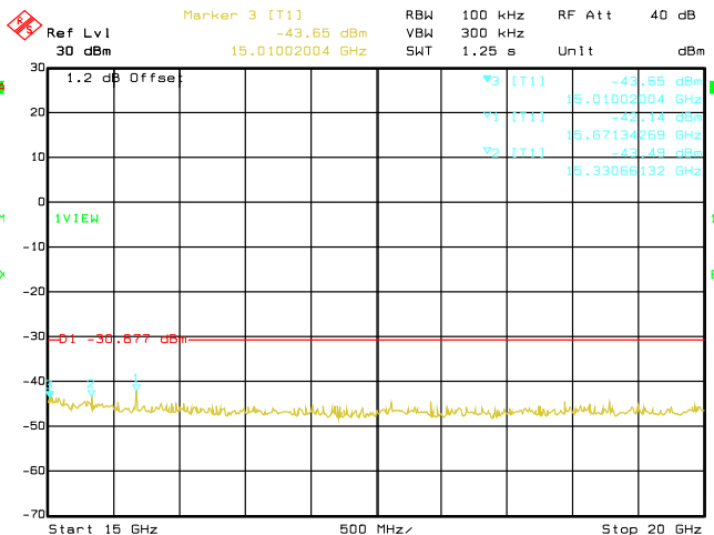
Date: 29.AUG.2019 03:26:00 Conducted Emissions. 802.11n, Frequency 2412 MHz Emission Level, 15 GHz -> 20 GHz
