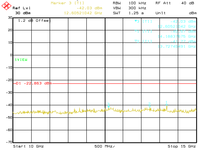
Date: 29.AUG.2019 02:47:27 Conducted Emissions. 802.11b, Frequency 2462 MHz Emission Level, 10 GHz -> 15 GHz
