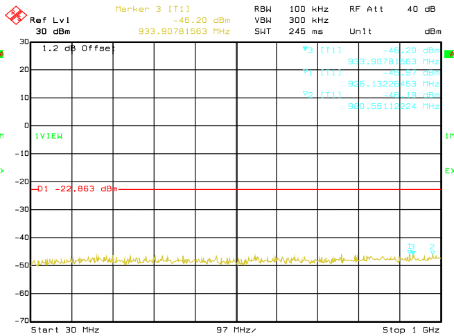
Date: 29.AUG.2019 02:44:46 Conducted Emissions. 802.11b, Frequency 2462 MHz Emission Level, 30 MHz -> 1 GHz
