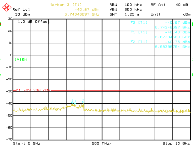
Date: 29.AUG.2019 03:02:04 Conducted Emissions. 802.11g, Frequency 2437 MHz Emission Level, 5 GHz -> 10 GHz
