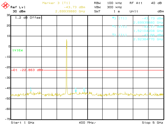
Date: 29.AUG.2019 02:45:40 Conducted Emissions. 802.11b, Frequency 2462 MHz Emission Level, 1 GHz -> 5 GHz
