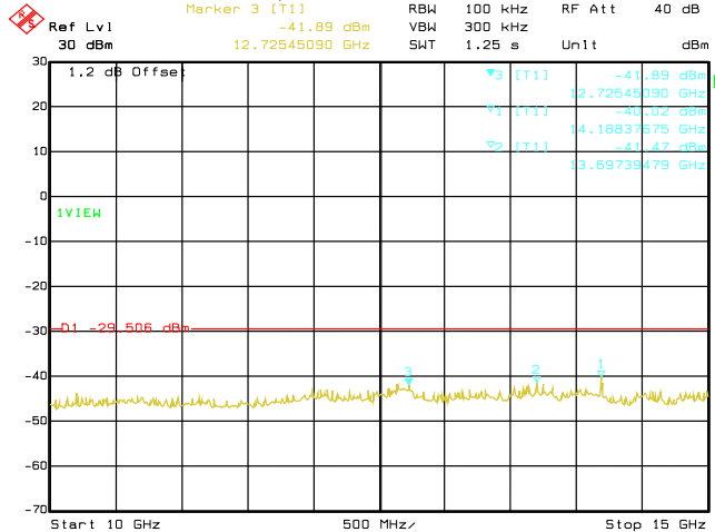
Date: 29.AUG.2019 03:14:33 Conducted Emissions. 802.11g, Frequency 2462 MHz Emission Level, 10 GHz -> 15 GHz
