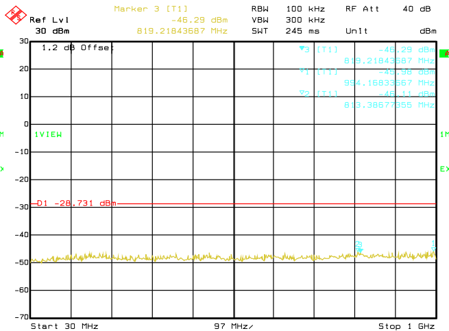
Date: 29.AUG.2019 02:52:45 Conducted Emissions. 802.11g, Frequency 2412 MHz Emission Level, 30 MHz -> 1 GHz
