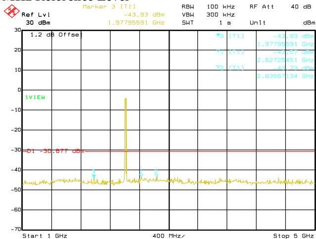
Date: 29.AUG.2019 03:23:20 Conducted Emissions. 802.11n, Frequency 2412 MHz Emission Level, 1 GHz -> 5 GHz
