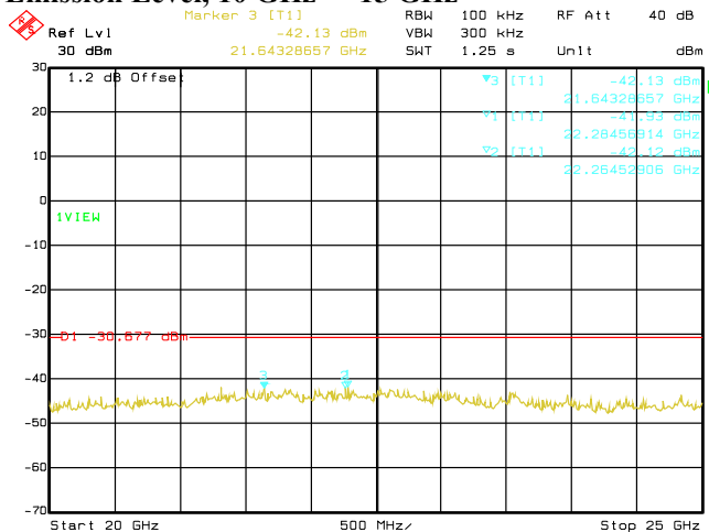
Date: 29.AUG.2019 03:26:54 Conducted Emissions. 802.11n, Frequency 2412 MHz Emission Level, 20 GHz -> 25 GHz
