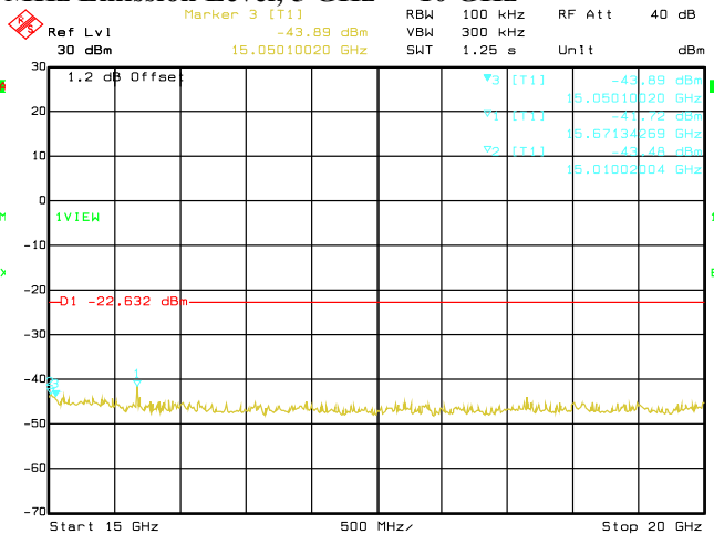
Date: 29.AUG.2019 02:34:05 Conducted Emissions. 802.11b, Frequency 2412 MHz Emission Level, 15 GHz -> 20 GHz
