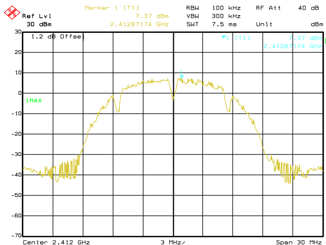
Date: 29.AUG.2019 02:29:37 Conducted Emissions. 802.11b, Frequency 2412 MHz Reference Level
