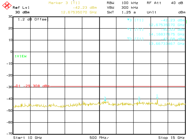
Date: 29.AUG.2019 03:02:57 Conducted Emissions. 802.11g, Frequency 2437 MHz Emission Level, 10 GHz -> 15 GHz
