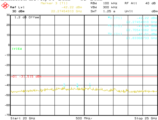
Date: 29.AUG.2019 03:38:58 Conducted Emissions. 802.11n, Frequency 2437 MHz Emission Level, 20 GHz -> 25 GHz
