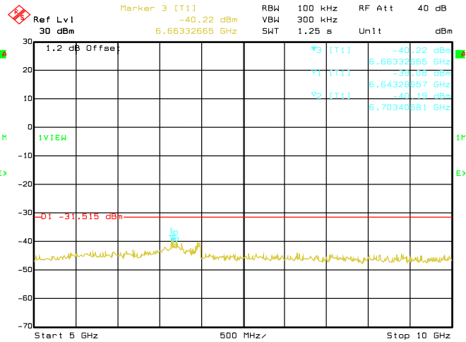
Date: 29.AUG.2019 03:36:18 Conducted Emissions. 802.11n, Frequency 2437 MHz Emission Level, 5 GHz -> 10 GHz
