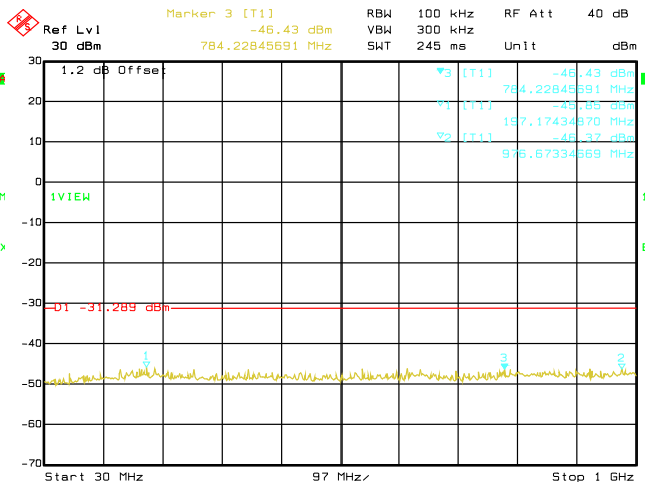
Date: 29.AUG.2019 03:42:13 Conducted Emissions. 802.11n, Frequency 2462 MHz Emission Level, 30 MHz -> 1 GHz
