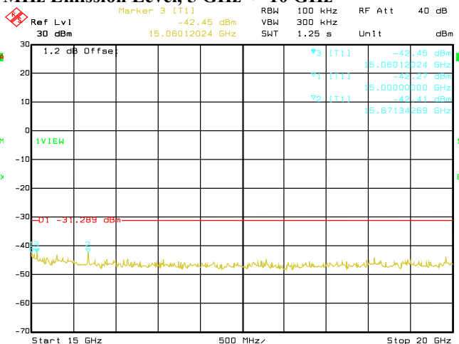
Date: 29.AUG.2019 03:45:46 Conducted Emissions. 802.11n, Frequency 2462 MHz Emission Level, 15 GHz -> 20 GHz
