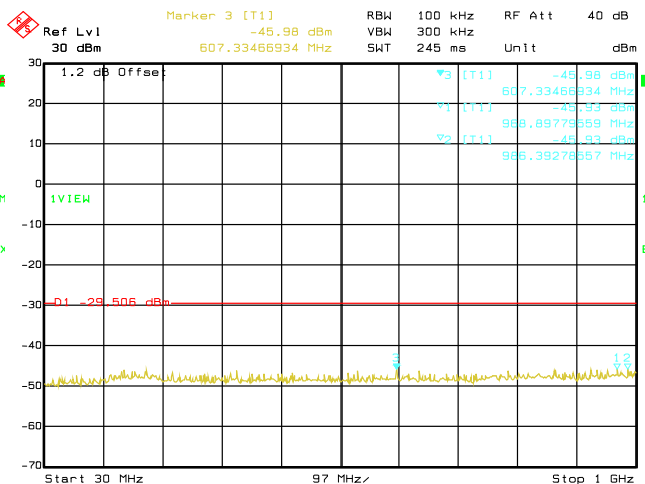
Date: 29.AUG.2019 03:11:53 Conducted Emissions. 802.11g, Frequency 2462 MHz Emission Level, 30 MHz -> 1 GHz
