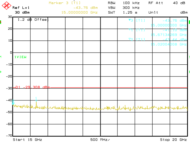
Date: 29.AUG.2019 03:03:51 Conducted Emissions. 802.11g, Frequency 2437 MHz Emission Level, 15 GHz -> 20 GHz
