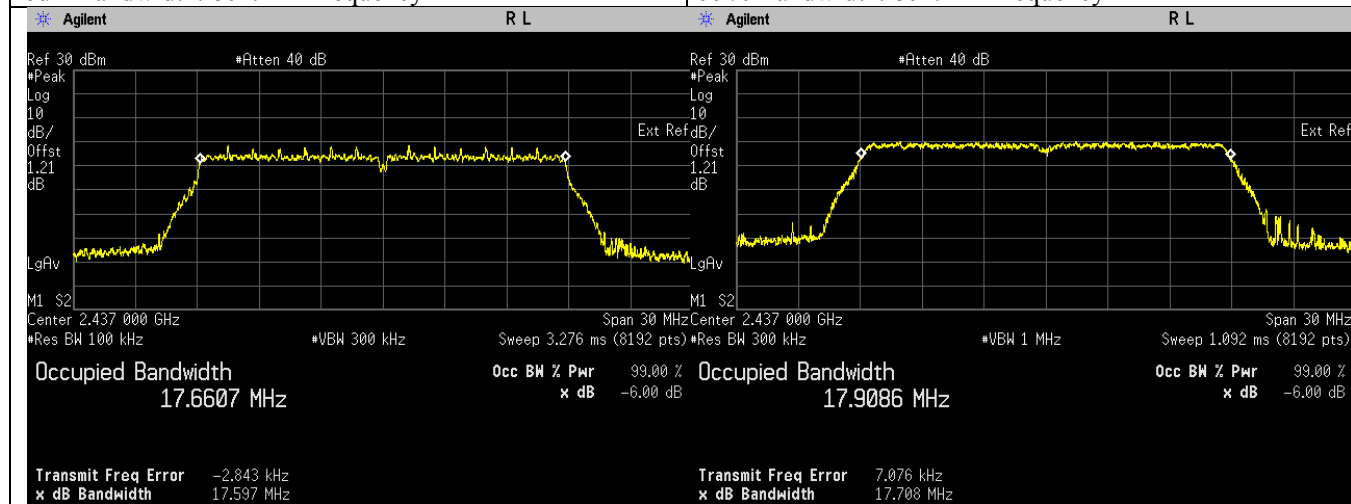
6dB Bandwidth. 802.11n Frequency 2437 MHz
