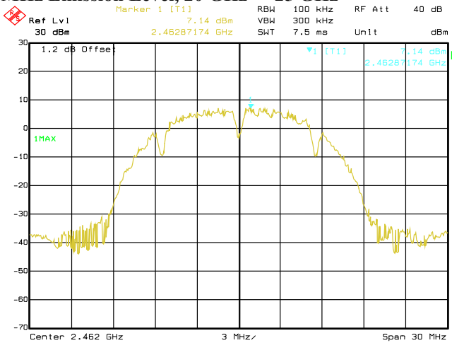
Date: 29.AUG.2019 02:43:53 Conducted Emissions. 802.11b, Frequency 2462 MHz Reference Level
