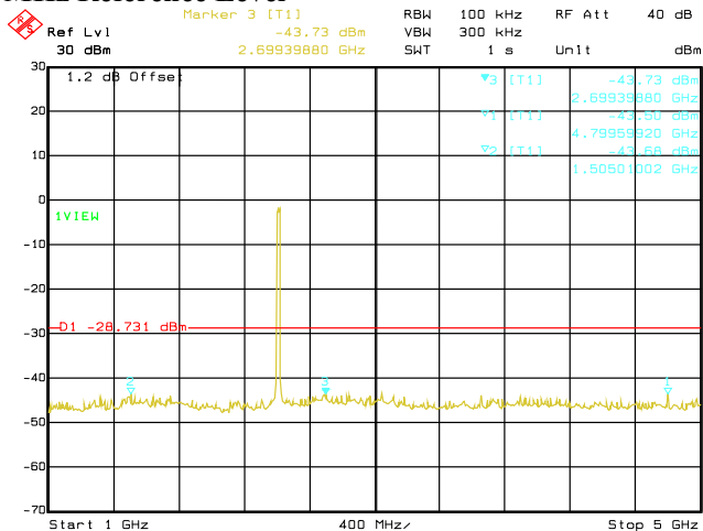
Date: 29.AUG.2019 02:53:39 Conducted Emissions. 802.11g, Frequency 2412 MHz Emission Level, 1 GHz -> 5 GHz
