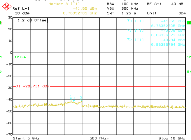
Date: 29.AUG.2019 02:54:32 Conducted Emissions. 802.11g, Frequency 2412 MHz Emission Level, 5 GHz -> 10 GHz
