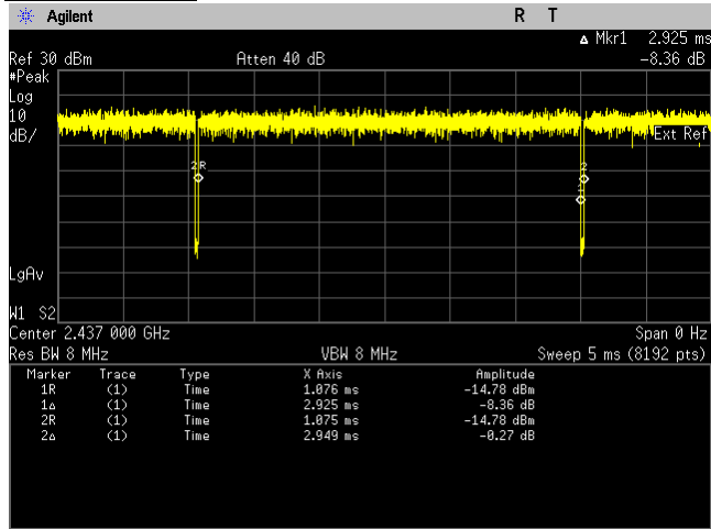
Duty Cycle, Antenna 1
