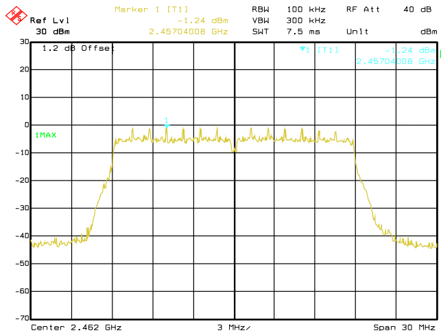
Date: 29.AUG.2019 03:41:19 Conducted Emissions. 802.11n, Frequency 2462 MHz Reference Level
