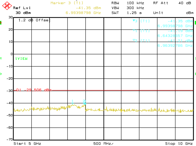
Date: 29.AUG.2019 03:13:40 Conducted Emissions. 802.11g, Frequency 2462 MHz Emission Level, 5 GHz -> 10 GHz
