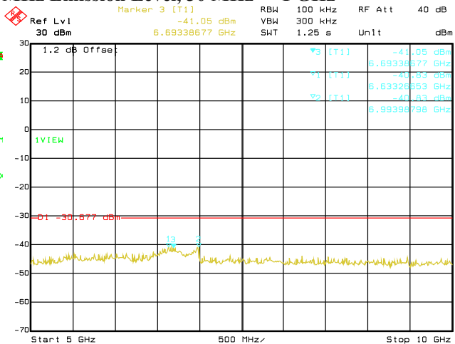
Date: 29.AUG.2019 03:24:13 Conducted Emissions. 802.11n, Frequency 2412 MHz Emission Level, 5 GHz -> 10 GHz
