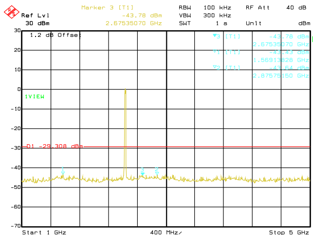
Date: 29.AUG.2019 03:01:11 Conducted Emissions. 802.11g, Frequency 2437 MHz Emission Level, 1 GHz -> 5 GHz
