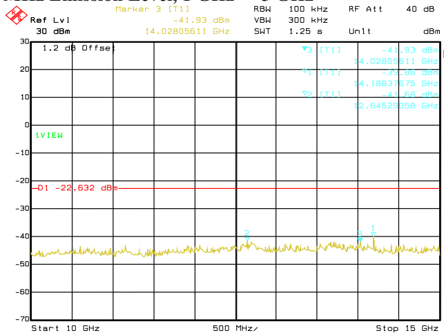
Date: 29.AUG.2019 02:33:12 Conducted Emissions. 802.11b, Frequency 2412 Emission Level, 10 GHz -> 15 GHz
