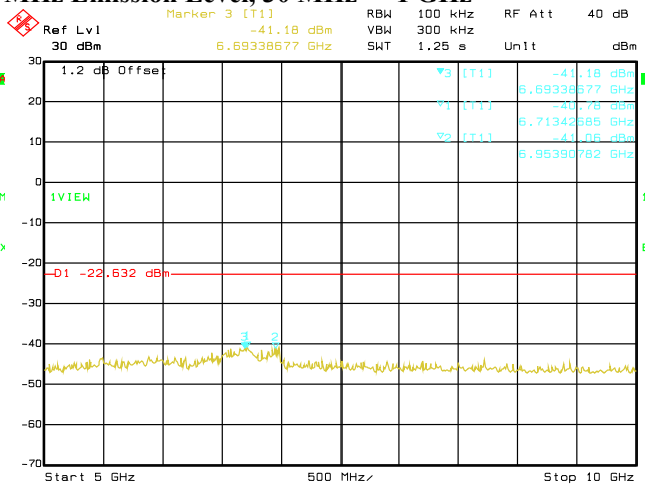
Date: 29.AUG.2019 02:32:19 Conducted Emissions. 802.11b, Frequency 2412 MHz Emission Level, 5 GHz -> 10 GHz
