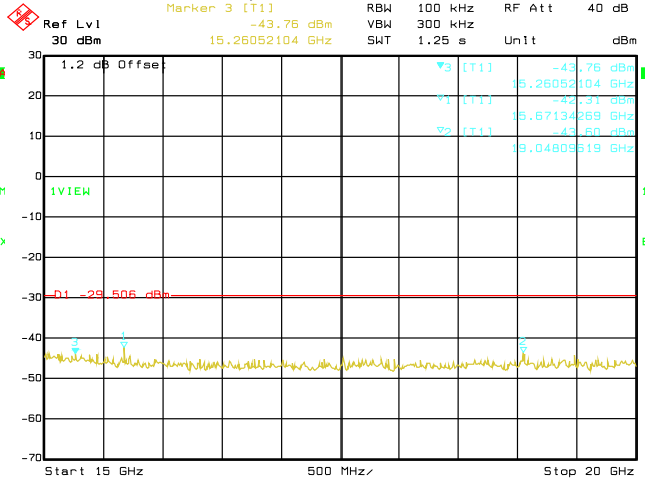
Date: 29.AUG.2019 03:15:26 Conducted Emissions. 802.11g, Frequency 2462 MHz Emission Level, 15 GHz -> 20 GHz
