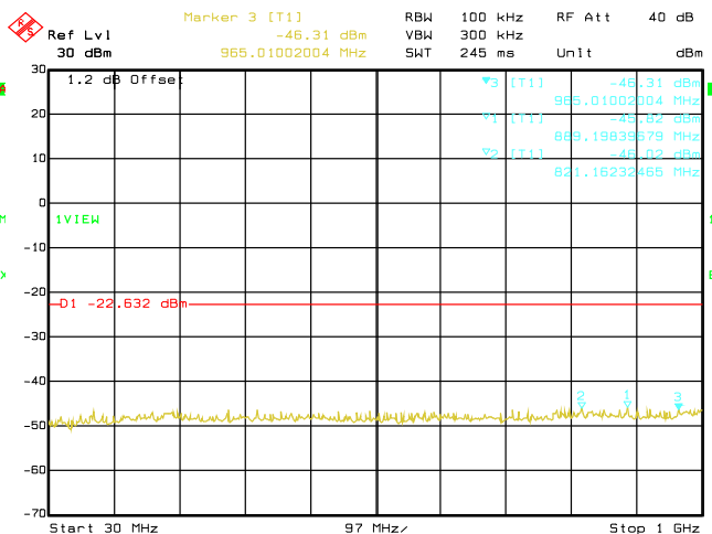
Date: 29.AUG.2019 02:30:31 Conducted Emissions. 802.11b, Frequency 2412 MHz Emission Level, 30 MHz -> 1 GHz
