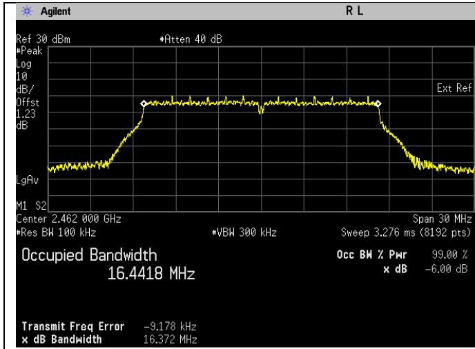
6dB Bandwidth. 802.11g Frequency 2462 MHz
