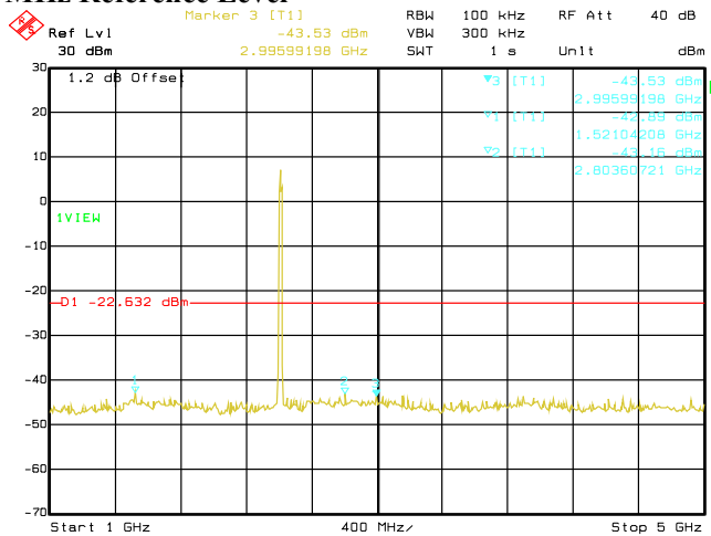
Date: 29.AUG.2019 02:31:25 Conducted Emissions. 802.11b, Frequency 2412 MHz Emission Level, 1 GHz -> 5 GHz
