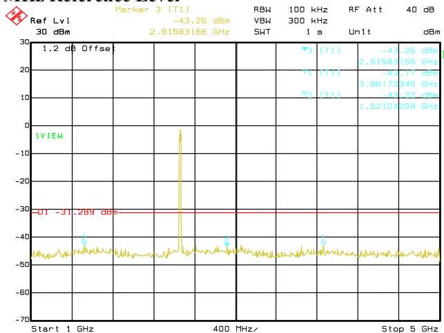
Date: 29.AUG.2019 03:43:07 Conducted Emissions. 802.11n, Frequency 2462 MHz Emission Level, 1 GHz -> 5 GHz
