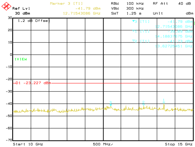
Date: 29.AUG.2019 02:40:06 Conducted Emissions. 802.11b, Frequency 2437 MHz Emission Level, 10 GHz -> 15 GHz
