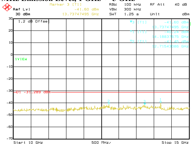
Date: 29.AUG.2019 03:44:53 Conducted Emissions. 802.11n, Frequency 2462 MHz Emission Level, 10 GHz -> 15 GHz
