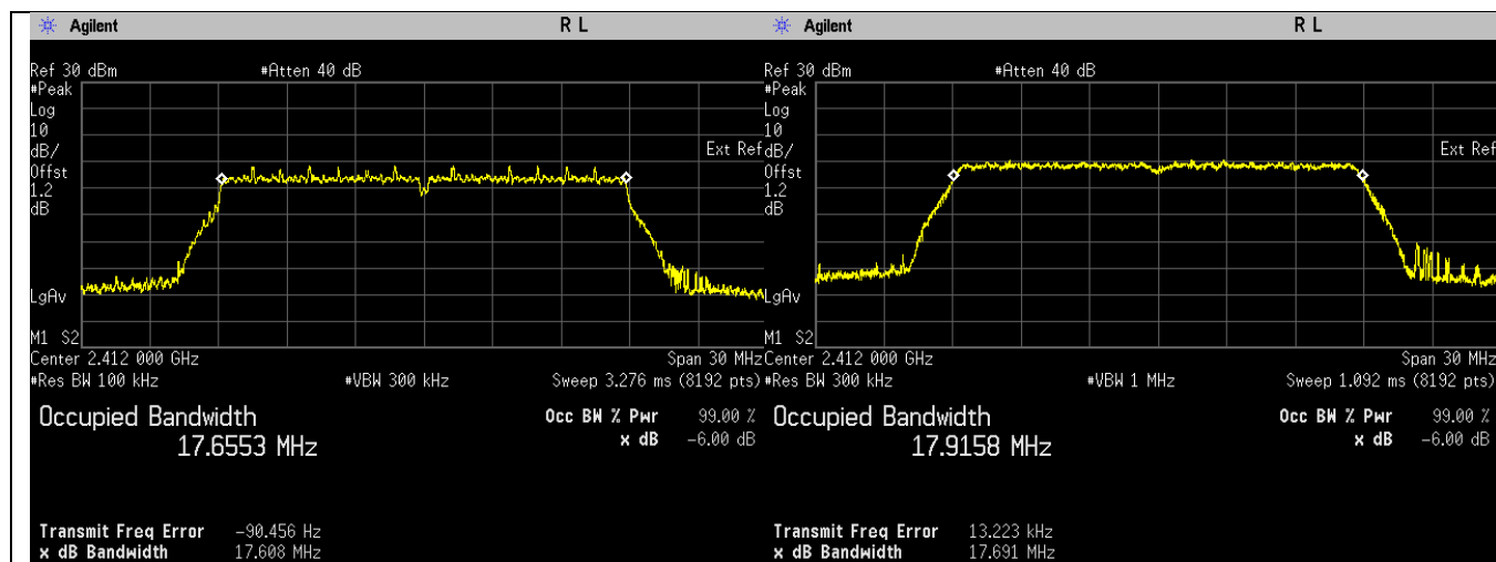
6dB Bandwidth. 802.11n Frequency 2412 MHz
