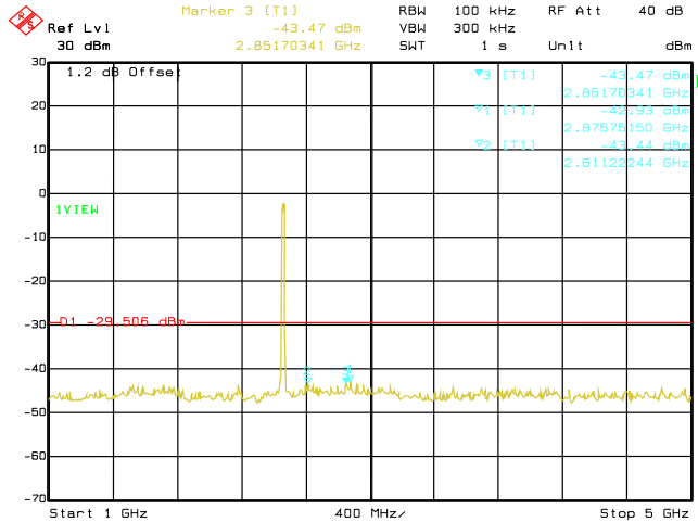
Date: 29.AUG.2019 03:12:47 Conducted Emissions. 802.11g, Frequency 2462 MHz Emission Level, 1 GHz -> 5 GHz
