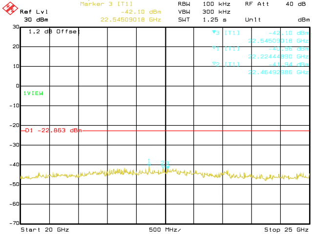
Date: 29.AUG.2019 02:49:14 Conducted Emissions. 802.11b, Frequency 2462 MHz Emission Level, 20 GHz -> 25 GHz
