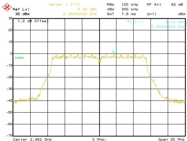
Date: 29.AUG.2019 03:10:59 Conducted Emissions. 802.11g, Frequency 2462 MHz Reference Level
