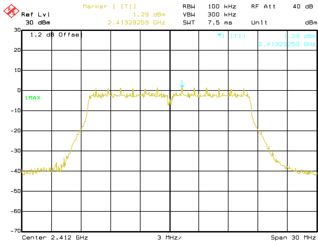
Date: 29.AUG.2019 02:51:51 Conducted Emissions. 802.11g, Frequency 2412 MHz Reference Level
