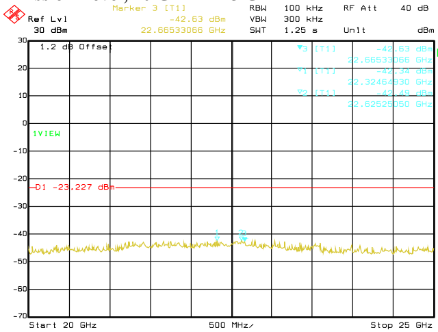
Date: 29.AUG.2019 02:41:52 Conducted Emissions. 802.11b, Frequency 2437 MHz Emission Level, 20 GHz -> 25 GHz
