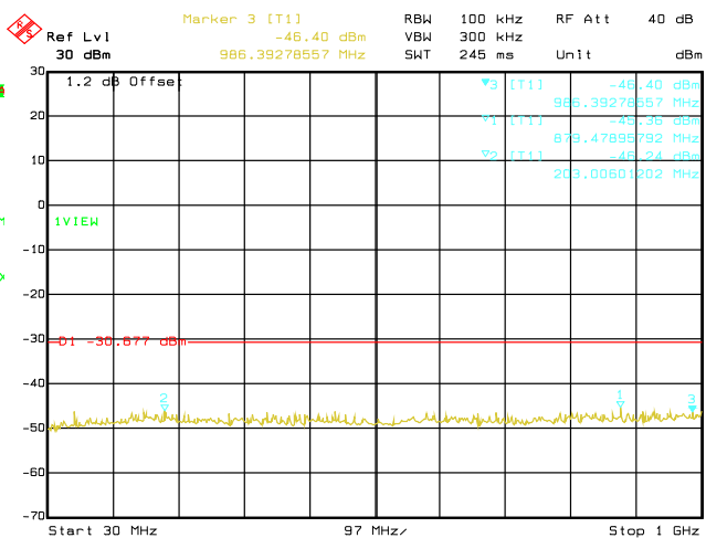
Date: 29.AUG.2019 03:22:26 Conducted Emissions. 802.11n, Frequency 2412 MHz Emission Level, 30 MHz -> 1 GHz
