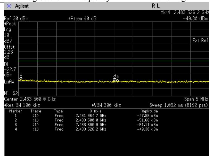
Band Edge. 802.11b Frequency 2462 MHz Band Edge
