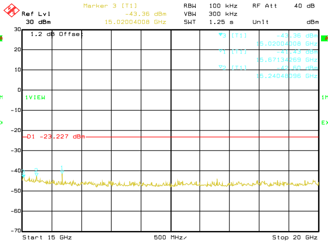
Date: 29.AUG.2019 02:40:59 Conducted Emissions. 802.11b, Frequency 2437 MHz Emission Level, 15 GHz -> 20 GHz
