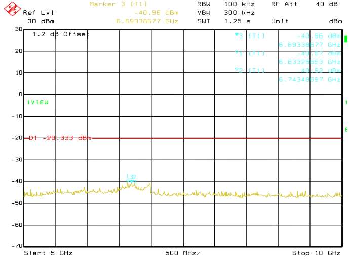
Date: 29.AUG.2019 04:06:14 Conducted Emissions. Bluetooth LE, Frequency 2402 MHz Emission Level, 5 GHz -> 10 GHz
