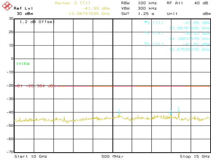
Date: 29.AUG.2019 04:22:27 Conducted Emissions. Bluetooth LE, Frequency 2480 MHz Emission Level, 10 GHz -> 15 GHz
