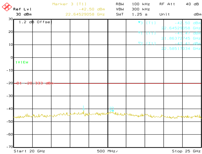
Date: 29.AUG.2019 04:08:55 Conducted Emissions. Bluetooth LE, Frequency 2402 MHz Emission Level, 20 GHz -> 25 GHz
