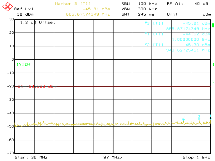
Date: 29.AUG.2019 04:04:27 Conducted Emissions. Bluetooth LE, Frequency 2402 MHz Emission Level, 30 MHz -> 1 GHz
