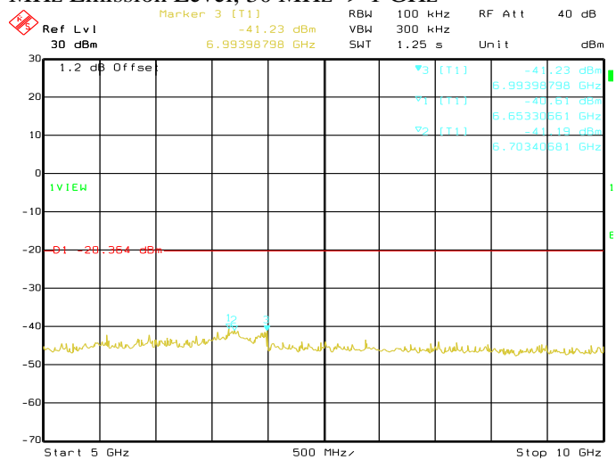
Date: 29.AUG.2019 04:13:50 Conducted Emissions. Bluetooth LE, Frequency 2440 MHz Emission Level, 5 GHz -> 10 GHz
