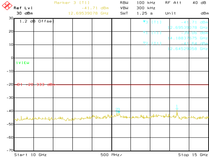
Date: 29.AUG.2019 04:07:08 Conducted Emissions. Bluetooth LE, Frequency 2402 MHz Emission Level, 10 GHz -> 15 GHz
