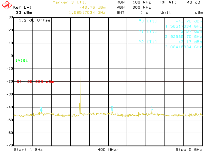
Date: 29.AUG.2019 04:05:21 Conducted Emissions. Bluetooth LE, Frequency 2402 MHz Emission Level, 1 GHz -> 5 GHz
