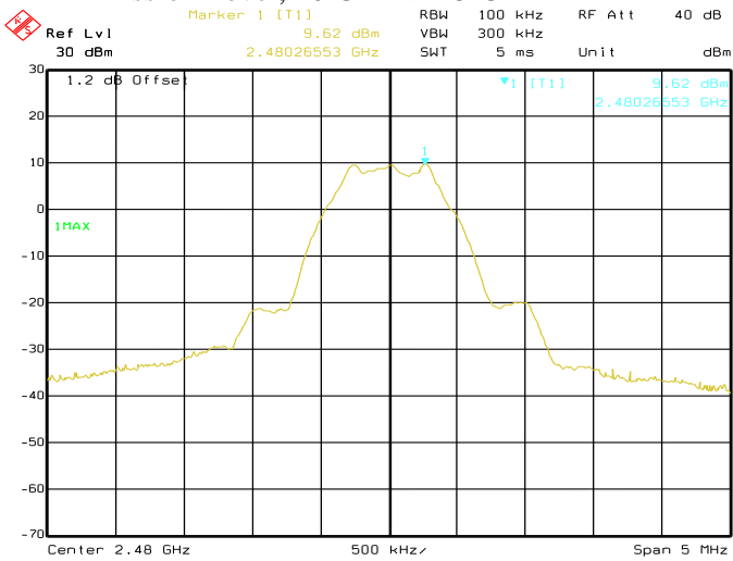
Date: 29.AUG.2019 04:18:41 Conducted Emissions. Bluetooth LE, Frequency 2480 MHz Reference Level
