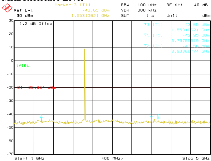
Date: 29.AUG.2019 04:12:57 Conducted Emissions. Bluetooth LE, Frequency 2440 MHz Emission Level, 1 GHz -> 5 GHz
