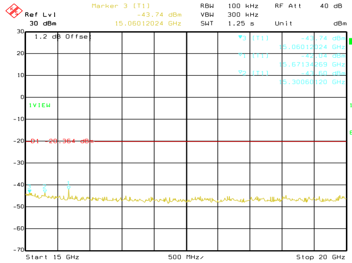
Date: 29.AUG.2019 04:15:36 Conducted Emissions. Bluetooth LE, Frequency 2440 MHz Emission Level, 15 GHz -> 20 GHz
