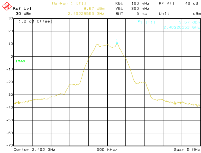
Date: 29.AUG.2019 04:03:32 Conducted Emissions. Bluetooth LE, Frequency 2402 MHz Reference Level
