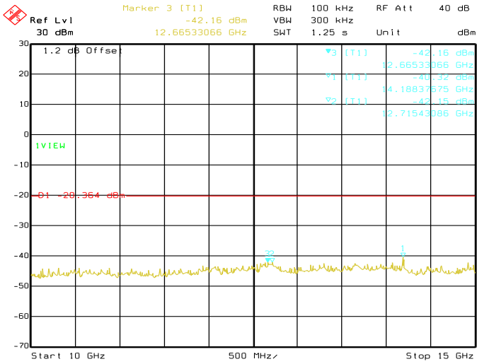
Date: 29.AUG.2019 04:14:43 Conducted Emissions. Bluetooth LE, Frequency 2440 MHz Emission Level, 10 GHz -> 15 GHz
