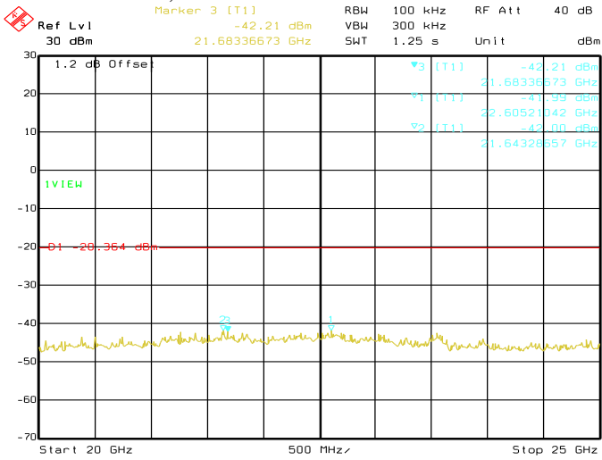
Date: 29.AUG.2019 04:16:30 Conducted Emissions. Bluetooth LE, Frequency 2440 MHz Emission Level, 20 GHz -> 25 GHz
