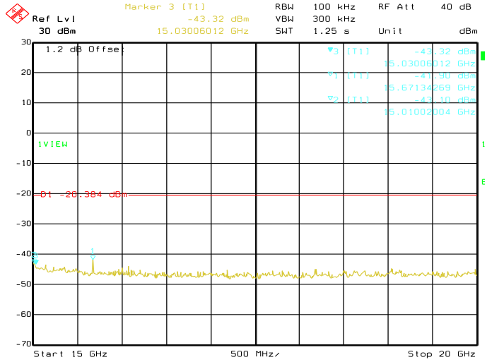
Date: 29.AUG.2019 04:23:20 Conducted Emissions. Bluetooth LE, Frequency 2480 MHz Emission Level, 15 GHz -> 20 GHz
