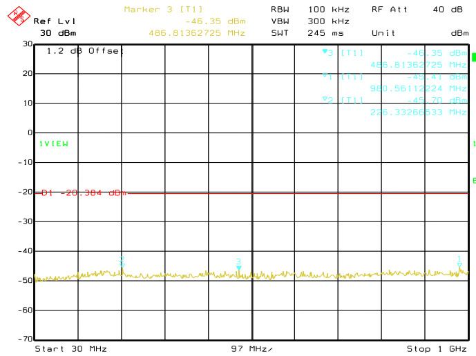
Date: 29.AUG.2019 04:19:35 Conducted Emissions. Bluetooth LE, Frequency 2480 MHz Emission Level, 30 MHz -> 1 GHz
