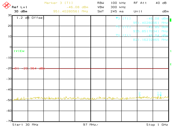
Date: 29.AUG.2019 04:12:03 Conducted Emissions. Bluetooth LE, Frequency 2440 MHz Emission Level, 30 MHz -> 1 GHz
