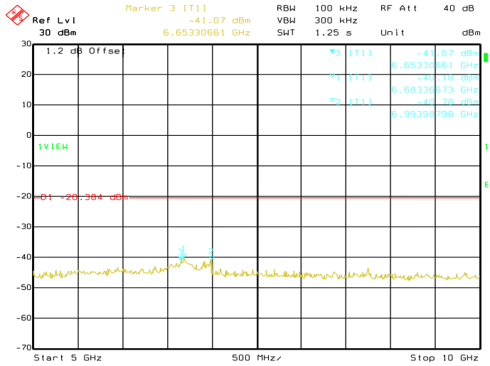
Date: 29.AUG.2019 04:21:34 Conducted Emissions. Bluetooth LE, Frequency 2480 MHz Emission Level, 5 GHz -> 10 GHz
