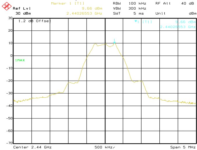
Date: 29.AUG.2019 04:11:09 Conducted Emissions. Bluetooth LE, Frequency 2440 MHz Reference Level
