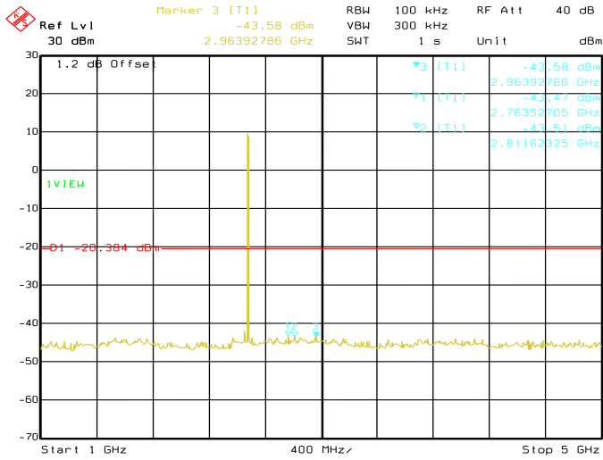
Date: 29.AUG.2019 04:20:40 Conducted Emissions. Bluetooth LE, Frequency 2480 MHz Emission Level, 1 GHz -> 5 GHz
