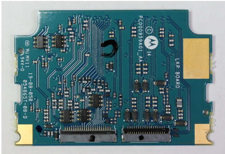
Limited Keypad board (Bottom)
