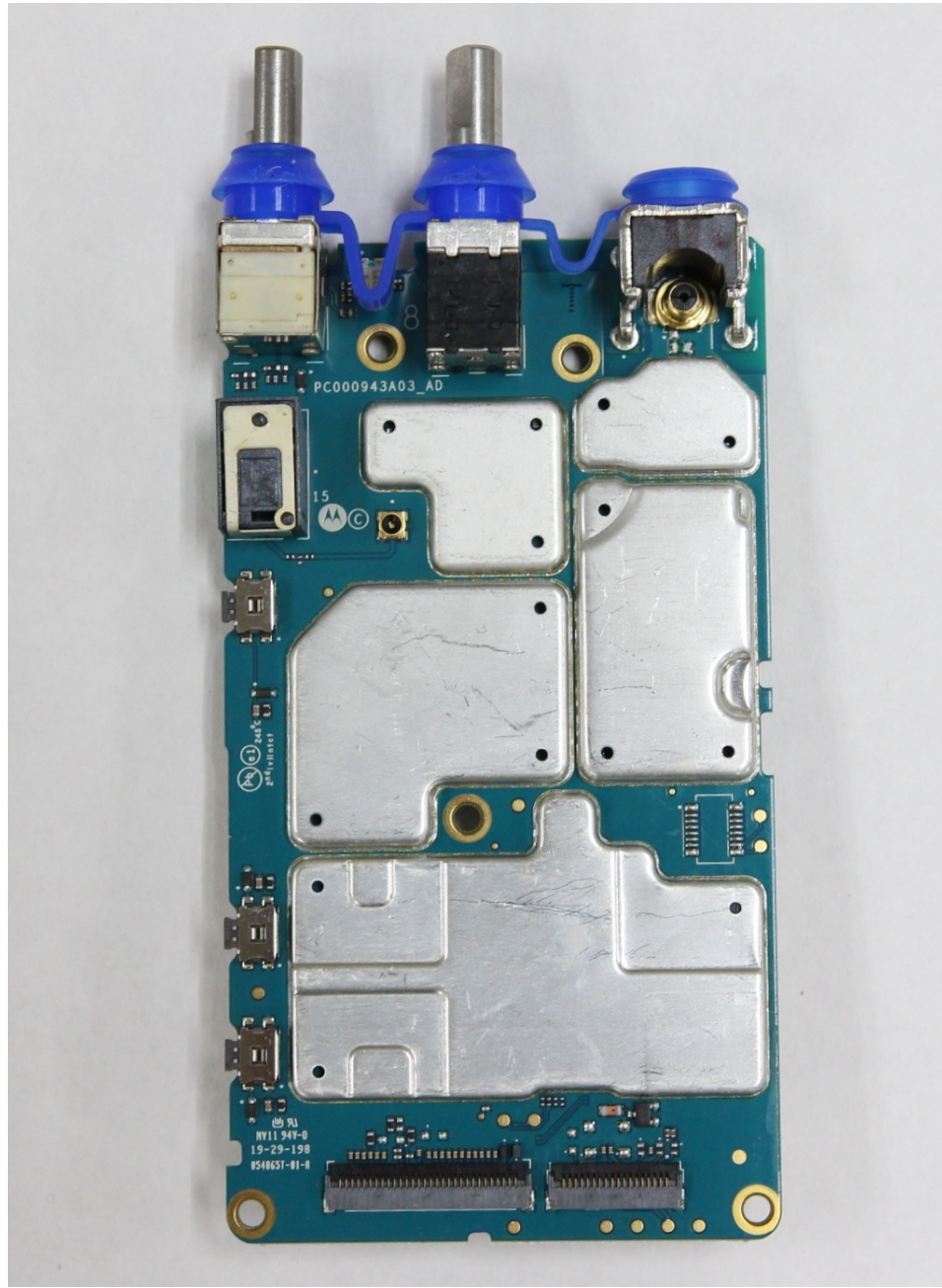
RF board with Shields (Top)
