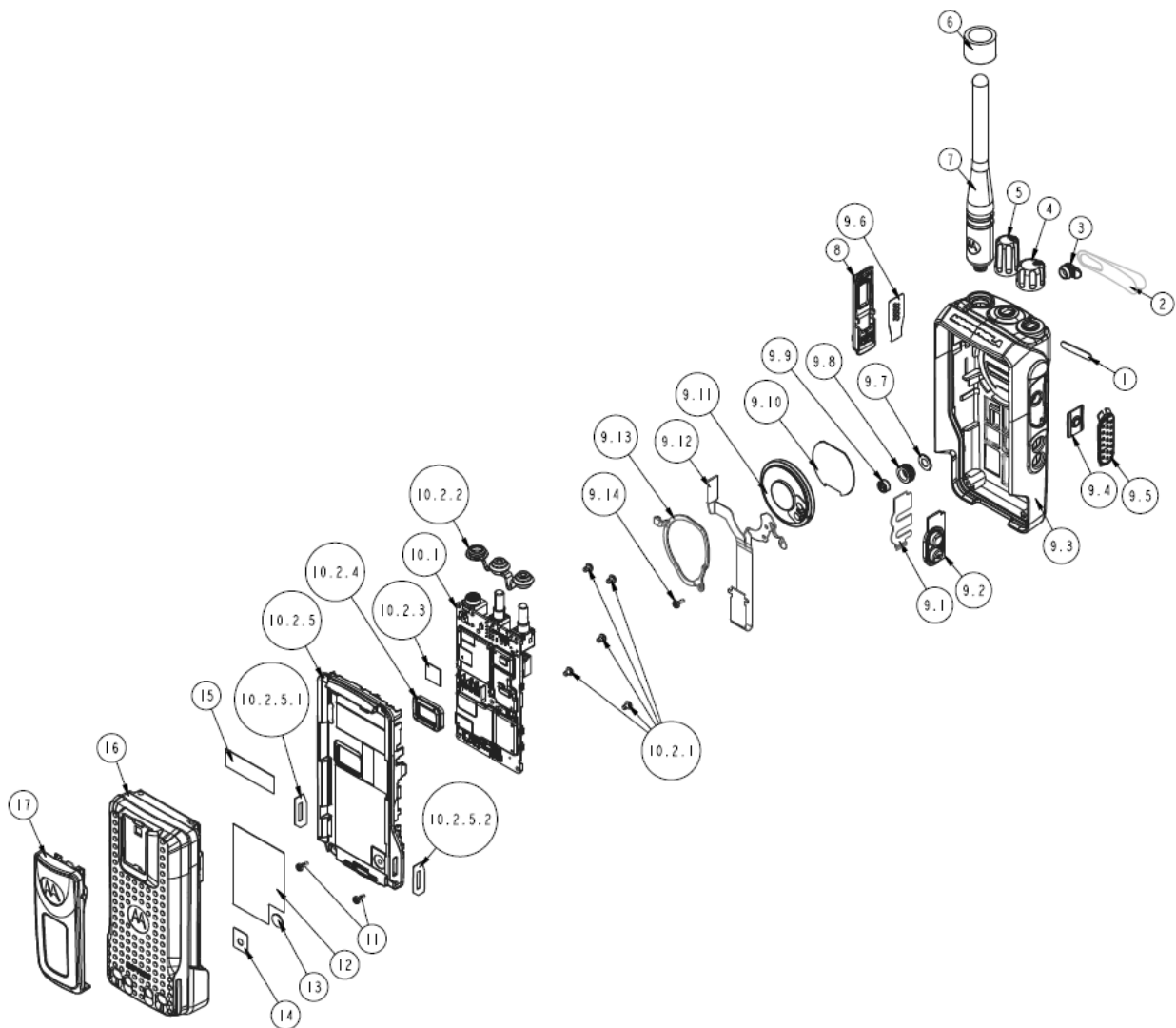
Exploded view of NKP radio
