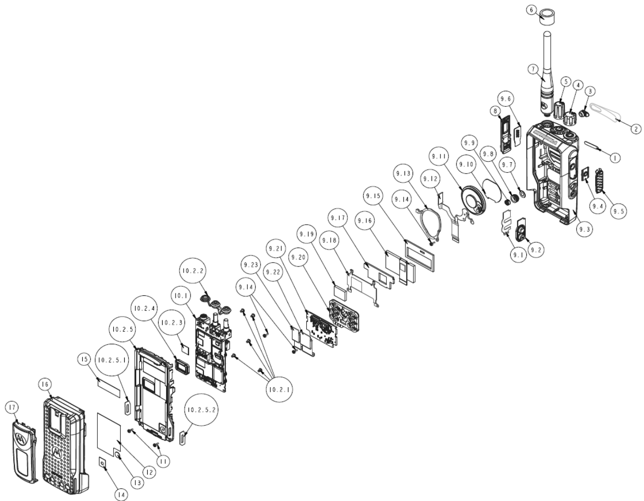
Exploded view of LKP radio
