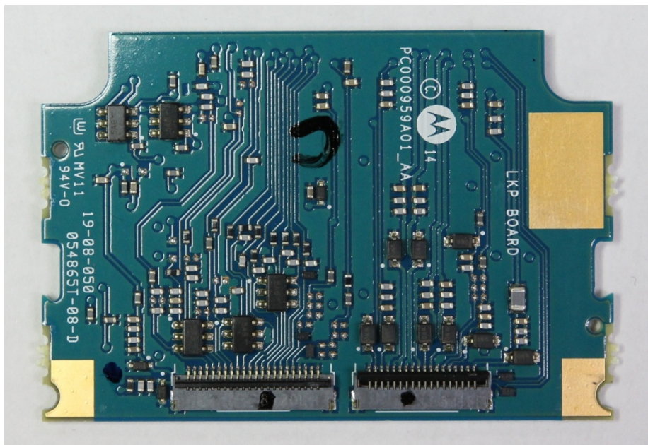
Limited Keypad Board (Bottom)
