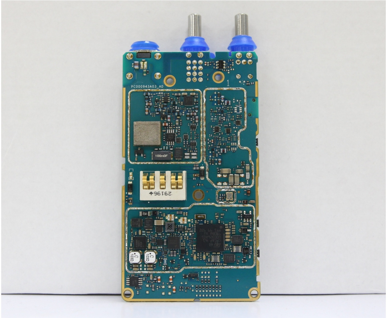
RF board without Shields (Bottom)
