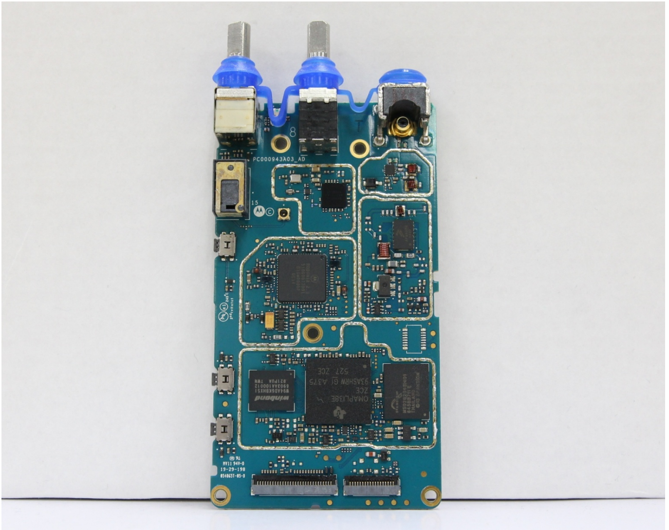
RF board without Shields (Top)
