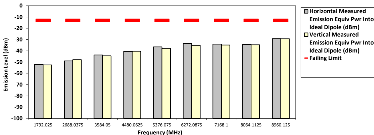
RADIATED SPURIOUS EMISSIONS
