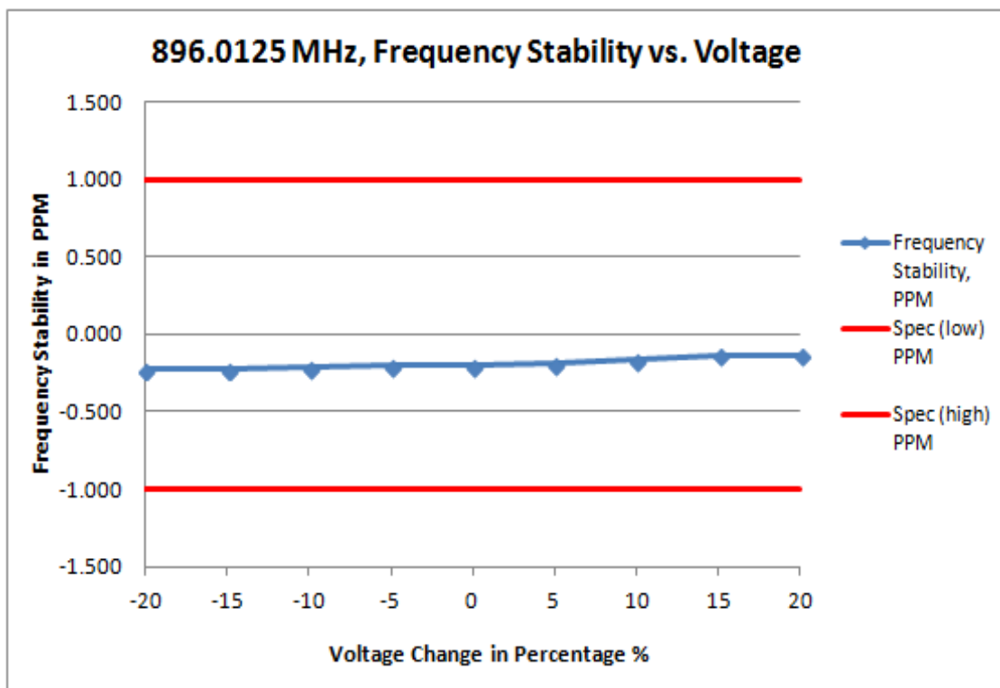
(i) Frequency Stability VS Voltage
