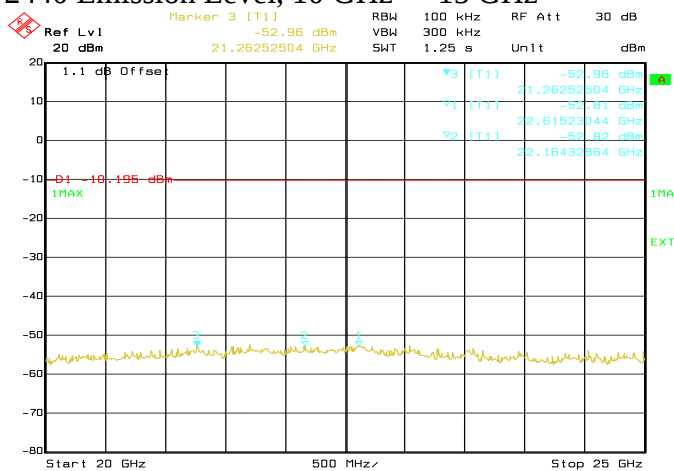
Conducted Emissions. Bluetooth LE, Frequency 2440 MHz Emission Level, 20 GHz -> 25 GHz
