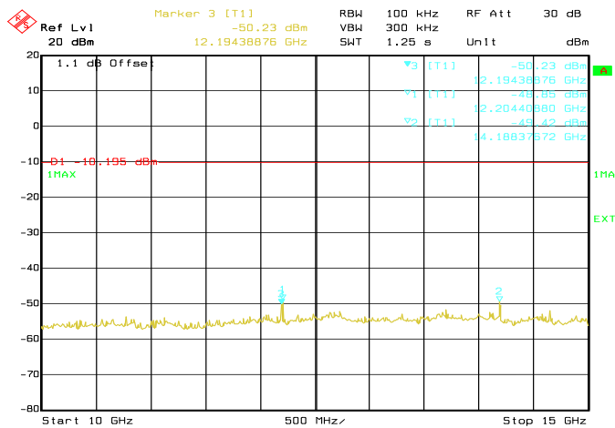
Conducted Emissions. Bluetooth LE, Frequency 2440 Emission Level, 10 GHz -> 15 GHz
