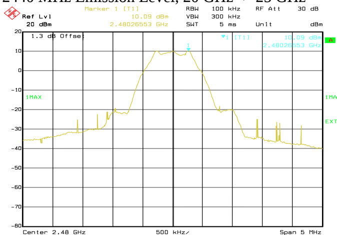
Conducted Emissions. Bluetooth LE, Frequency 2480 MHz Reference Level
