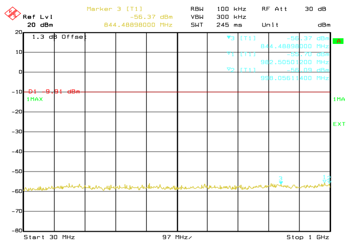
Conducted Emissions. Bluetooth LE, Frequency 2480 MHz Emission Level, 30 MHz -> 1 GHz
