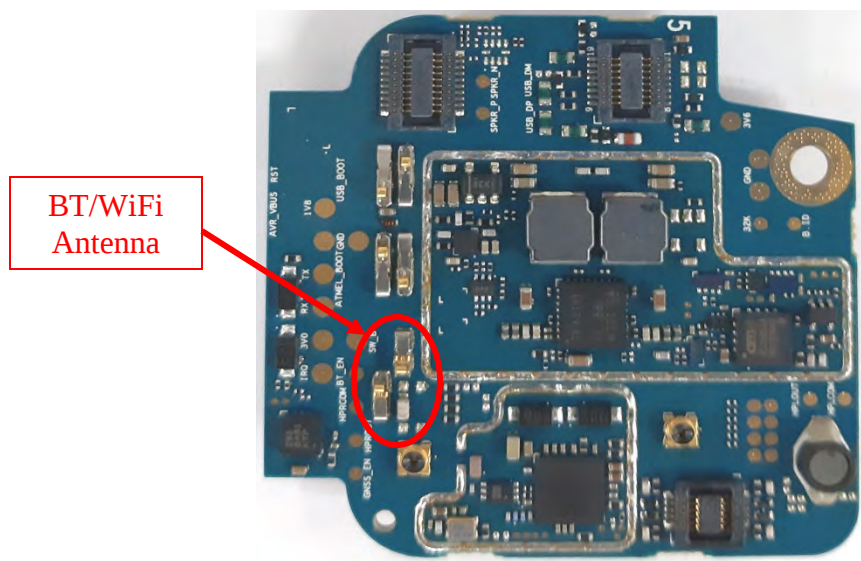
Expansion board without shields (Top) (APX6000/APX5000/APX6000XE/APX6000Li/SRX2200)
