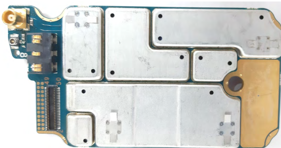
RF board with Shields (Bottom) (APX6000/APX5000/APX6000XE/APX6000Li/SRX2200)
