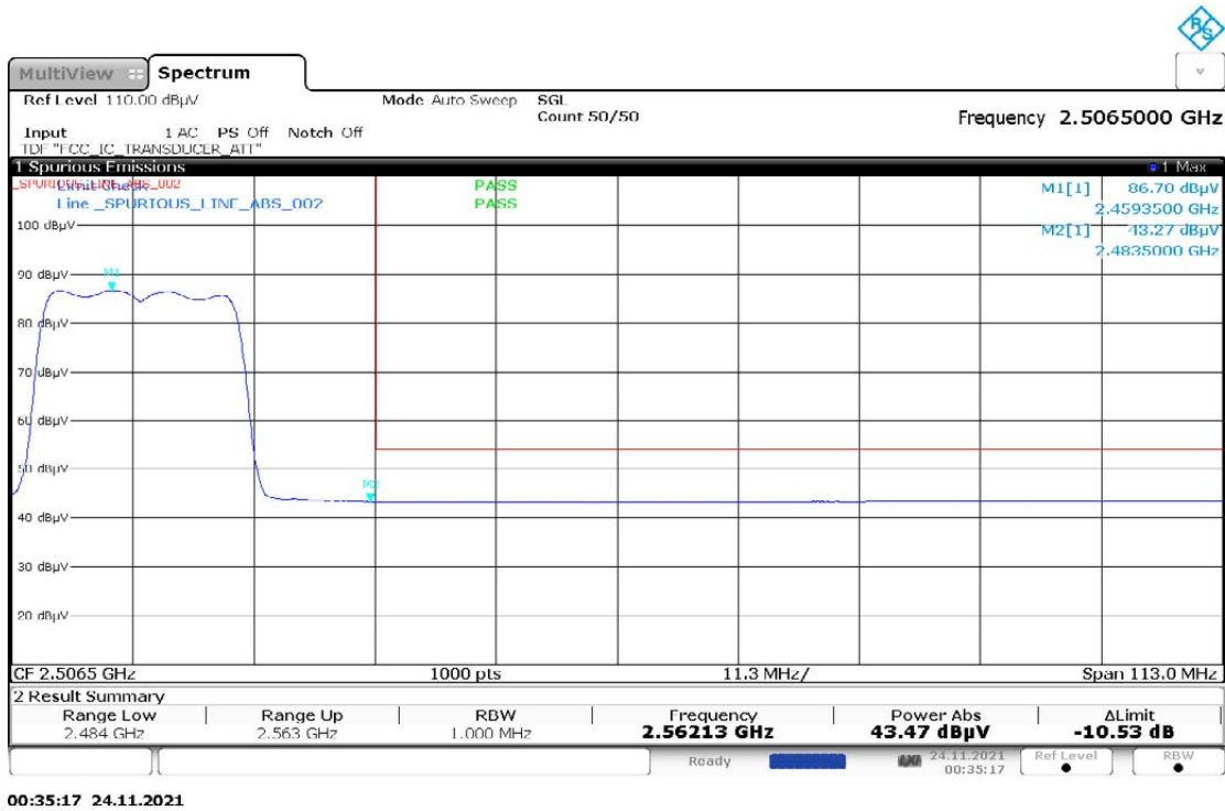
Restricted Band Edge (High Channel, Horizontal, Average) graphical screen shot
