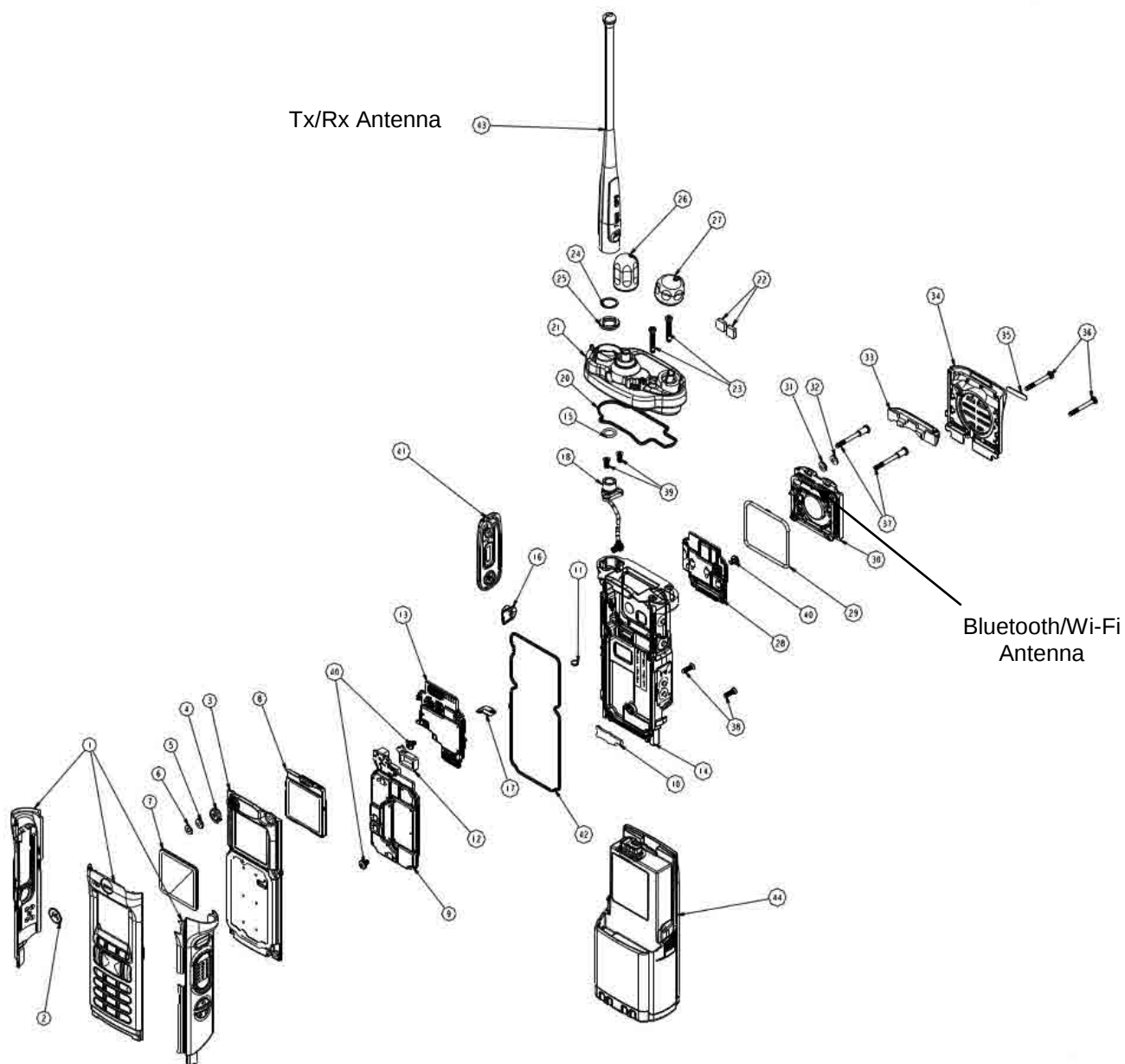
Exploded view of APX6000XE Model 3.5 radio
