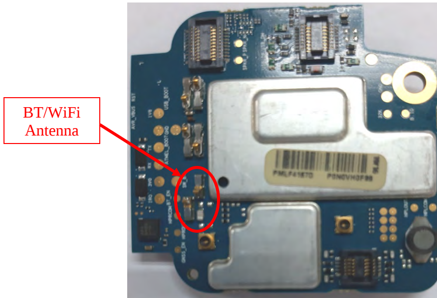
Expansion board with shields (Top) (APX6000/APX5000/APX6000XE/APX6000Li/SRX2200)
