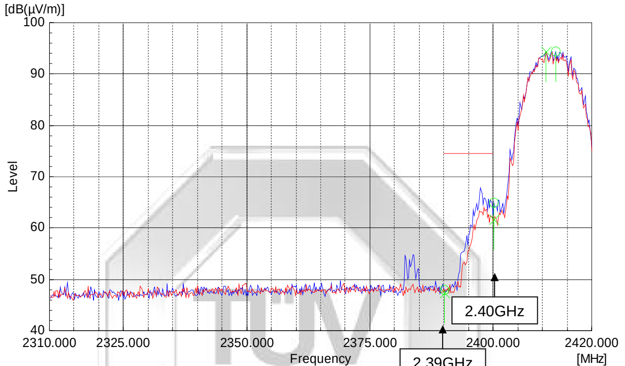
Plot 485 – Lower Band Edge at 2.4000GHz @ CCK 11Mbps
