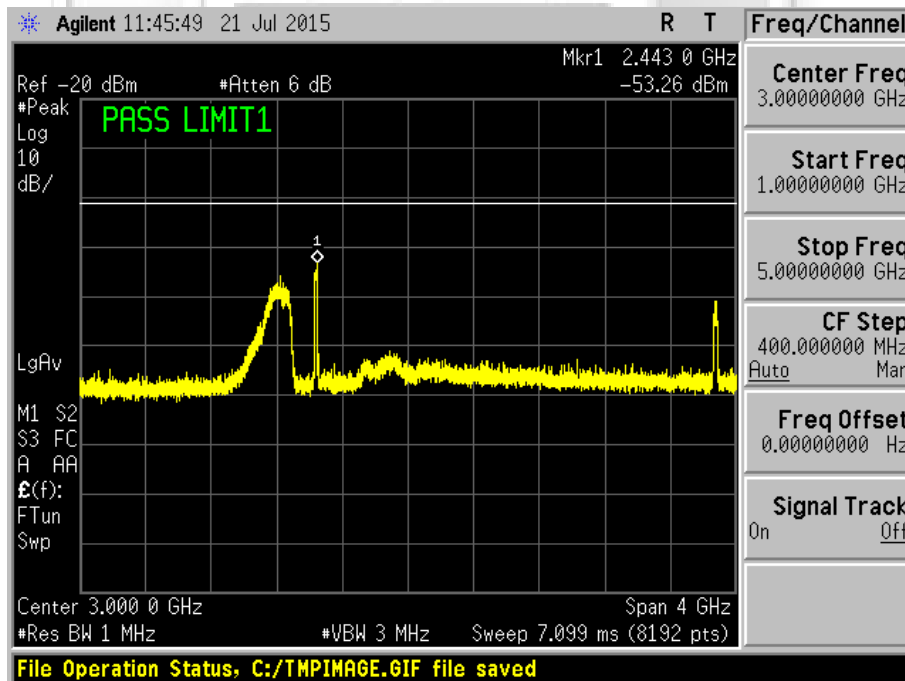
Plot 286 – Channel 6 (middle ch) @ 16QAM 36Mbps
