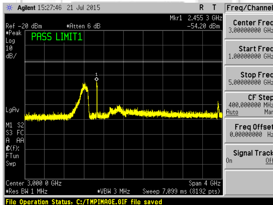
Plot 456 – Channel 11 (upper ch) @ 64QAM 65Mbps
