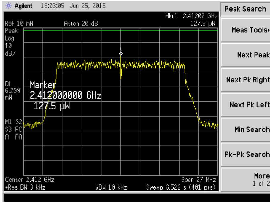
Plot 512 – Channel 1 (lower ch) @ 16QAM 39Mbps
