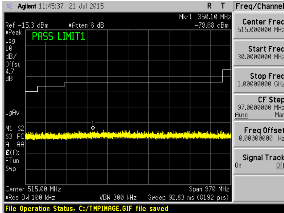
Plot 285 – Channel 6 (middle ch) @ 16QAM 36Mbps
