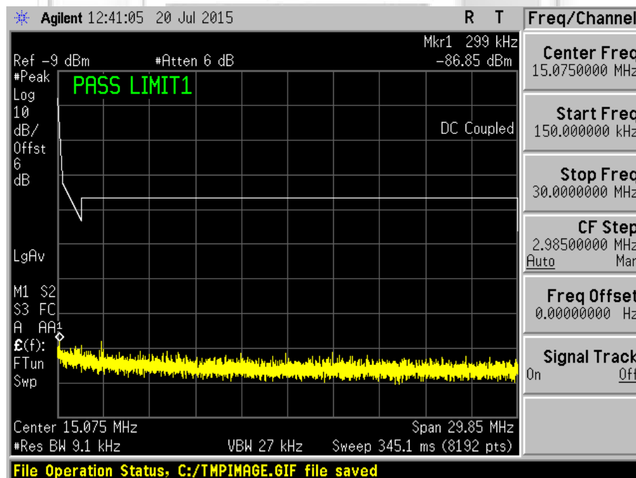
Plot 164 – Channel 6 (middle ch) @ DBPSK 1Mbps
