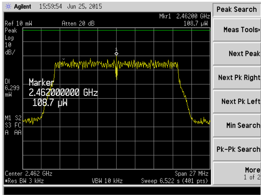
Plot 534 – Channel 11 (upper ch) @ 16QAM 39Mbps
