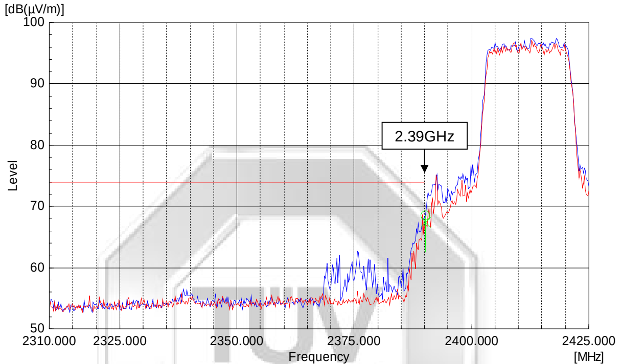
Plot 499 – Peak Plot at Lower Band Edge at 2.4000GHz @ 64QAM 65Mbps
