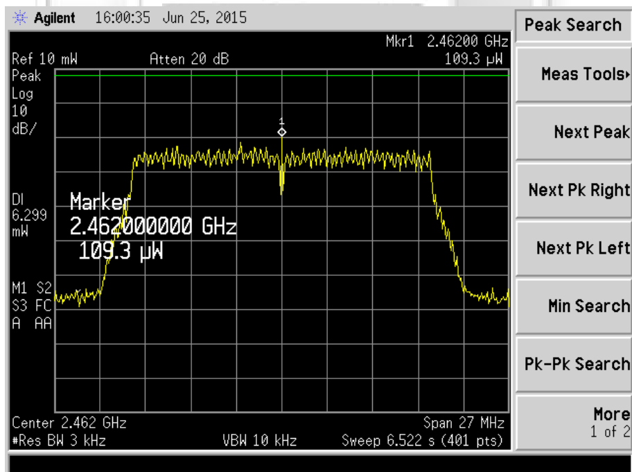
Plot 535 Channel 11 (upper ch) @ 64QAM 65Mbps
