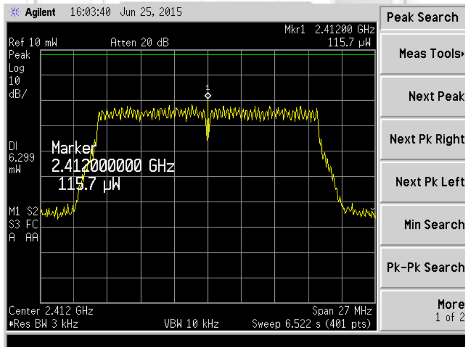
Plot 513 – Channel 1 (lower ch) @ 64QAM 65Mbps
