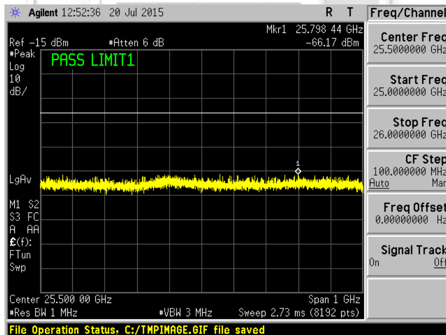
Plot 202 – Channel 11 (upper ch) @ DBPSK 1Mbps
