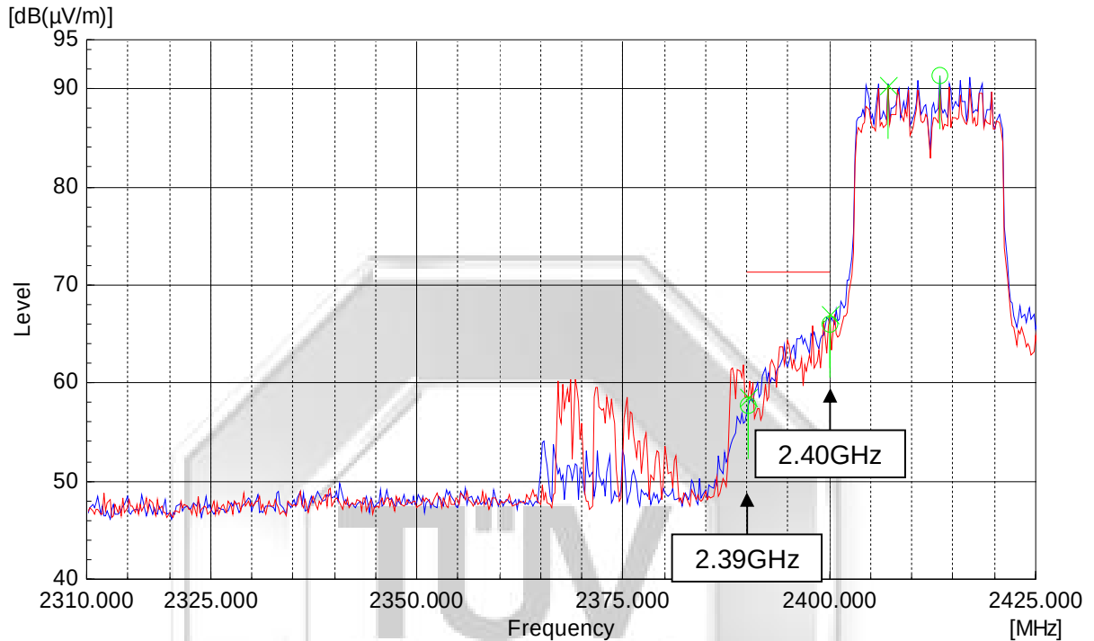
Plot 497 – Lower Band Edge at 2.4000GHz @ 64QAM 65Mbps
