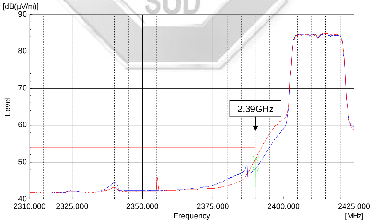
Plot 500 – Average Plot at Lower Band Edge at 2.4000GHz @ 64QAM 65Mbps
