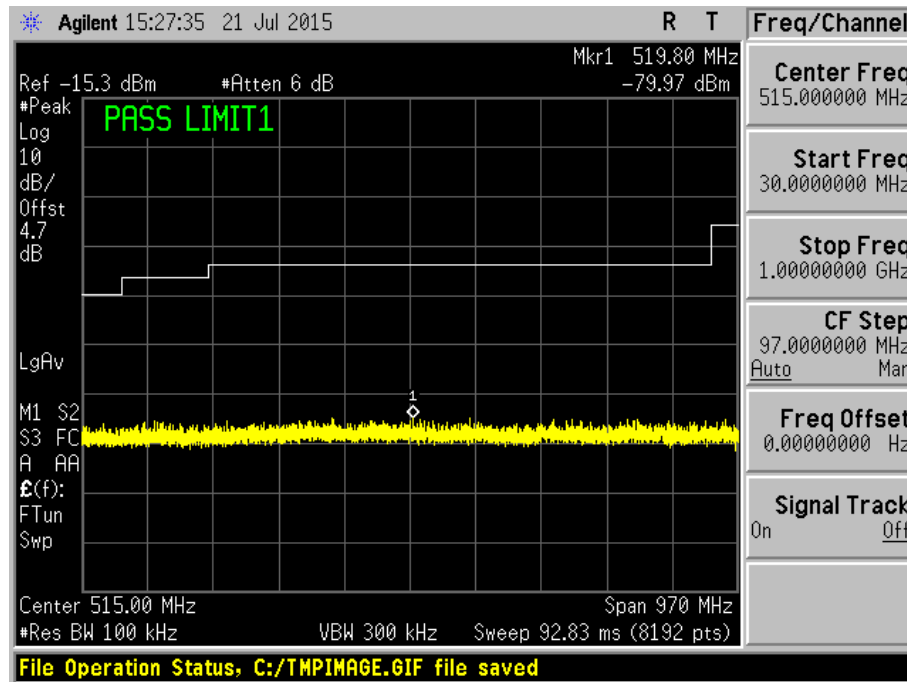
Plot 455 – Channel 11 (upper ch) @ 64QAM 65Mbps
