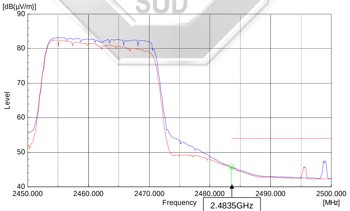
Plot 502 – Average Plot at Upper Band Edge at 2.4835GHz @ 64QAM 65Mbps
