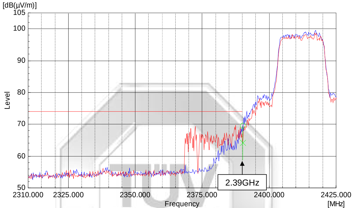
Plot 493 – Peak Plot at Lower Band Edge at 2.4000GHz @ 64QAM 54Mbps
