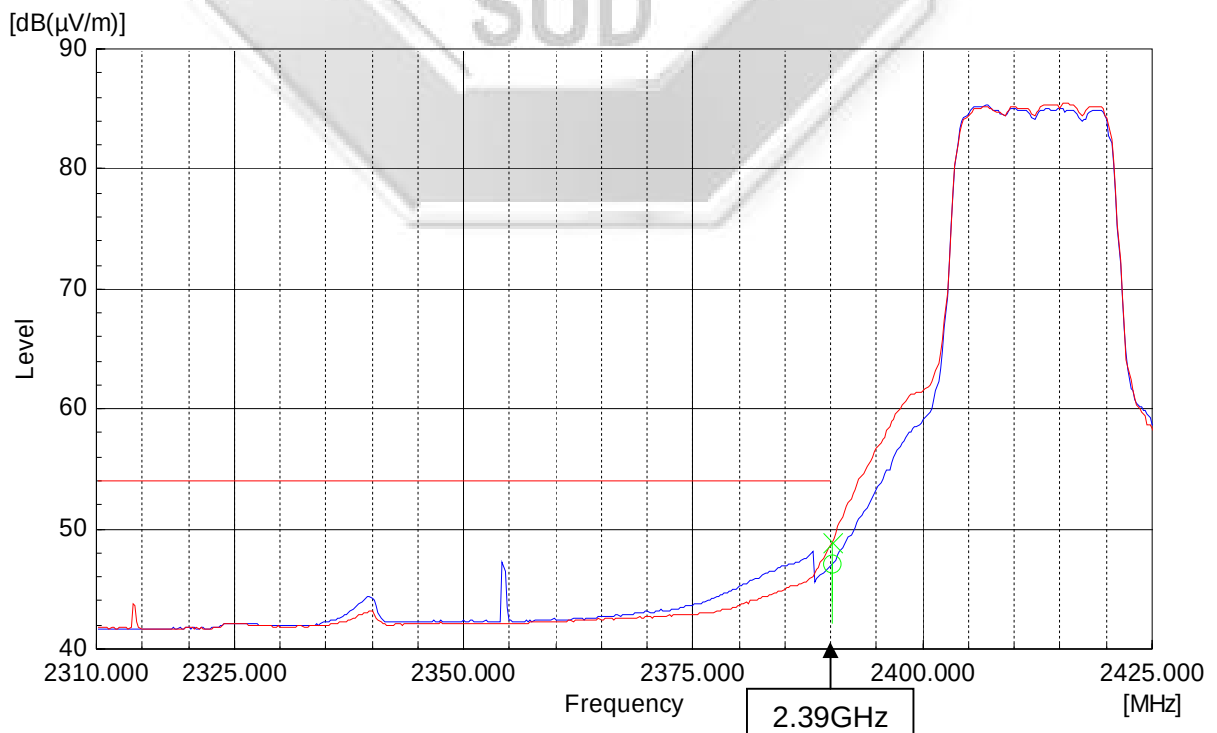
Plot 494 – Average Plot at Lower Band Edge at 2.4000GHz @ 64QAM 54Mbps
