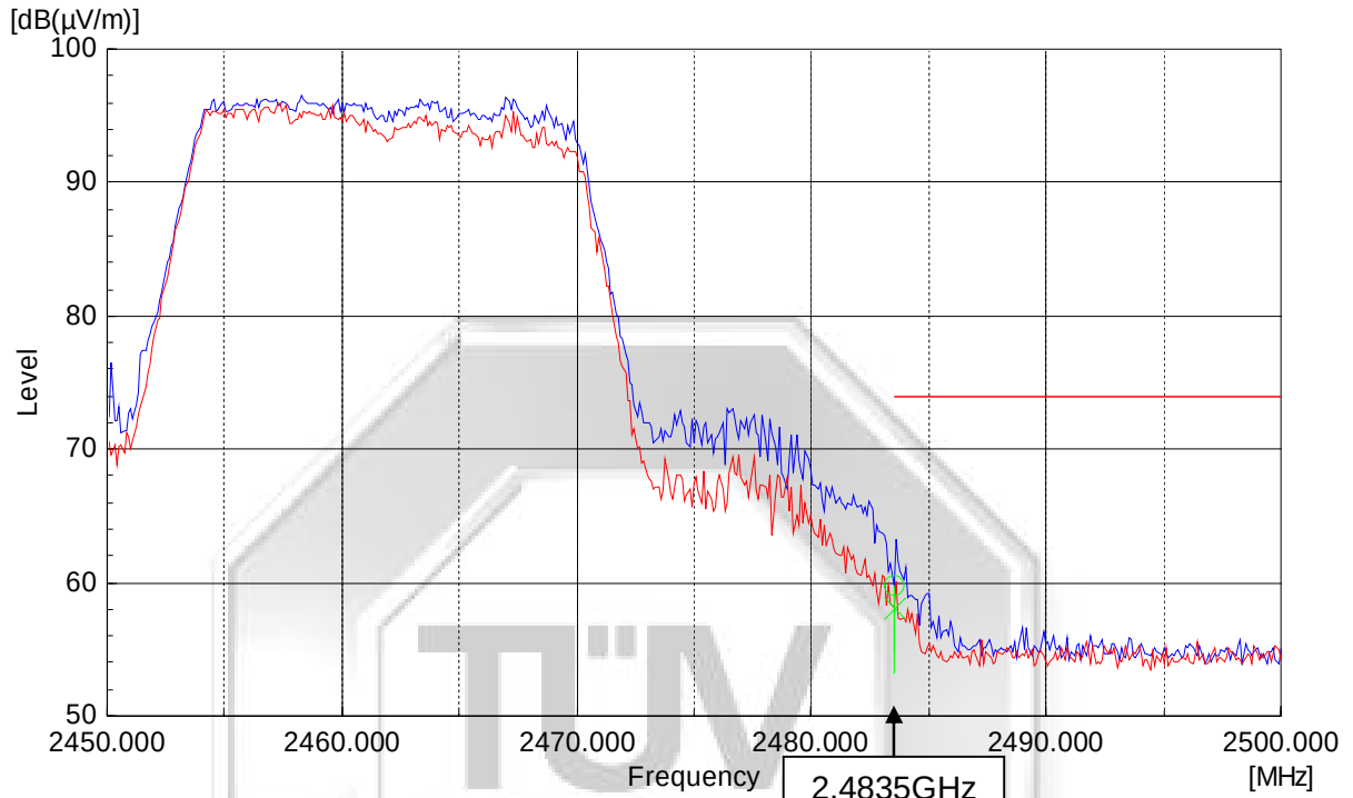
Plot 495 – Peak Plot at Upper Band Edge at 2.4835GHz @ 64QAM 54Mbps
