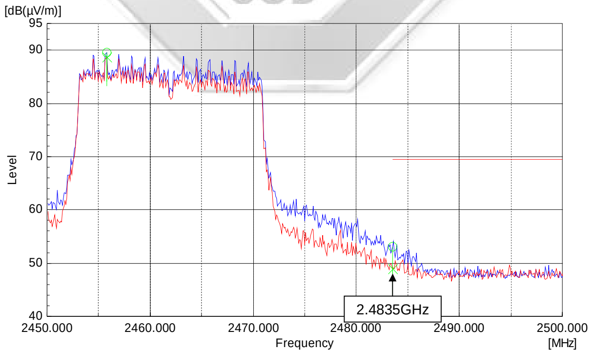
Plot 498 – Upper Band Edge at 2.4835GHz @ 64QAM 65Mbps
