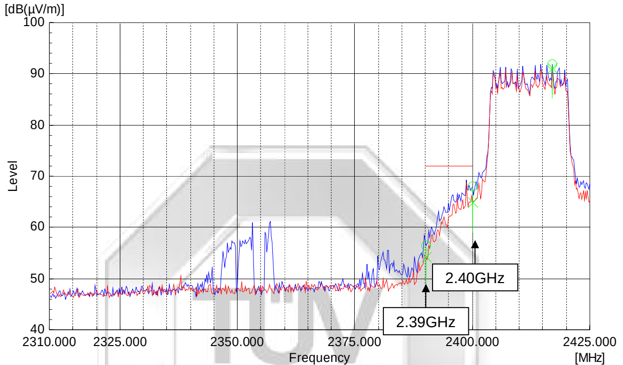
Plot 491 – Lower Band Edge at 2.4000GHz @ 64QAM 54Mbps
