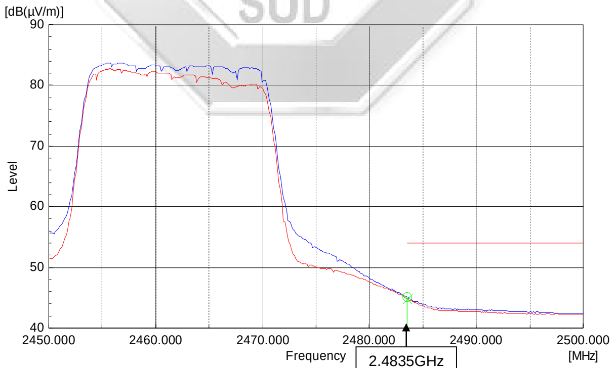
Plot 496 – Average Plot at Upper Band Edge at 2.4835GHz @ 64QAM 54Mbps
