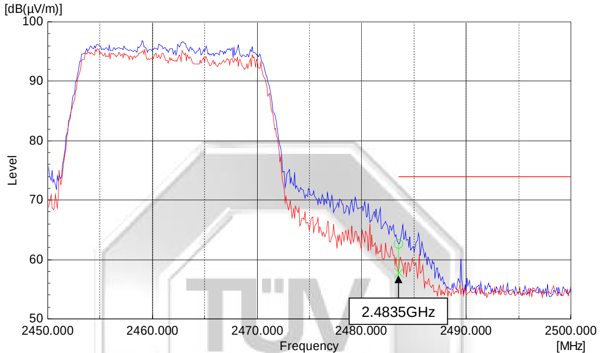
Plot 501 – Peak Plot at Upper Band Edge at 2.4835GHz @ 64QAM 65Mbps
