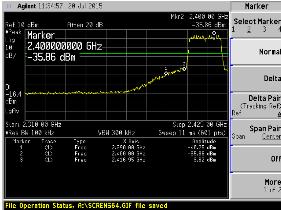
Plot 477 – Lower Band Edge at 2.4000GHz @ BPSK 6.5Mbps
