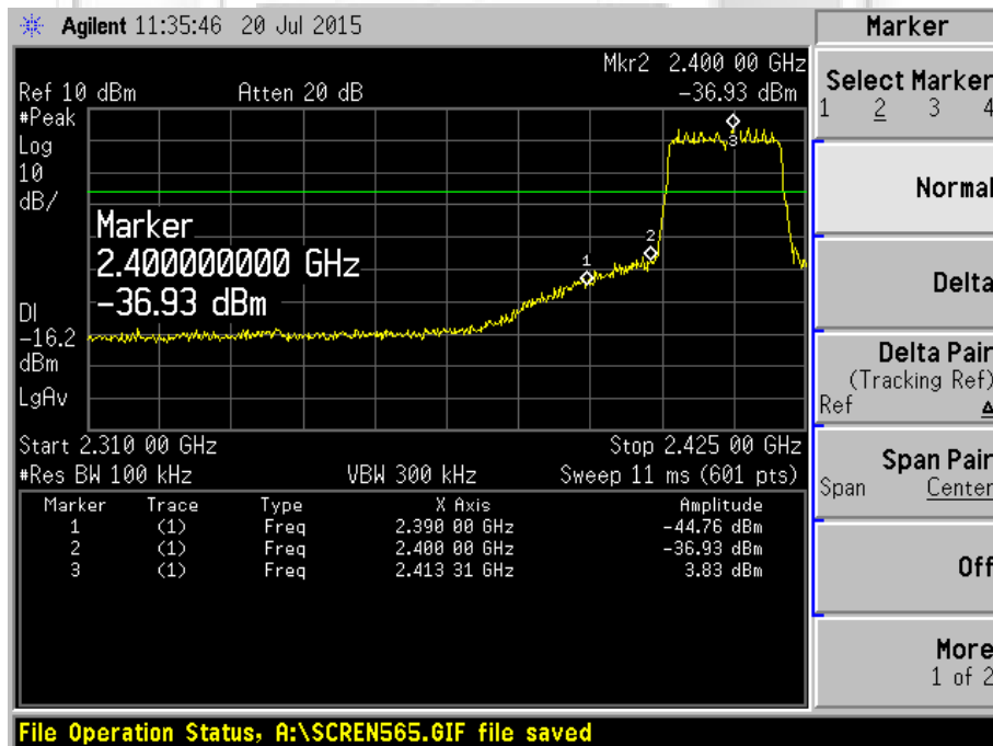
Plot 478 – Lower Band Edge at 2.4000GHz @ QPSK 19.5Mbps
