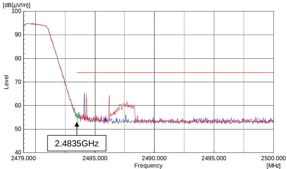
Plot 70 – Peak Plot at Upper Band Edge at 2.4835GHz
