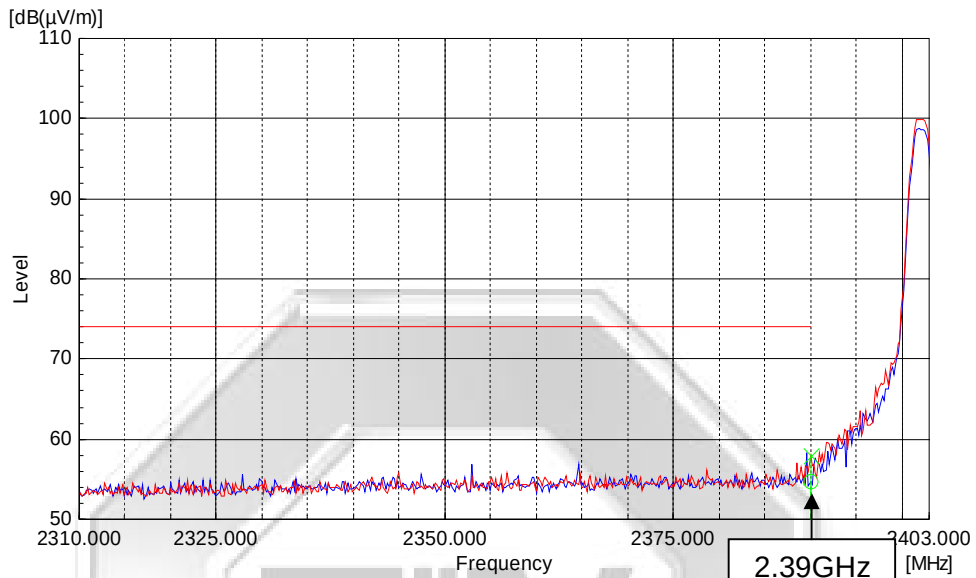
Plot 47 – Peak Plot at Lower Band Edge at 2.4000GHz
