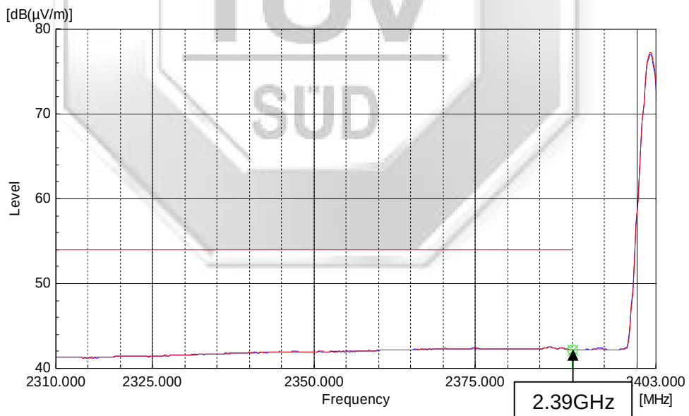
Plot 48 – Average Plot at Lower Band Edge at 2.4000GHz
