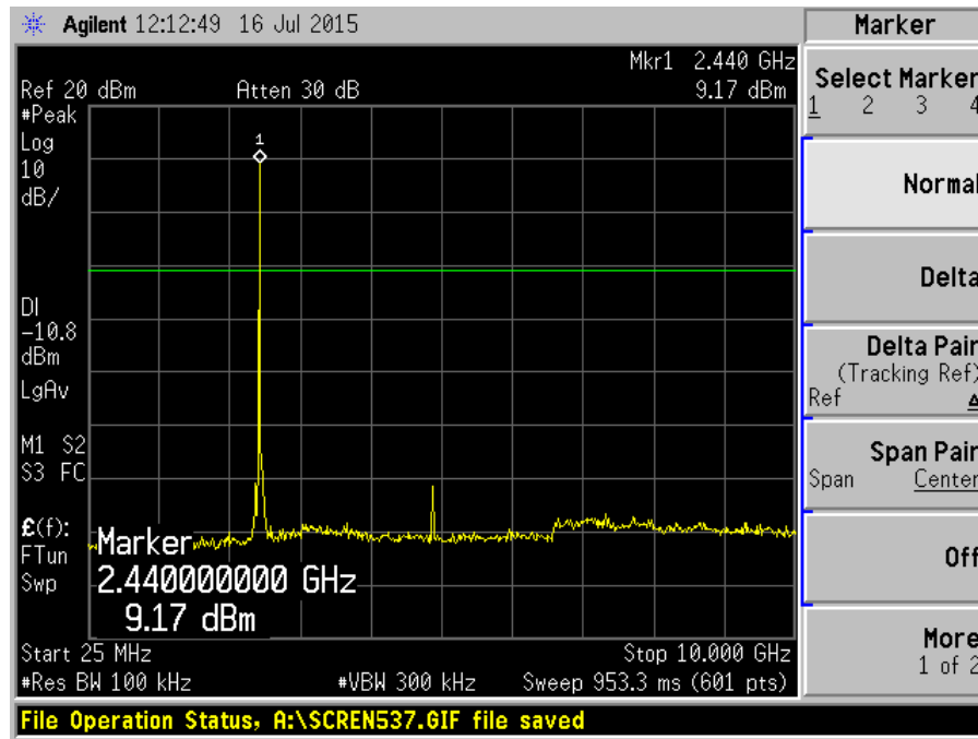
Plot 9 – Channel 19
