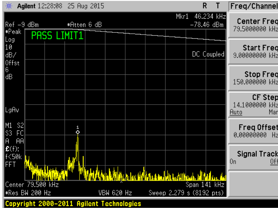
Plot 33 - Channel 39 (upper ch)
