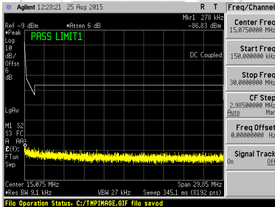
Plot 34 - Channel 39 (upper ch)
