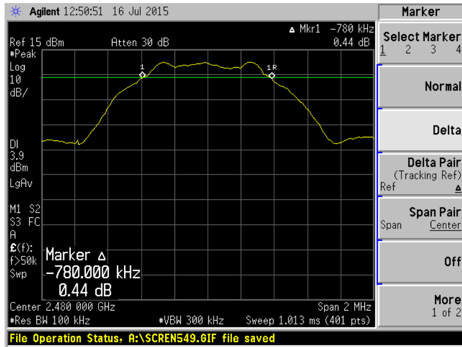
Plot 3 - Channel 39
