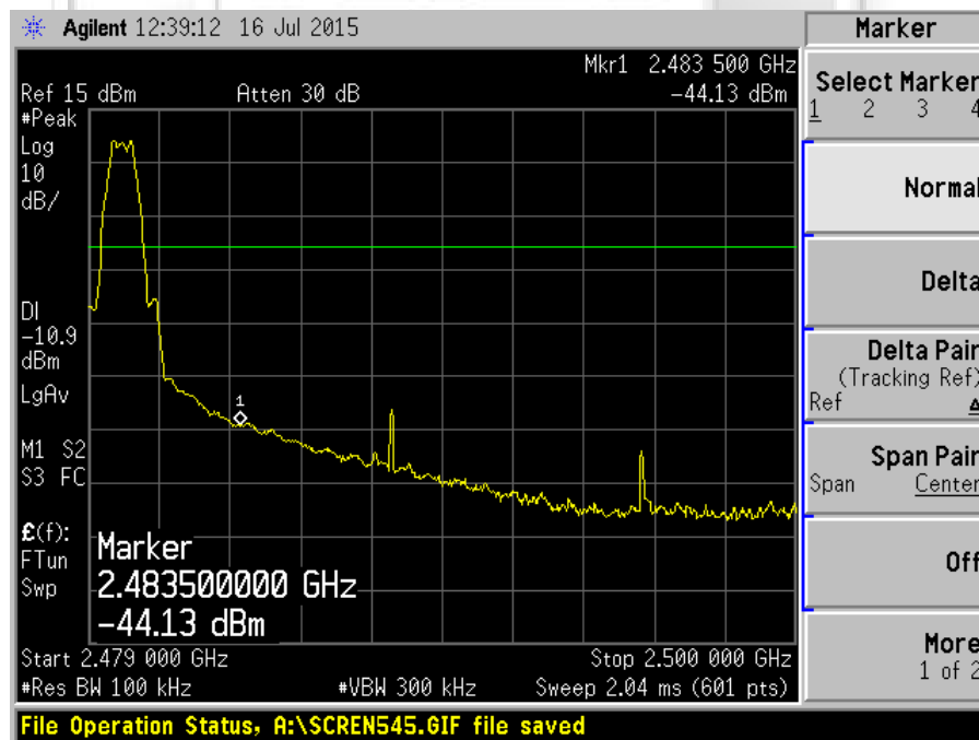
Plot 44 – Upper Band Edge at 2.4835GHz
