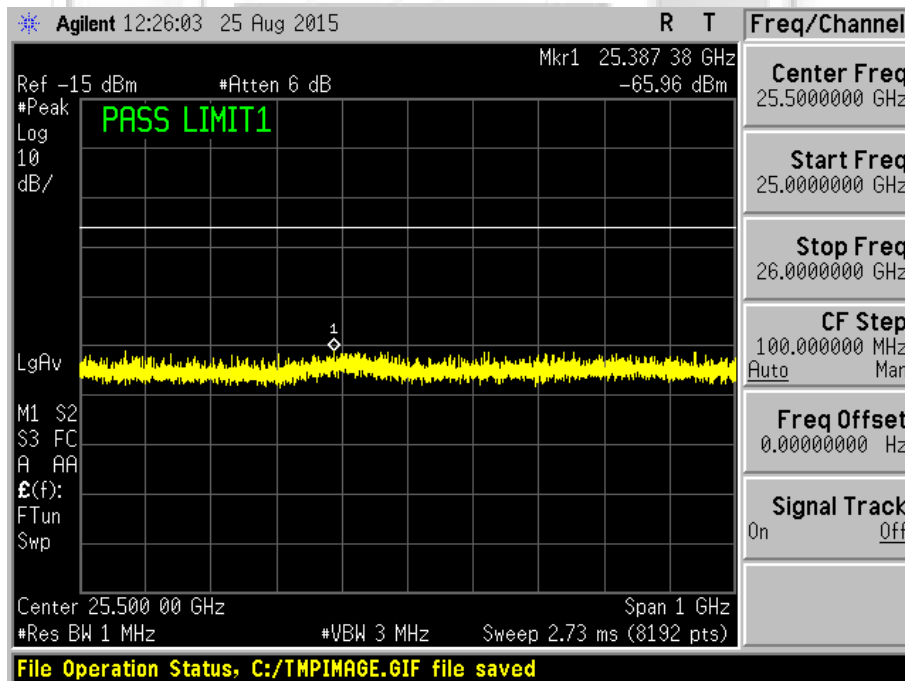
Plot 32 – Channel 19 (middle ch)
