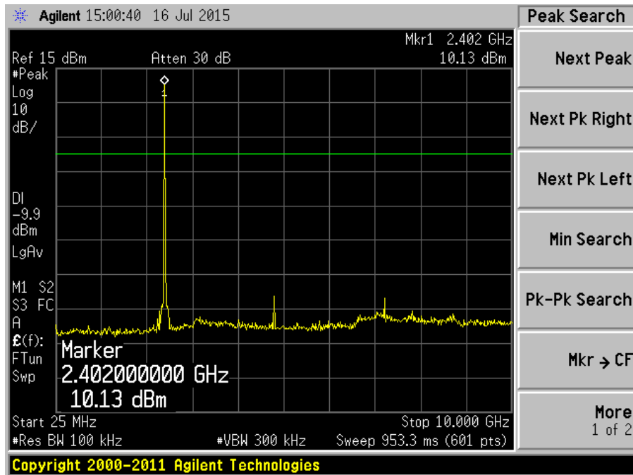
Plot 7 - Channel 0
