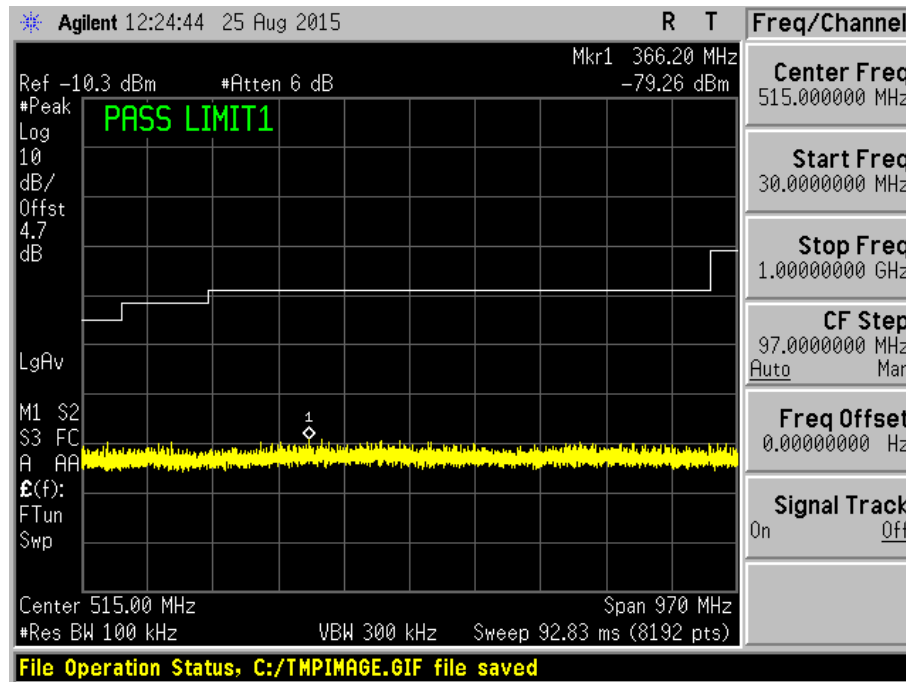
Plot 25 - Channel 19 (middle ch)
