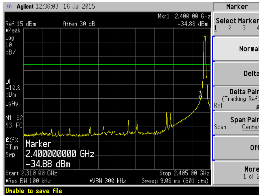
Plot 43 – Lower Band Edge at 2.4000GHz
