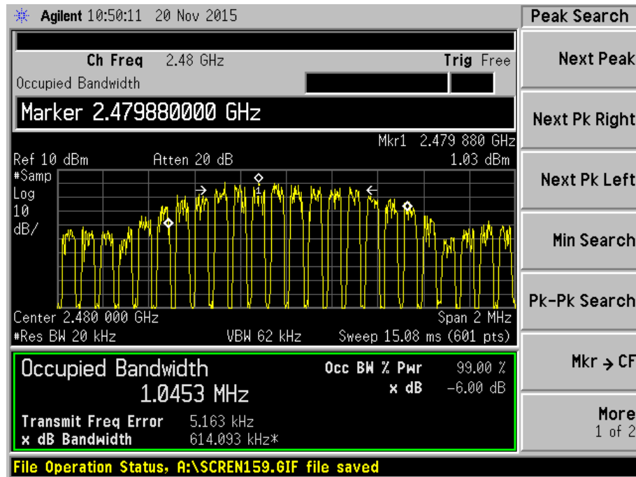
Plot 6 - Channel 39
