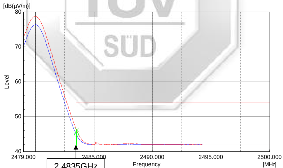
Plot 50 – Average Plot at Upper Band Edge at 2.4835GHz
