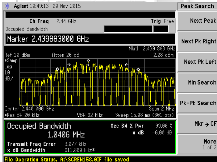
Plot 5 - Channel 19
