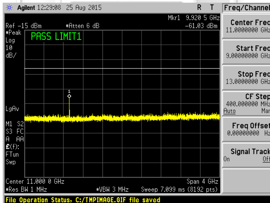
Plot 38 – Channel 39 (upper ch)
