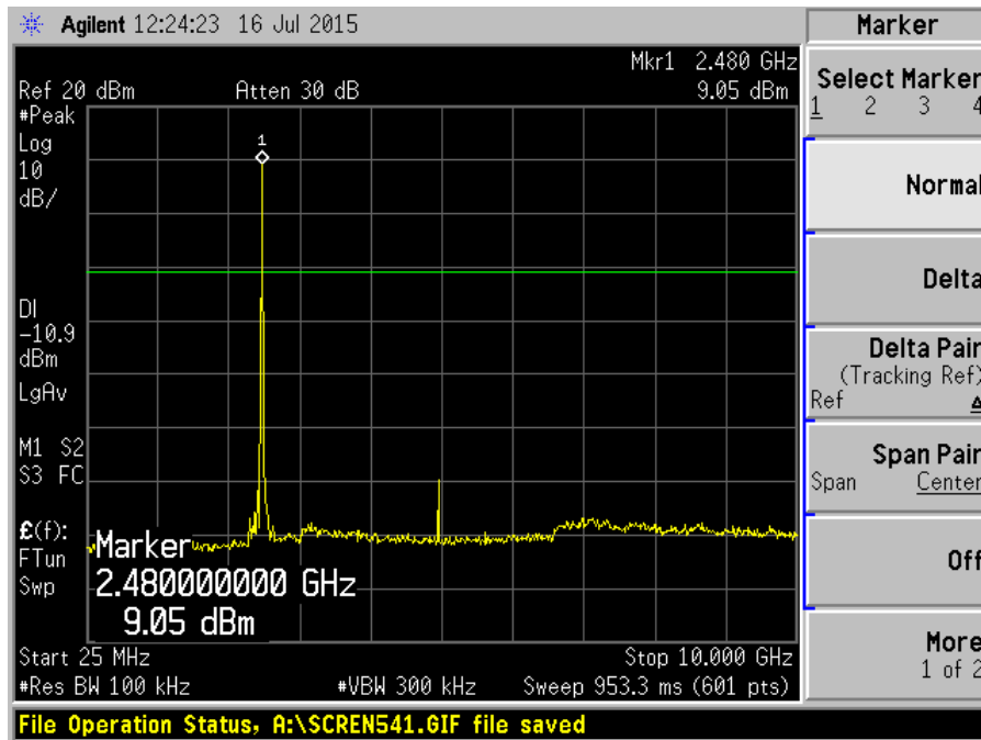
Plot 11 – Channel 39
