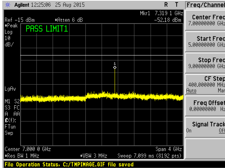
Plot 27 - Channel 19 (middle ch)
