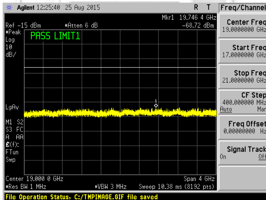
Plot 30 - Channel 19 (middle ch)
