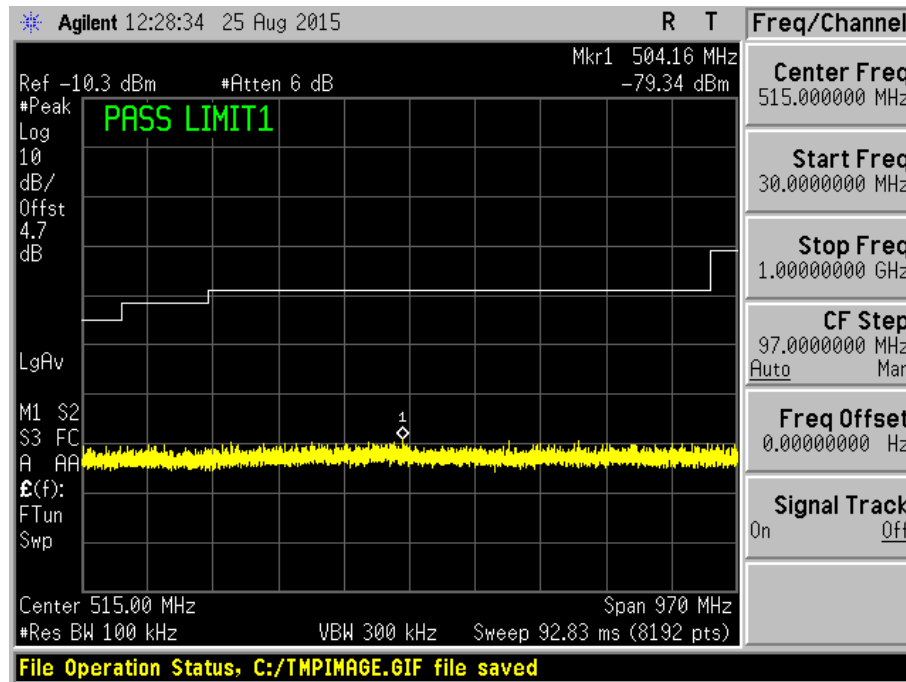
Plot 35 – Channel 39 (upper ch)
