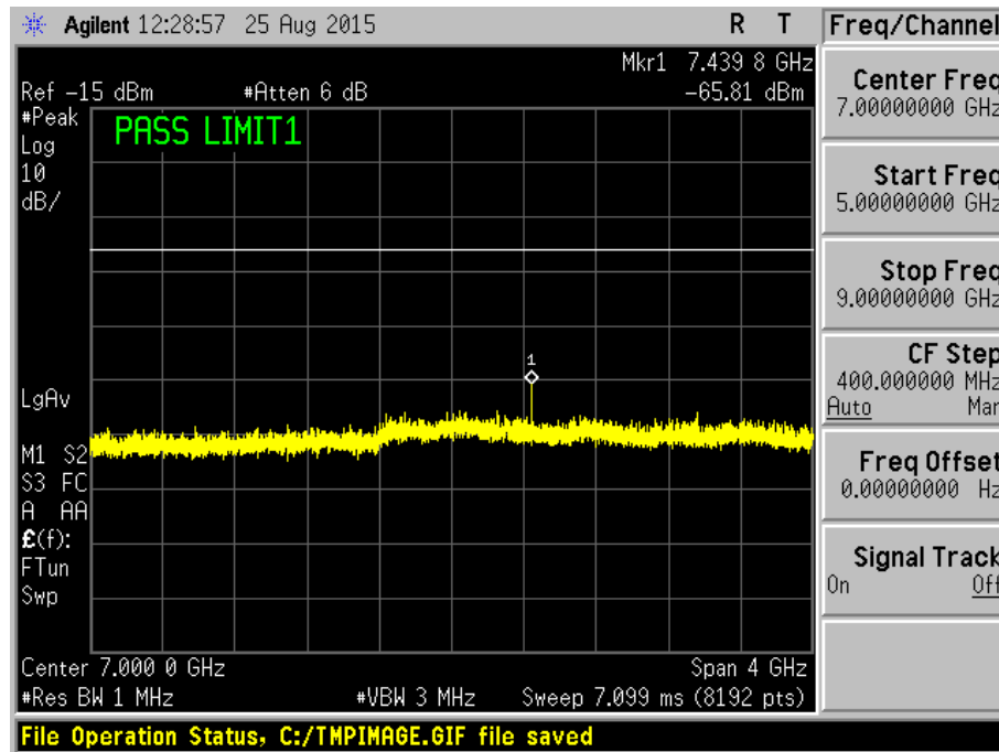
Plot 37 – Channel 39 (upper ch)
