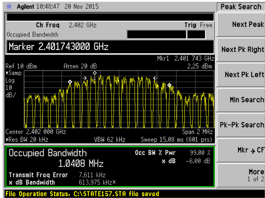
Plot 4 - Channel 0
