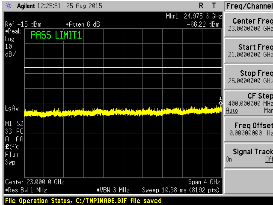
Plot 31 – Channel 19 (middle ch)
