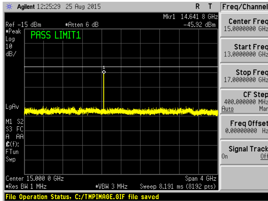
Plot 29 - Channel 19 (middle ch)
