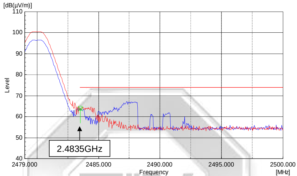
Plot 49 – Peak Plot at Upper Band Edge at 2.4835GHz
