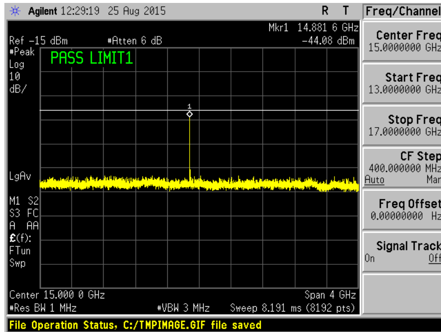
Plot 39 – Channel 39 (upper ch)
