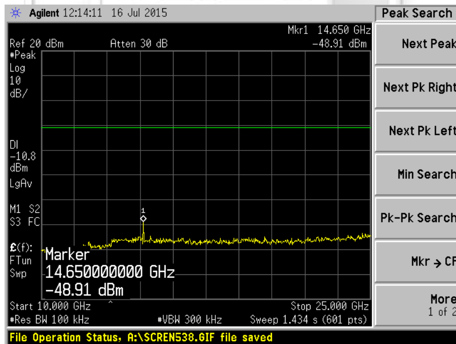
Plot 10 – Channel 19
