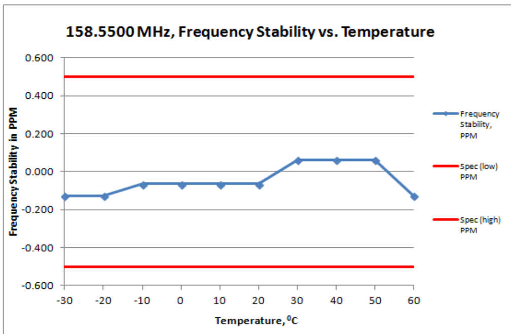
(ii) Frequency Stability VS temperature
