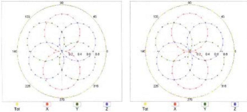
f=600 MHz,TEM
