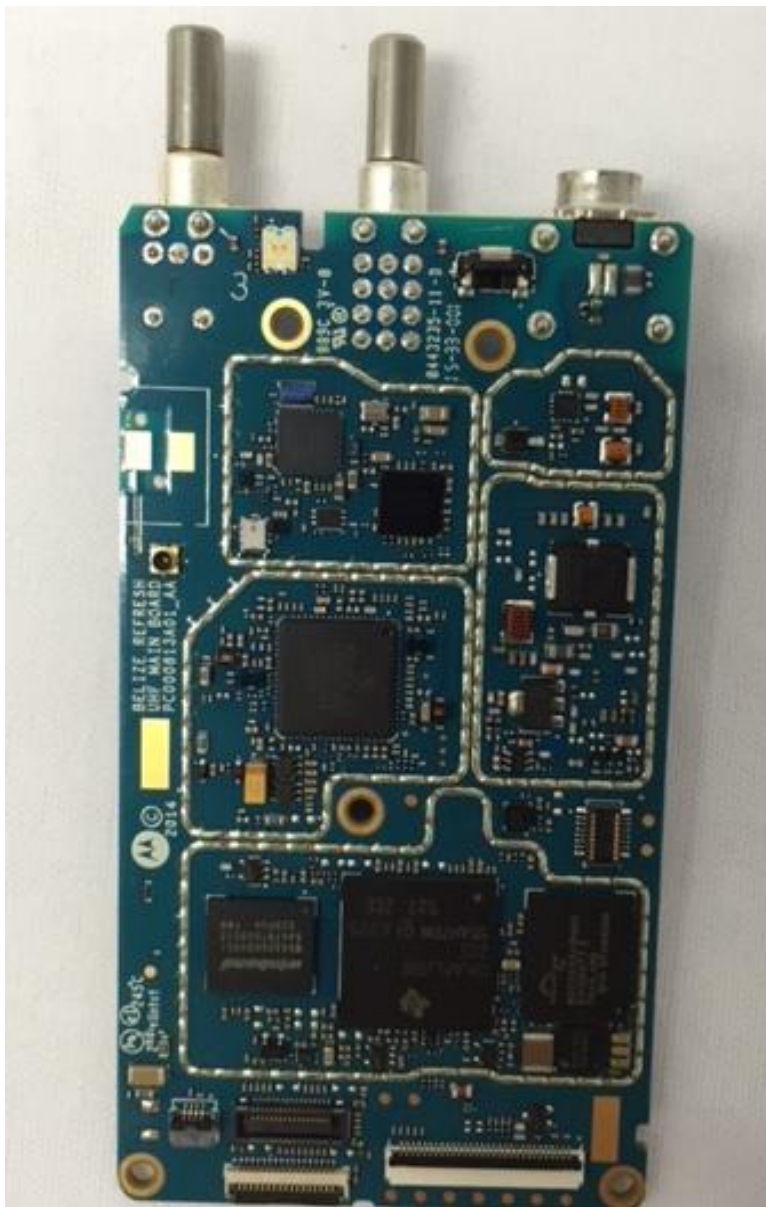
RF board without Shields (Top)
