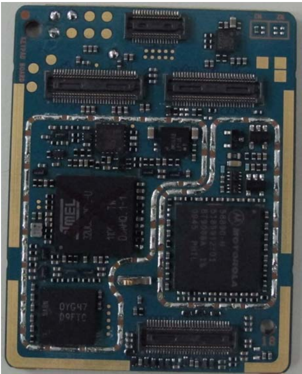
Keypad board without Shields (Bottom)
