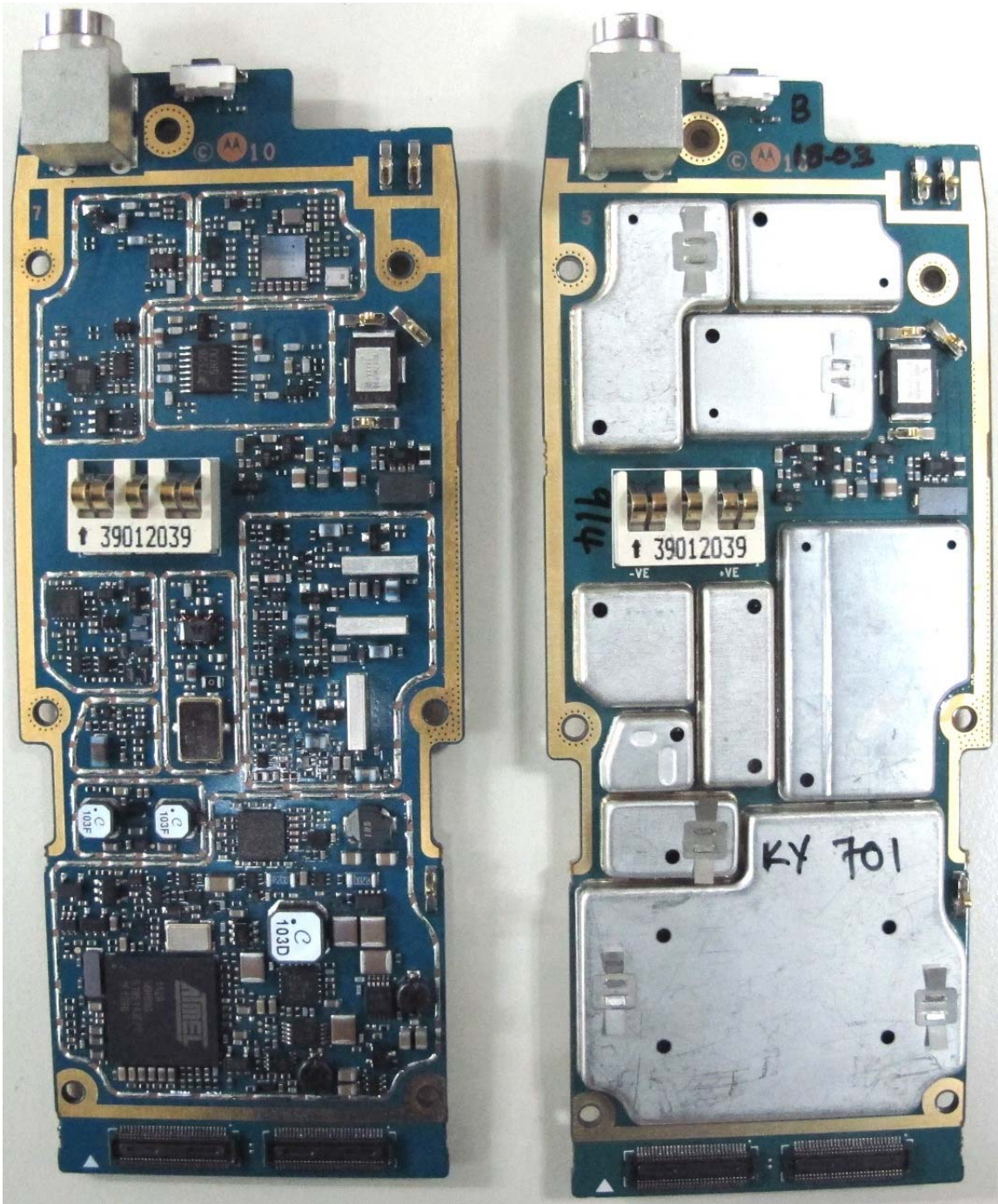
RF board without & with Shields (Bottom)
