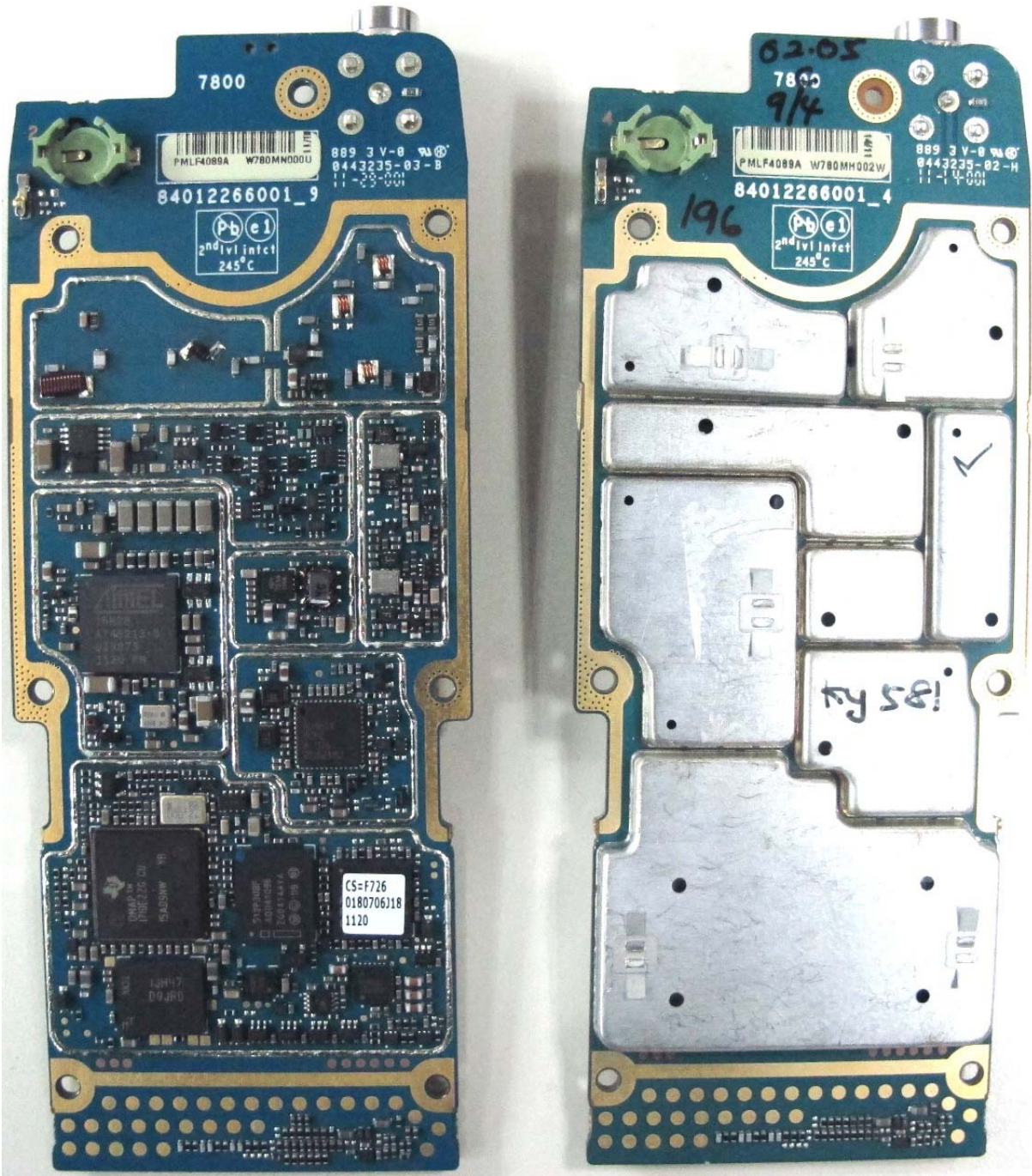
RF board without & with Shields (Top)
