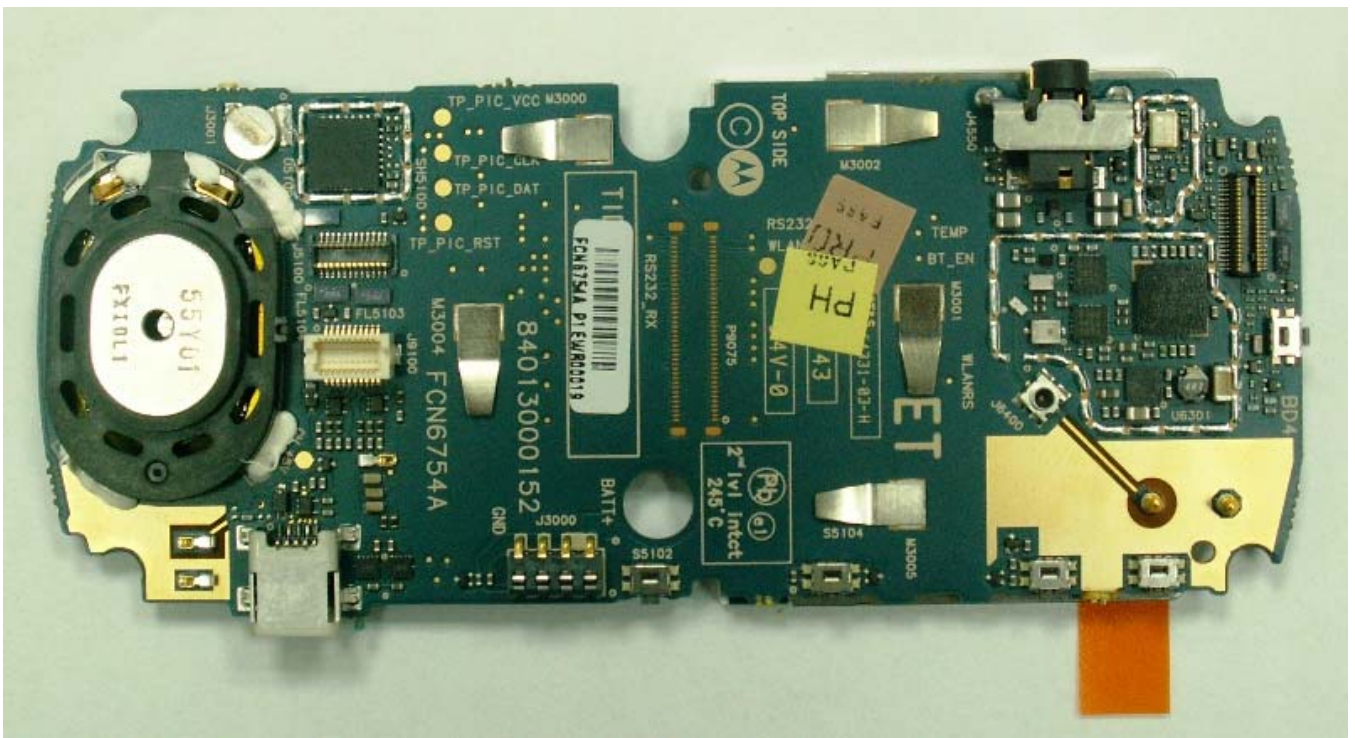
Photograph No. 4 - EWP3100 – Bottom Side no Shields
