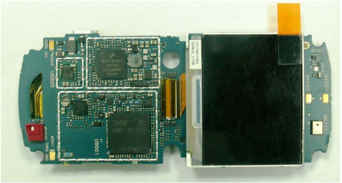
Photograph No. 3 - EWP3100 – Top Side no Shields
