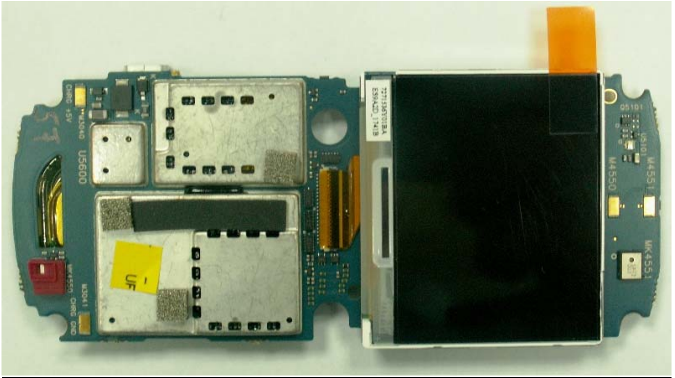
Photograph No. 1 - EWP3100 - Top Side with Shields
