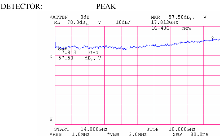
Plot 6.17.79: Tx Radiated emission measurements, 14 - 18GHz, at the mid carrier frequency, 802.11g mode.
