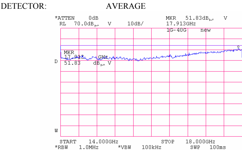
Plot 6.17.78: Tx Radiated emission measurements, 14 - 18GHz, at the low carrier frequency, 802.11g mode.
