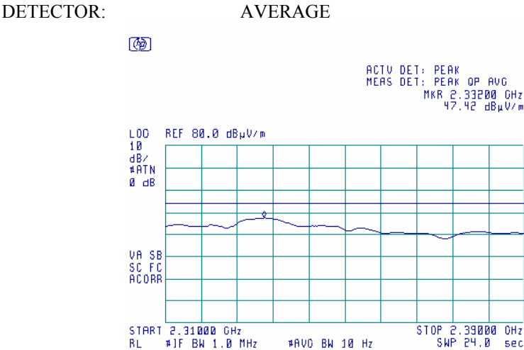
Plot 6.17.51: Tx Radiated emission measurements, 2310 - 2390MHz, at the high carrier frequency, 802.11g mode.
