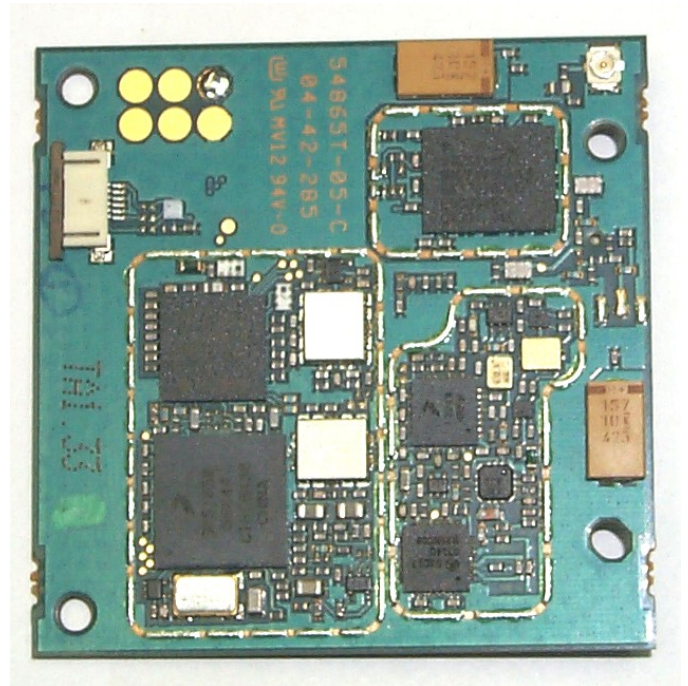
Photograph 9-4: Bottom side of module board with shields removed.
