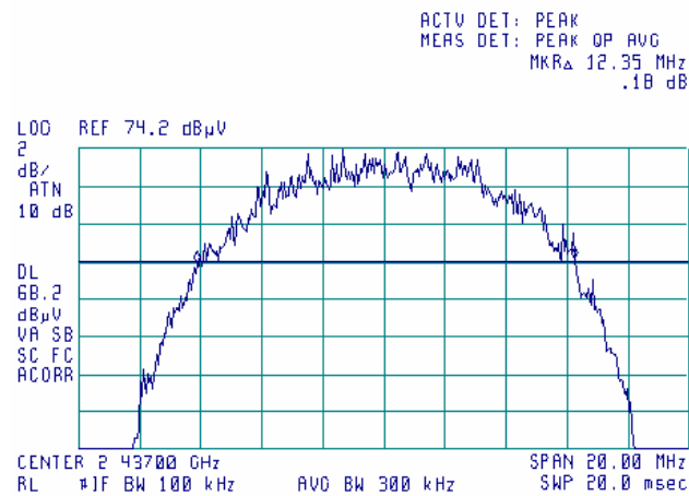
Plot 7.1.8 The 6 dB bandwidth test result at mid frequency, bitrate 11 Mbit/s
