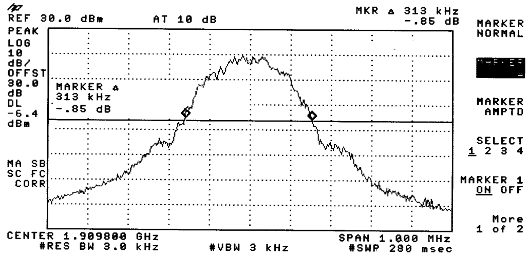
Fig.8.6: Channel 810, -26dB BC Bandwidth
