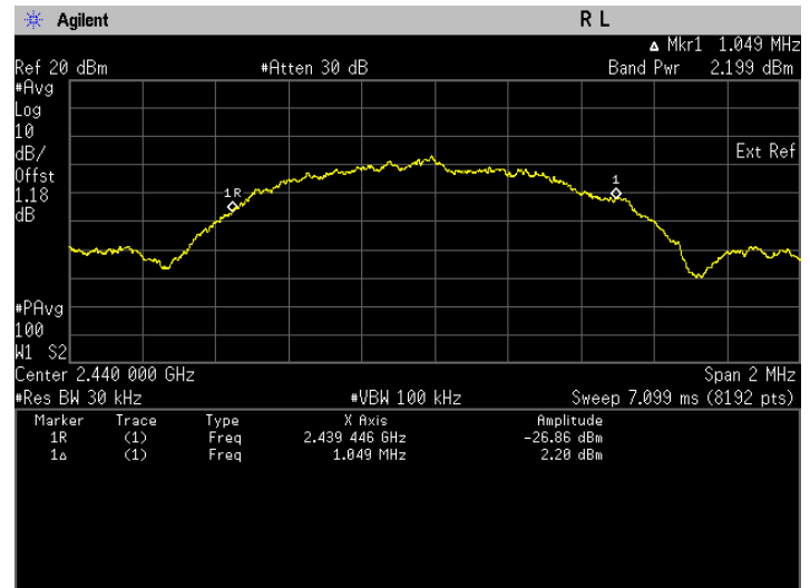
Maximum Peak Conducted RF Output Power. Bluetooth LE Frequency 2440 MHz
