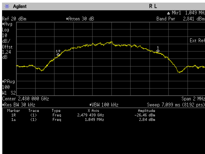
Maximum Peak Conducted RF Output Power. Bluetooth LE Frequency 2480 MHz
