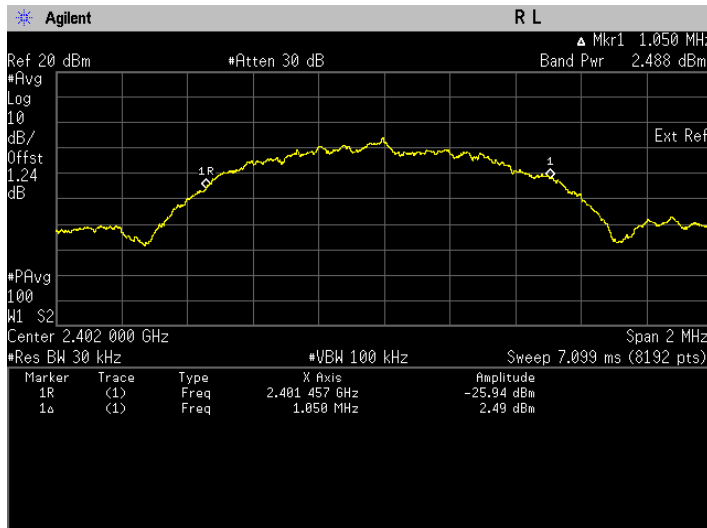
Maximum Peak Conducted RF Output Power. Bluetooth LE Frequency 2402 MHz
