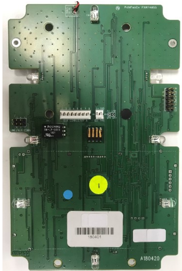
Board Side 2
