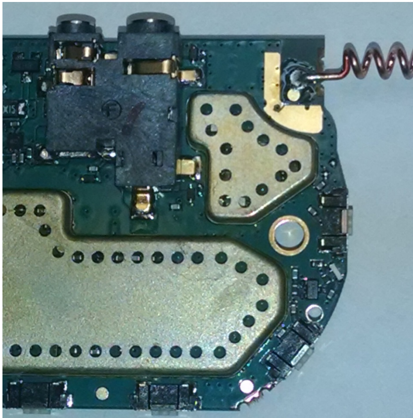
Figure 9-6 Bottom Side Internal photo W/Antenna
