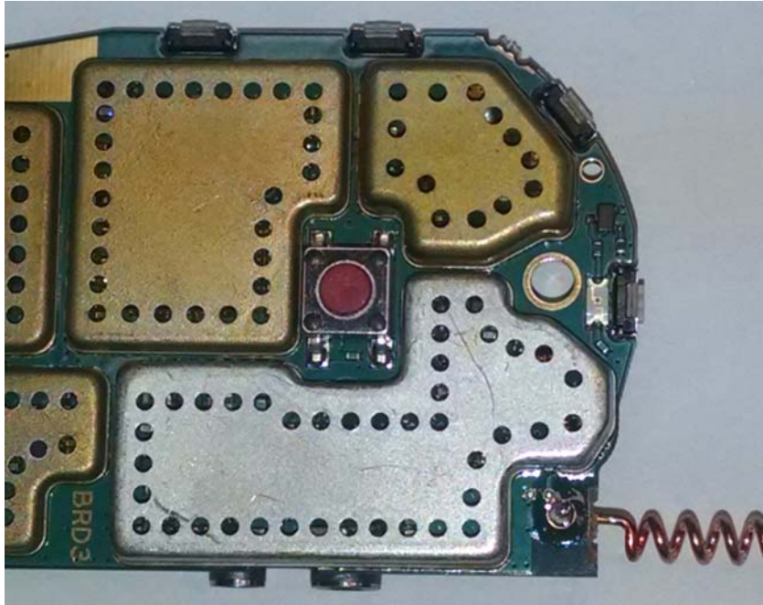
Figure 9-5 Top Side Internal photo W/Antenna
