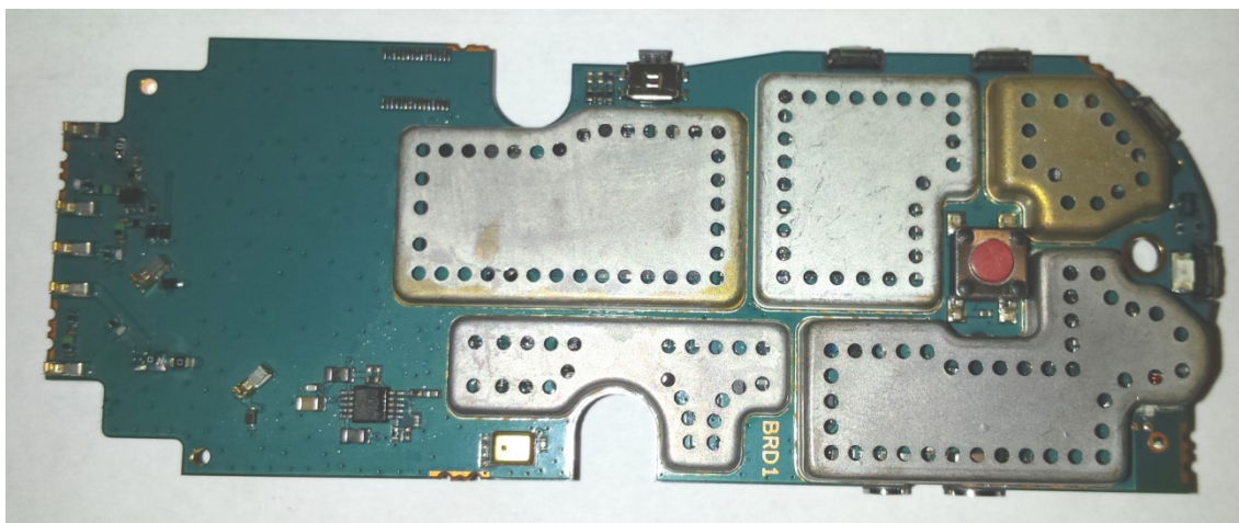
Figure 9-3 Top Side Internal photo with shields intact.
