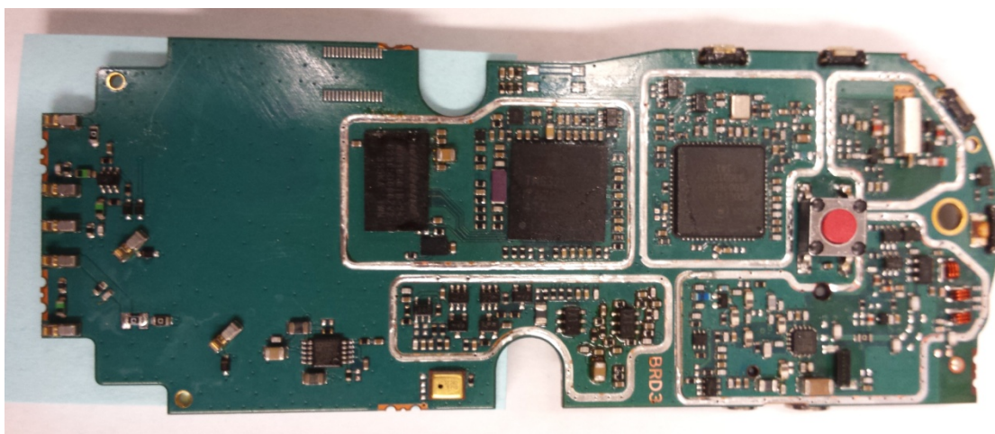
Figure 9-4 Top Side Internal photo without shields.
