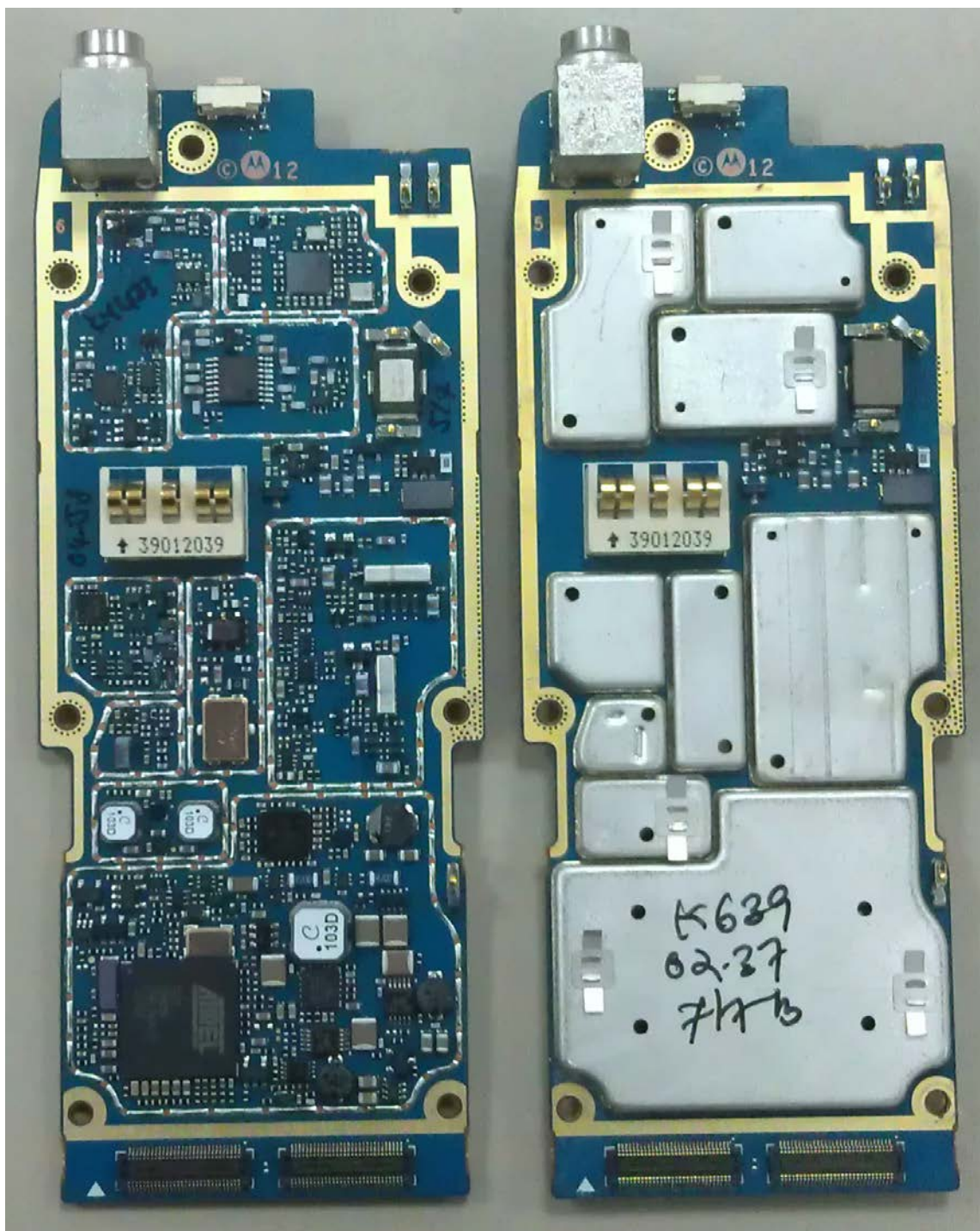
RF board without & with Shields (Bottom)
