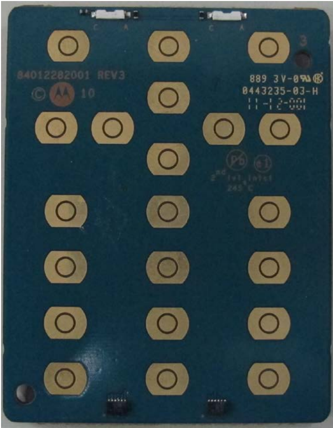
Keypad Board (Top)
