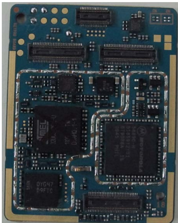
Keypad board without Shields (Bottom)
