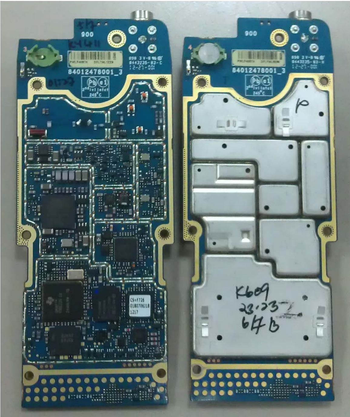
RF board without & with Shields (Top)
