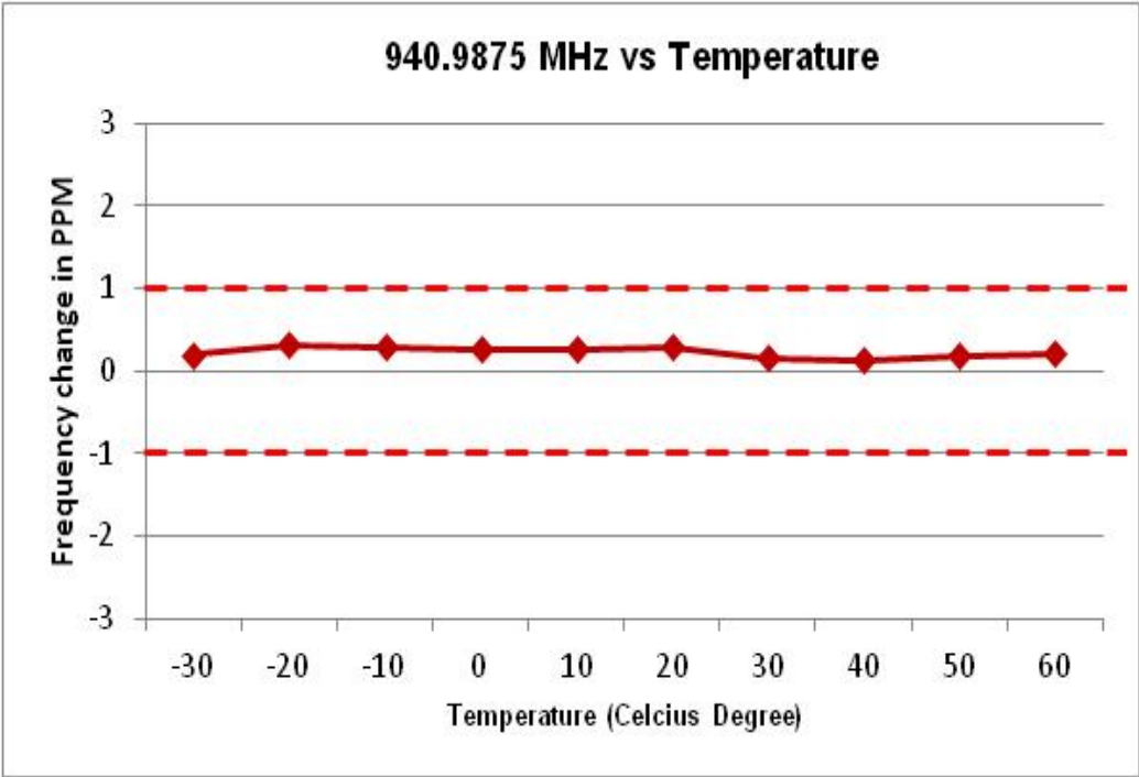
Frequency Stability (940.9875 MHz) vs. Temperature
