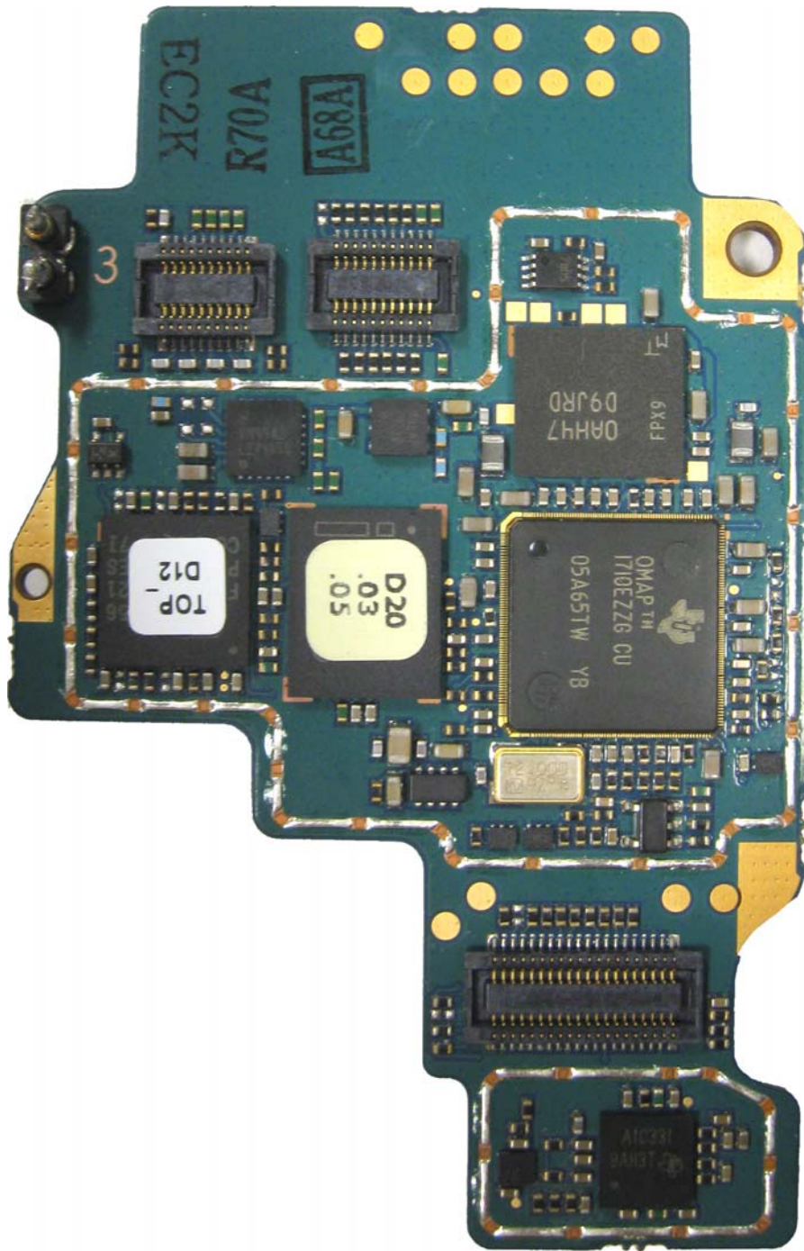
Vocon board without shields board (Bottom)
