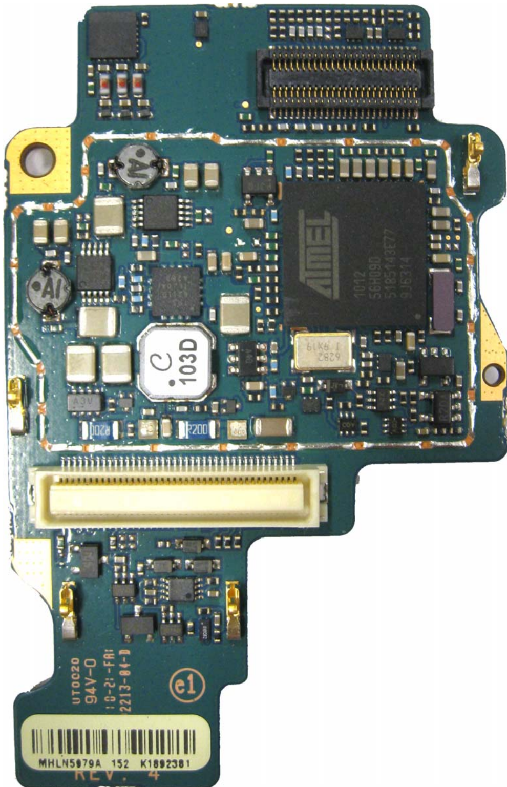
Vocon board without Shields (Top)
