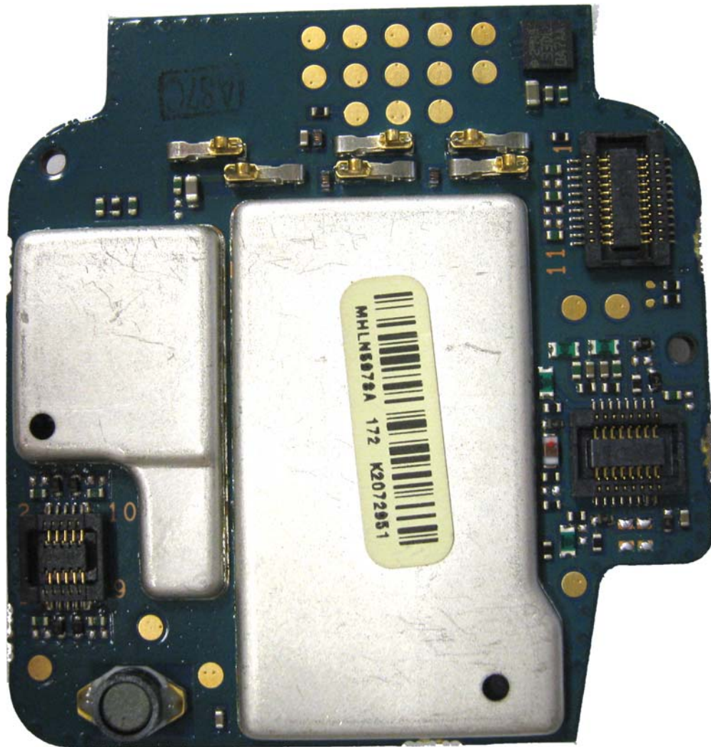
Expander board with shields board (Bottom)
