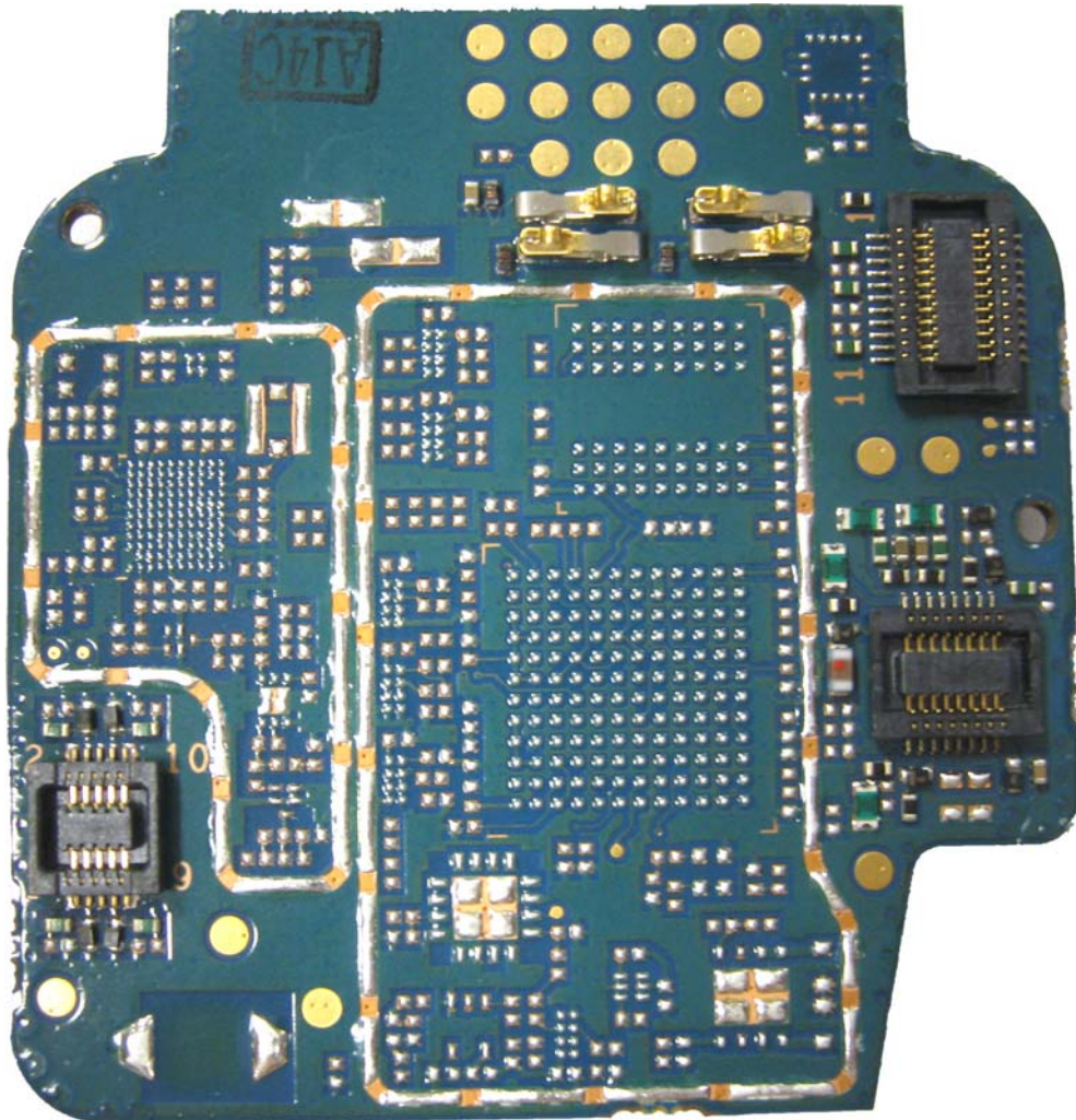
Expander board without shields board (Bottom)
