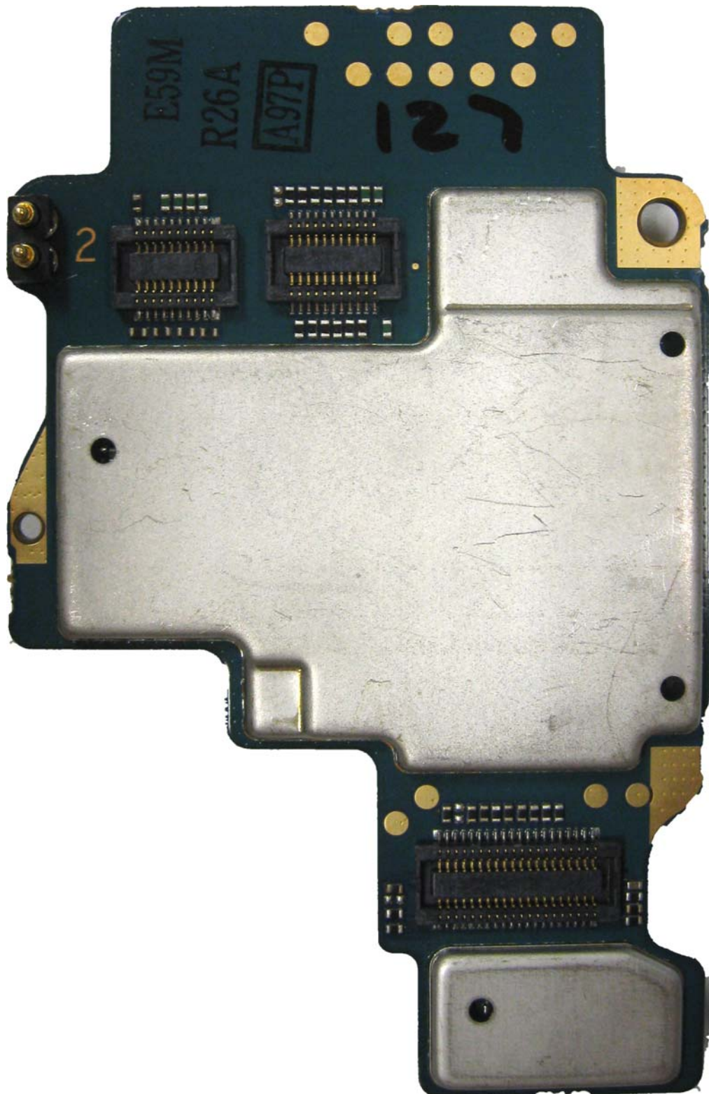
Vocon board with shields board (Bottom)
