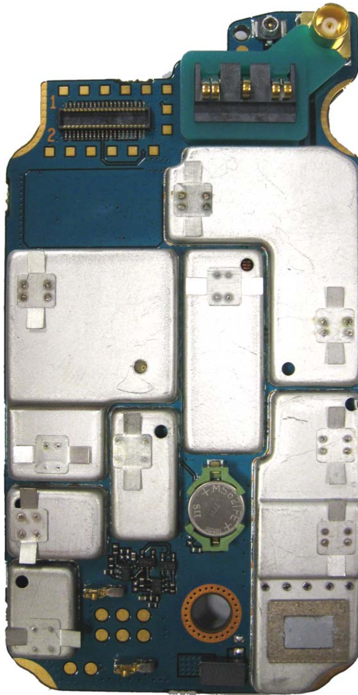
RF board with Shields (Top)
