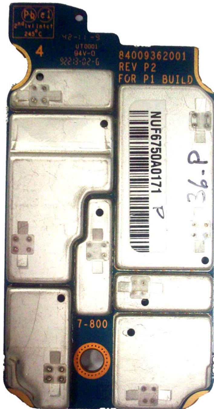
RF board with Shields (Bottom)
