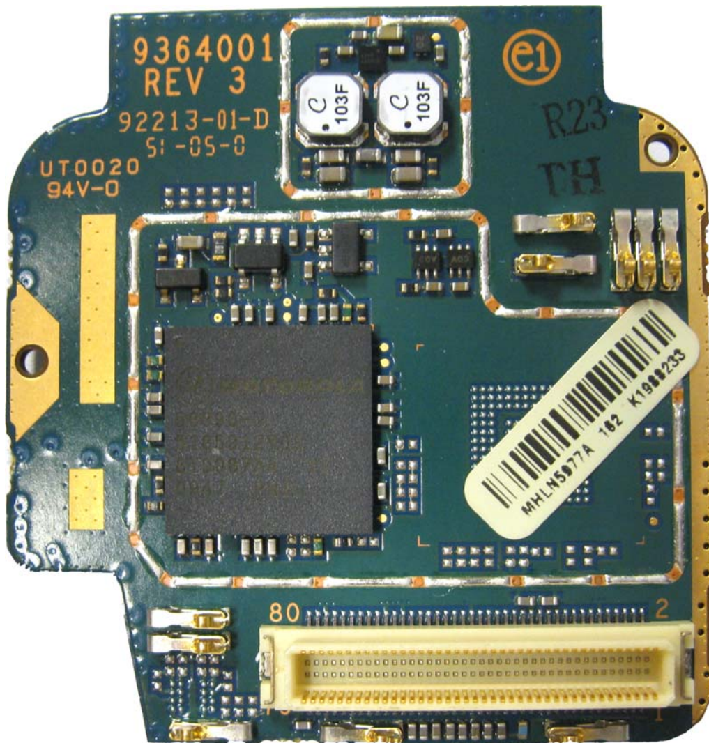
Expander board without shields board (Bottom)
