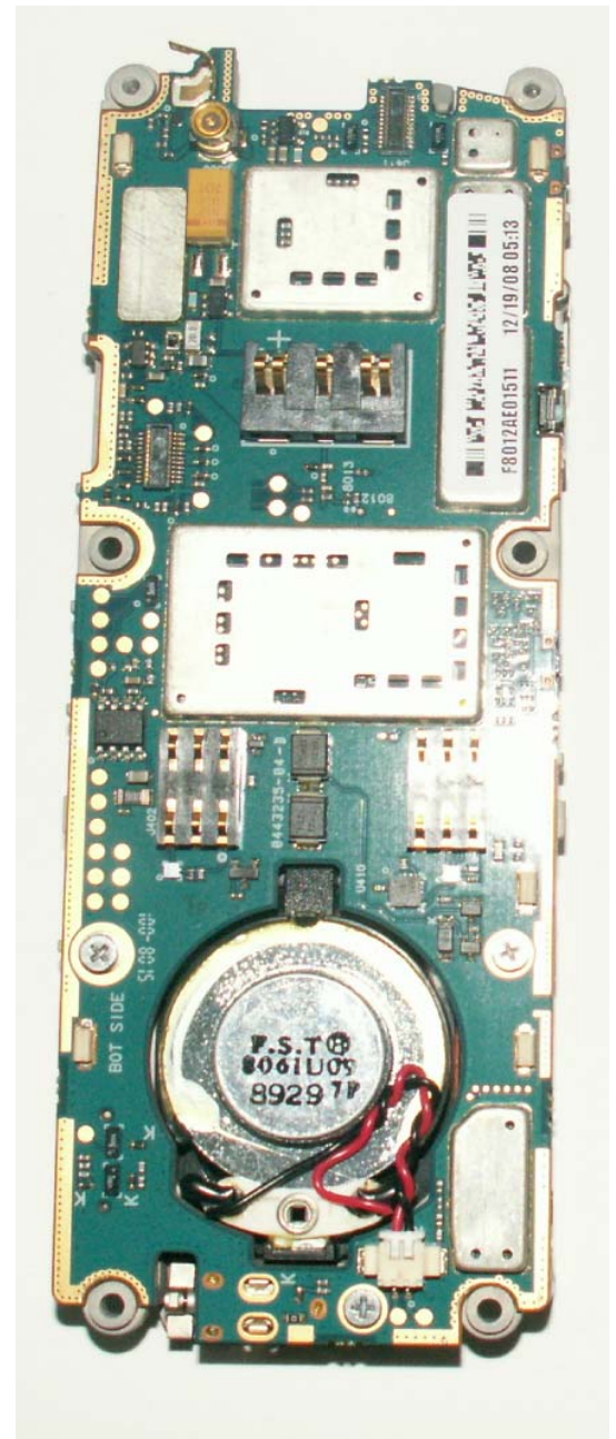
Photograph 9-4: Bottom side of main PC Board with shields.
