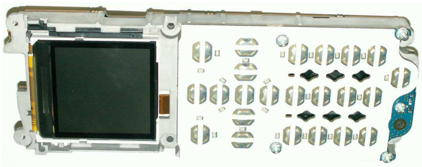
Photograph 9-8: Front view of internal assembly, showing display and keypadboard.
