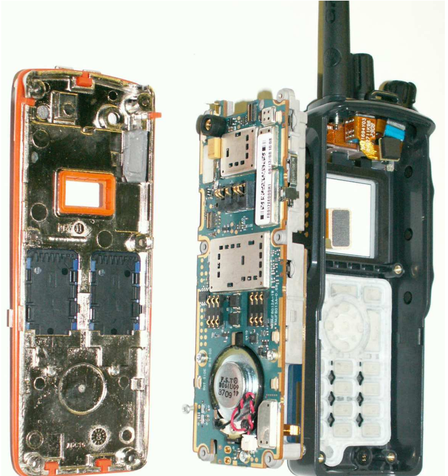
Photograph 9-6: View from back, back-chassis removed, internal assembly separated, uncovering front housing insides.
