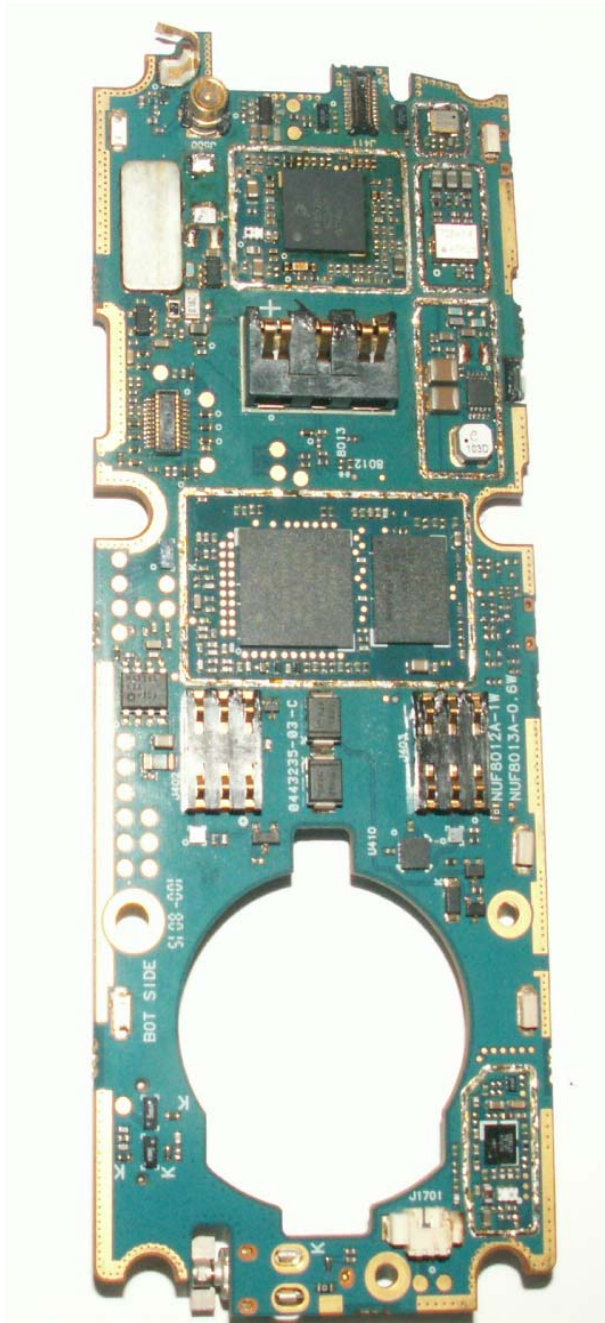
Photograph 9-3: Bottom side of main PC Board without shields.
