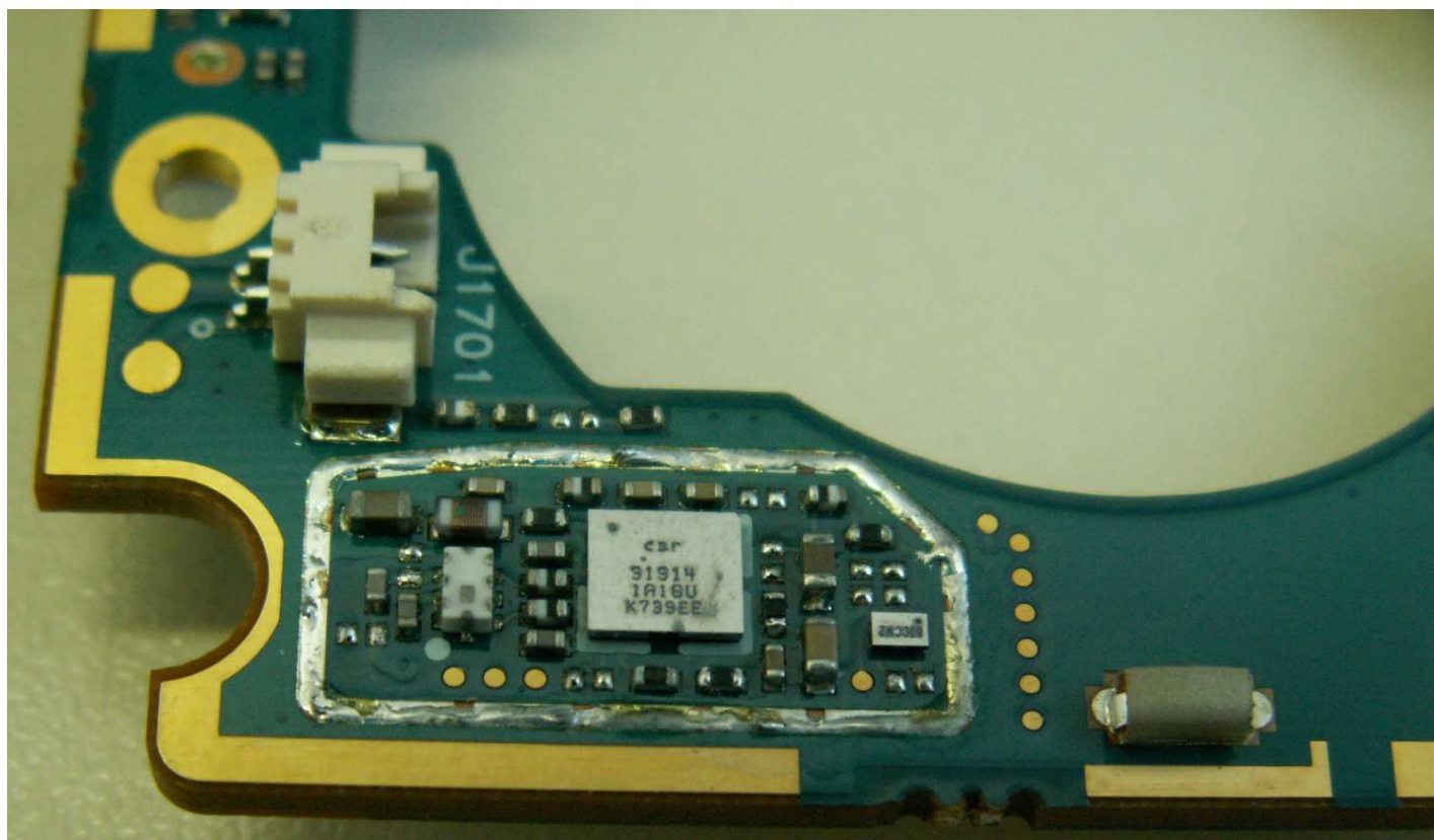
Photograph 9-5: Bottom side of main PC Board showing BT chip.
