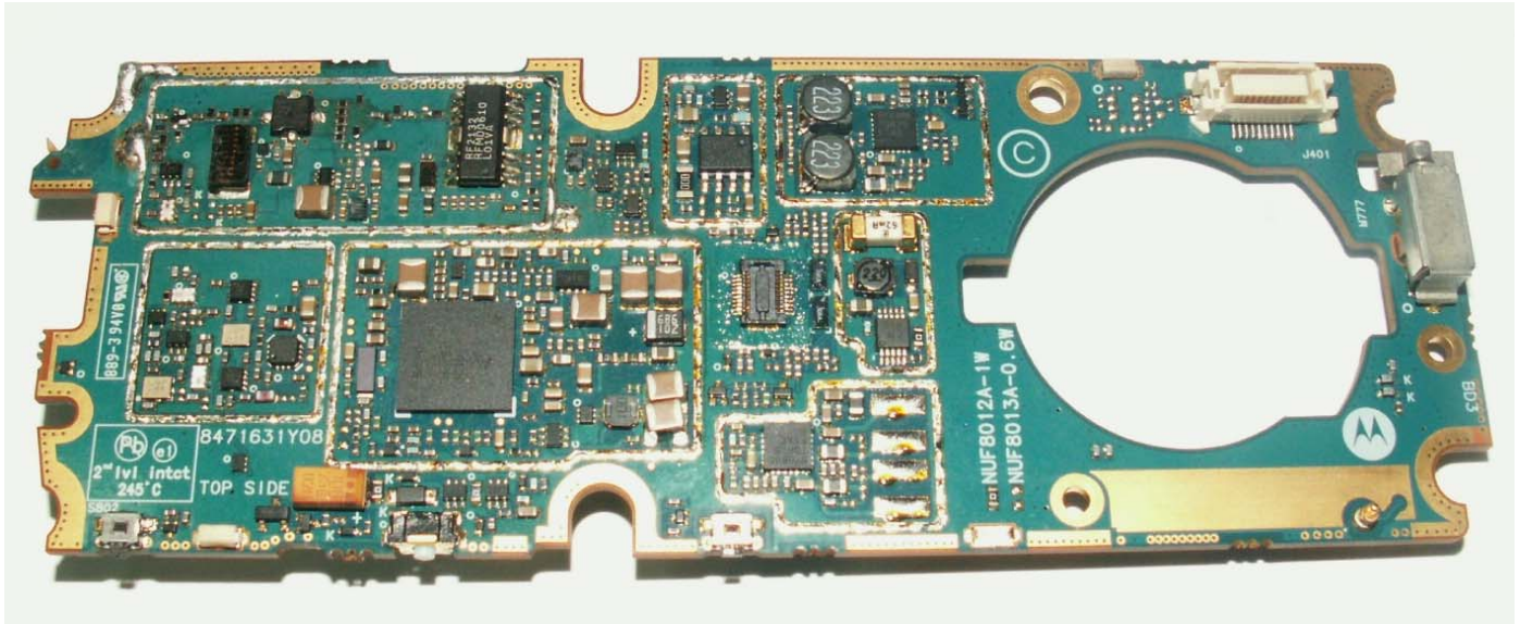
Photograph 9-1: Top side of main PC Board without shields
