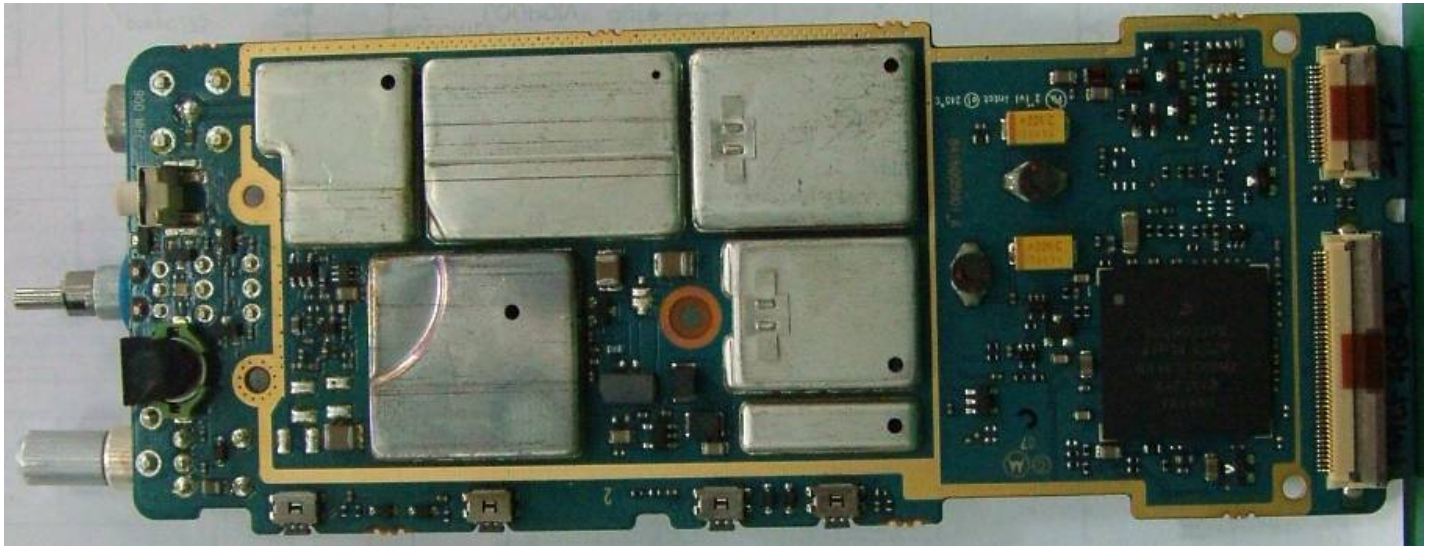
Figure 9-1: Top Side of PCB with shields
