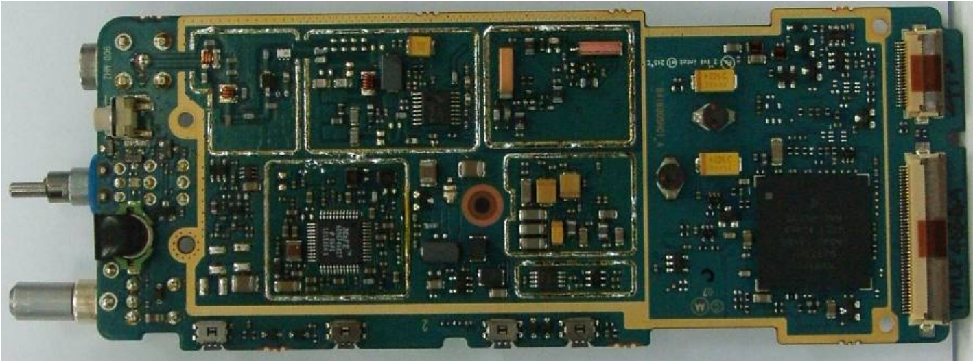
Figure 9-3: Top Side of PCB without shields
