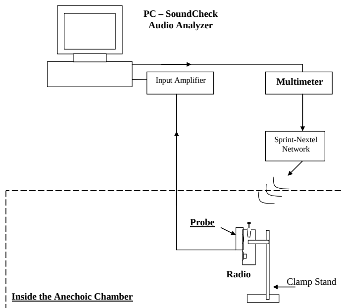
Figure 5-1 – Test setup
