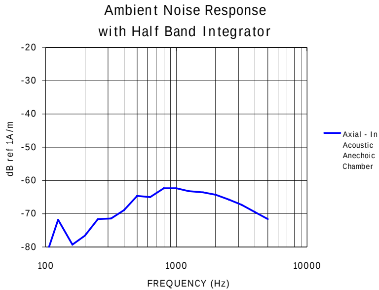
Figure 12A– Axial Ambient Magnetic frequency distribution
