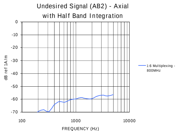
Figure 14B – 800MHz Undesired Signal (1:6)
