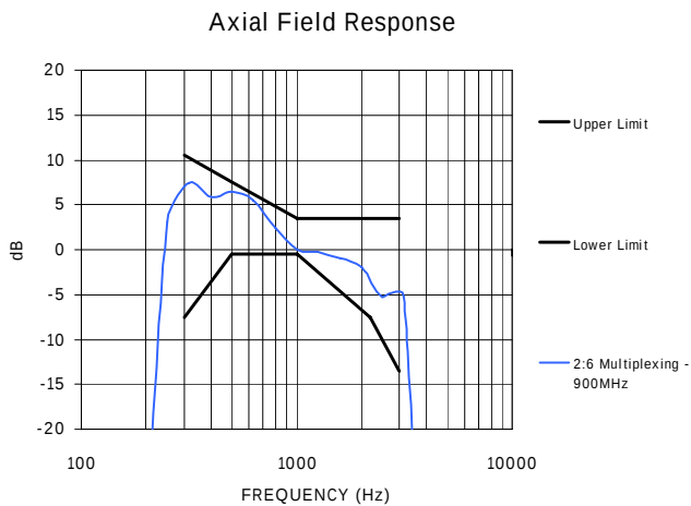
Figure 13C – 900MHz Measured Frequency response
