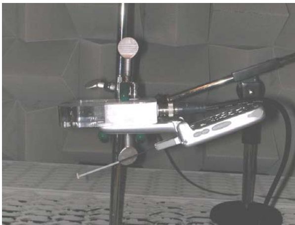
Figure 10 – Test holder
