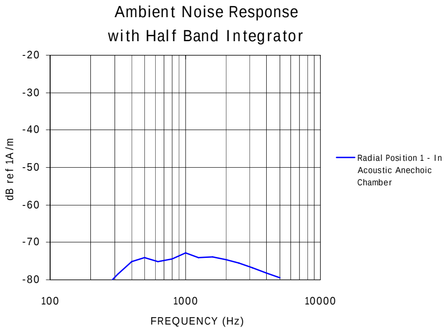
Figure 12B – Radial Position 1 Ambient Magnetic frequency distribution
