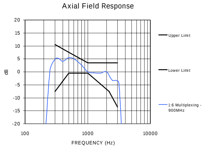
Figure 13D – 900MHz Measured Frequency response
