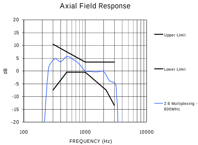
Figure 13A – 800MHz Measured Frequency response
