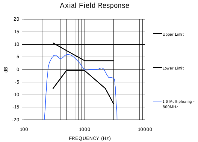
Figure 13B – 800MHz Measured Frequency response
