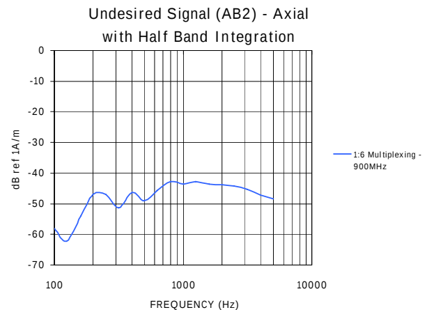
Figure 15B – 900MHz Undesired Signal (1:6)
