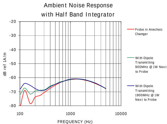
Figure 9 – Noise with RF Measured Response
