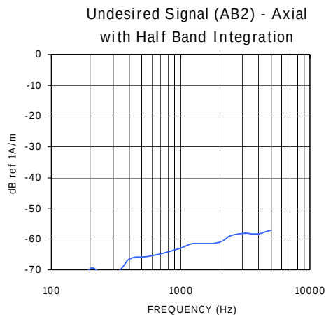
Figure 14A – 800MHz Undesired Signal (2:6)
