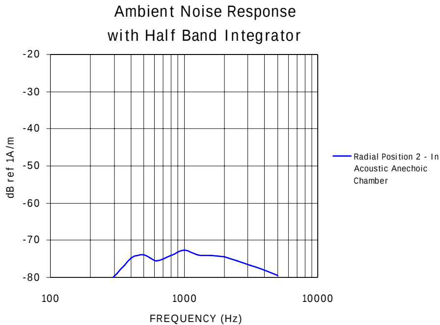
Figure 12C – Radial Position 2 Ambient Magnetic frequency distribution
