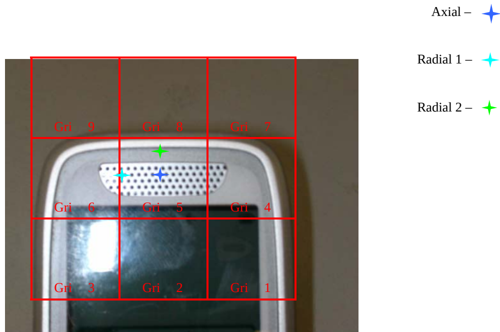
Figure 9 – Measurement Locations
