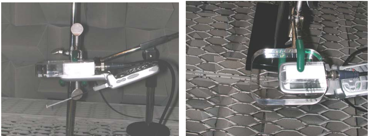
Figure 8 – Test holder
