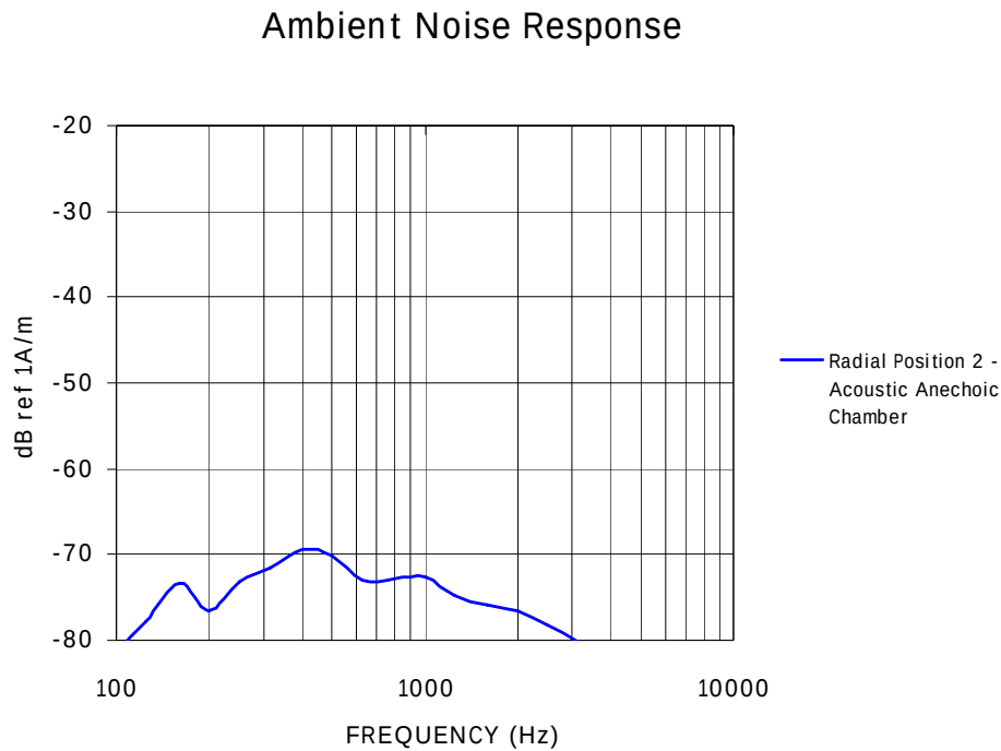
Figure 9C – Radial Position 2 Ambient Magnetic frequency distribution
