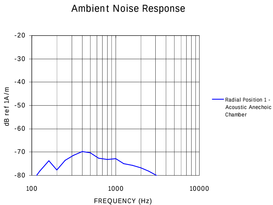
Figure 9B – Radial Position 1 Ambient Magnetic frequency distribution
