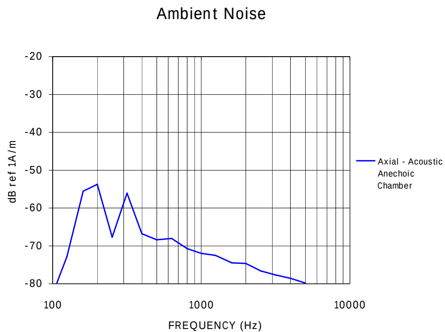
Figure 9A– Axial Ambient Magnetic frequency distribution
