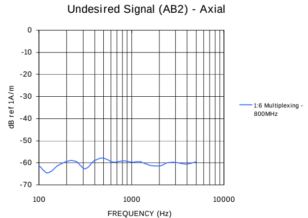
Figure 11B – 800MHz Undesired Signal (1:6)
