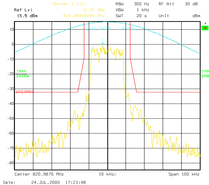
Figure 6a-2.3.3. WiDEN25 800 MHz Band, Quad-QPSK, Maximum Power, EA Emission Mask
