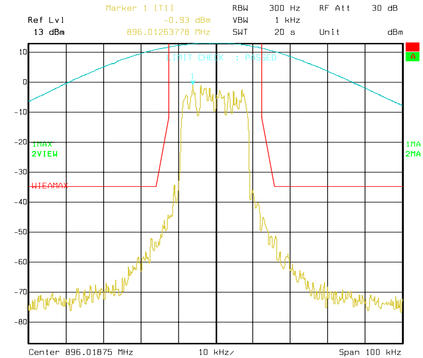
Date: 25.JUL.2005 20:53:55 Figure 6a-2.8.3. WiDEN25 900 MHz Band, QAM16, Maximum Power, EA Emission Mask
