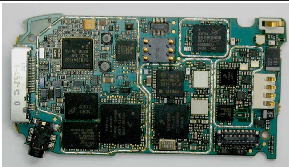
Photograph 9-3: Back side view of radio PC Board, without shields.
