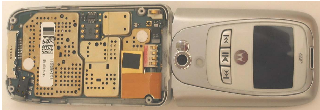
Photograph 9-1: Back side view of radio product PC Board
