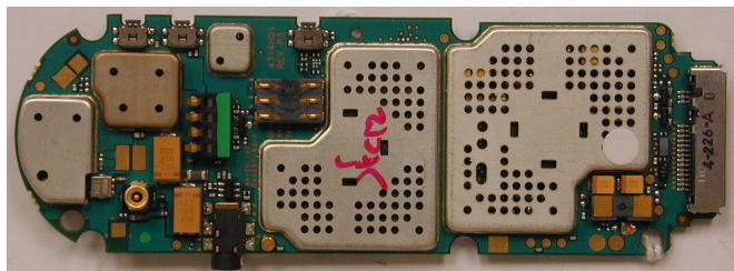
Photograph 9-1: Back side view of radio PCB.
