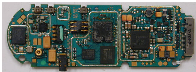
Photograph 9.3: Back side view of radio PCB without shields.
