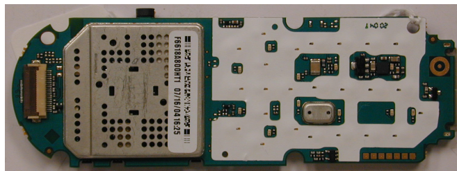
Photograph 9-2: Front side view of radio PCB.
