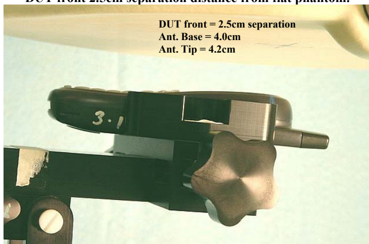
Figure 7. Assessment @ Body DUT w/ holster model NNTN4747A against the flat phantom
