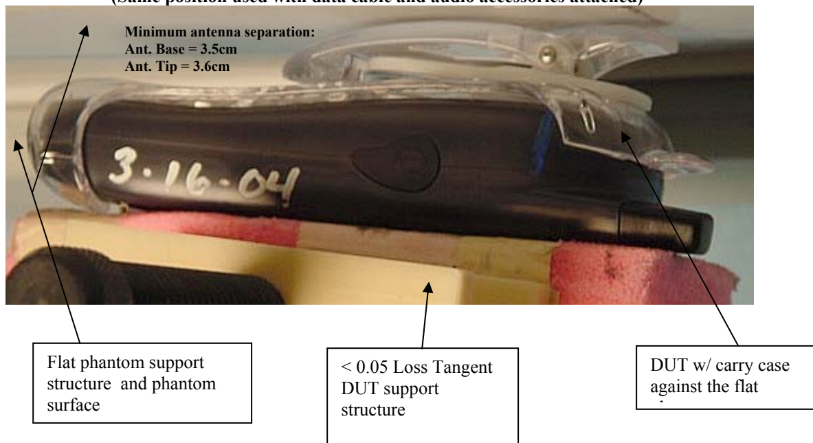
Figure 1: Highest S.A.R. Test Position (@ body) DUT with carry case model NNTN5510A against the flat phantom. (Same position used with data cable and audio accessories attached)
