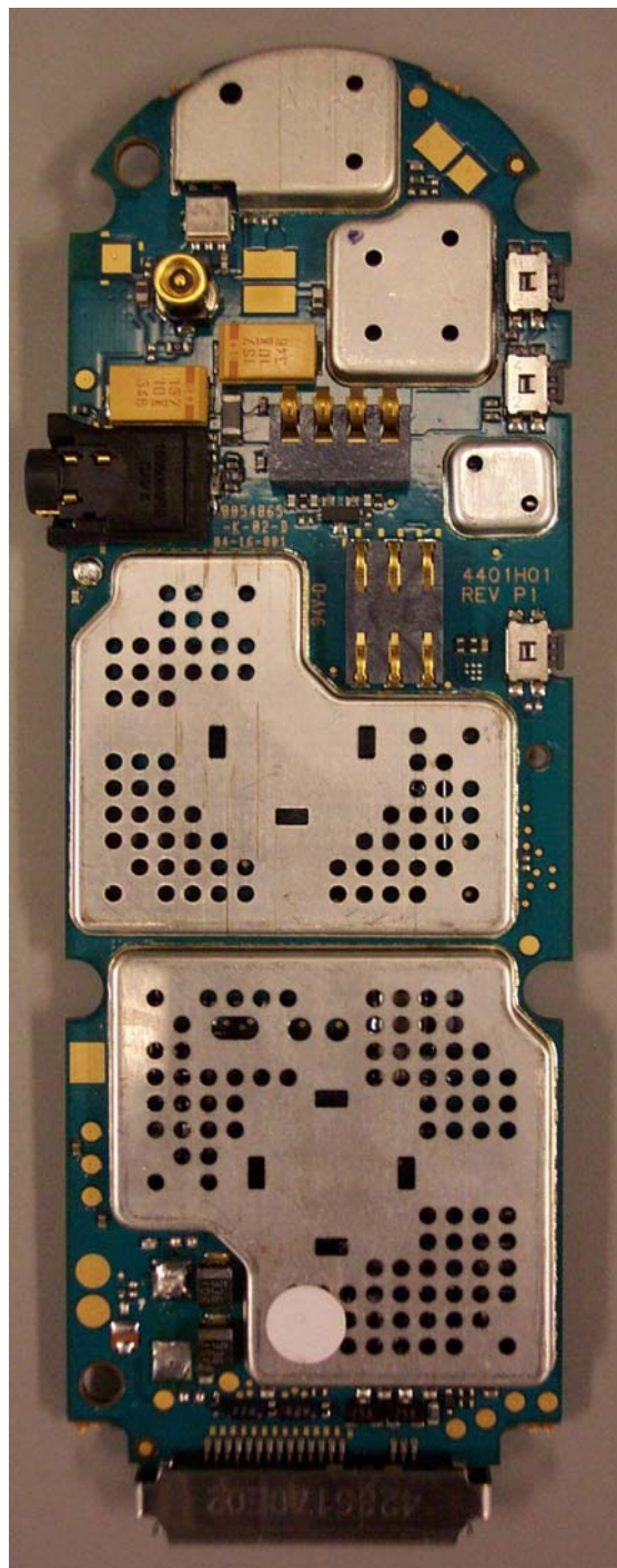
Photograph 9-2: Back side view of radio PCB.
