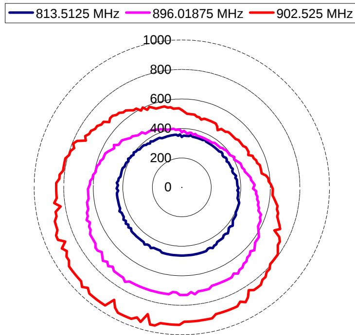
Figure 6-38: Land mobile Band: Scaled Maximum ERP(mW) vs. Azimuth Angle
