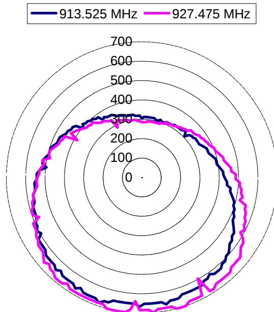
Figure 6-39: ISM Band: Scaled Maximum ERP(mW) vs. Azimuth Angle
