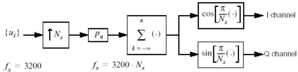
Figure 6-23. FSK Modulator
