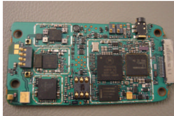
Photograph 9-4: Back side view of radio PCB without shields.
