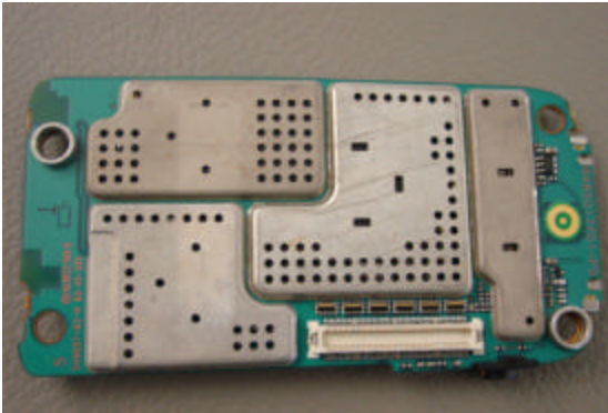
Photograph 9-1: Front side view of radio PCB.
