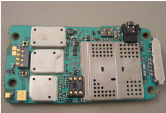
Photograph 9-2: Back side view of radio PCB.
