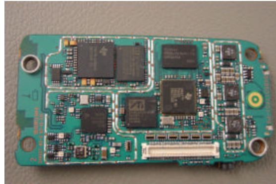
Photograph 9-3: Front side view of radio PCB without shields.
