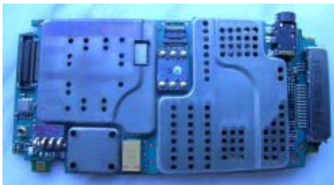
Photograph 9-1: Back side view of radio PCB.
