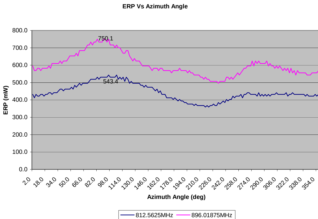
Figure 6-37: Scaled ERP vs. Azimuth Angle
