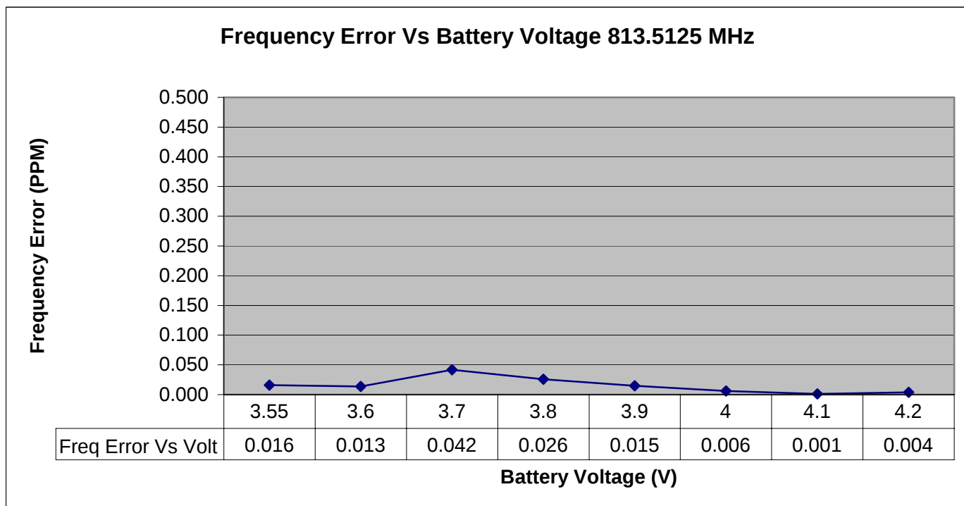
Figure 6-33: Transmitter Frequency Stability (800 MHz band) - Frequency Error vs. Voltage
