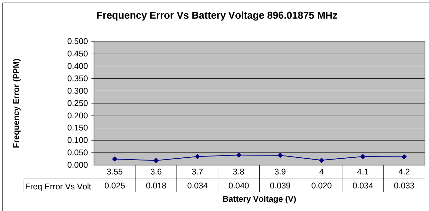
Figure 6-34: Transmitter Frequency Stability (900 MHz band)- Frequency Error vs. Voltage
