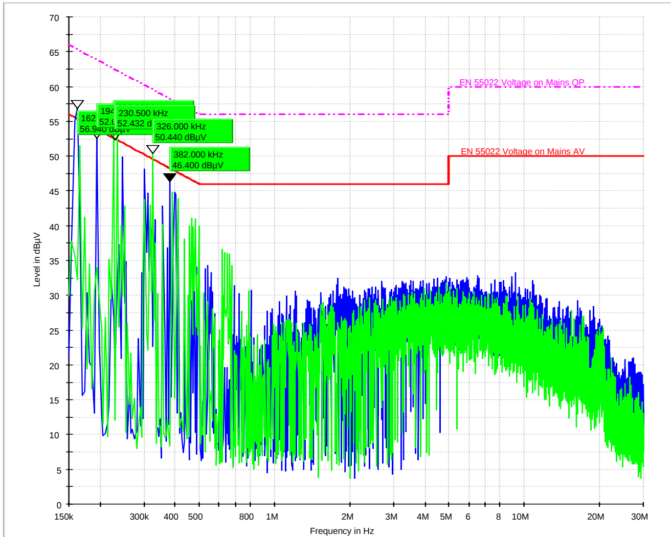
Figure 6-36: Neutral Line Voltage with a Peak and Average detector (Radio in transmit mode at 806.0625 MHz)
