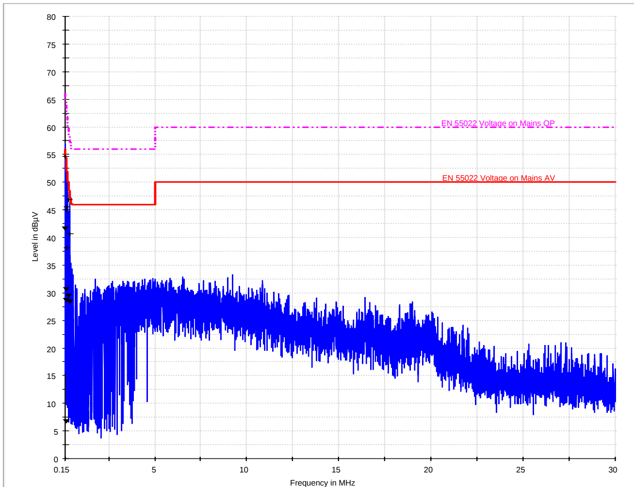
Figure 6-35: Phase Line Voltage with a Peak and Average Detector (Radio in transmit mode at 806.0625 MHz)
