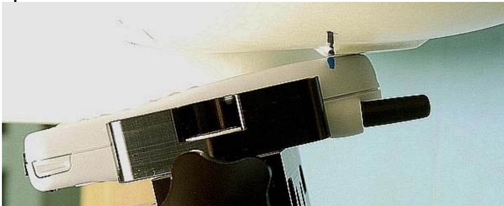
Figure 3. Assessment @ the Left ear; 15° tilt position; with antenna retracted. Same position used for antenna extended.
