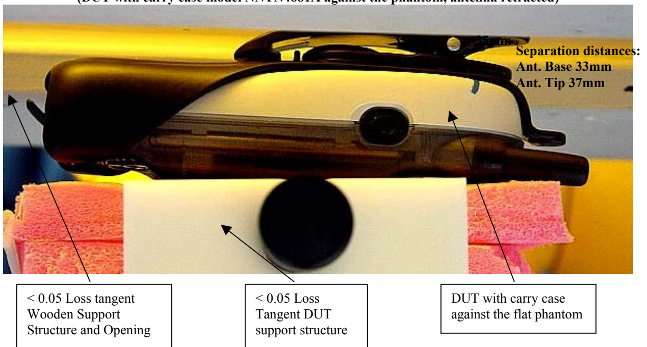
Figure 1: Highest S.A.R. Test Position (@ the Abdomen) (DUT with carry case model NNTN4681A against the phantom, antenna retracted)
