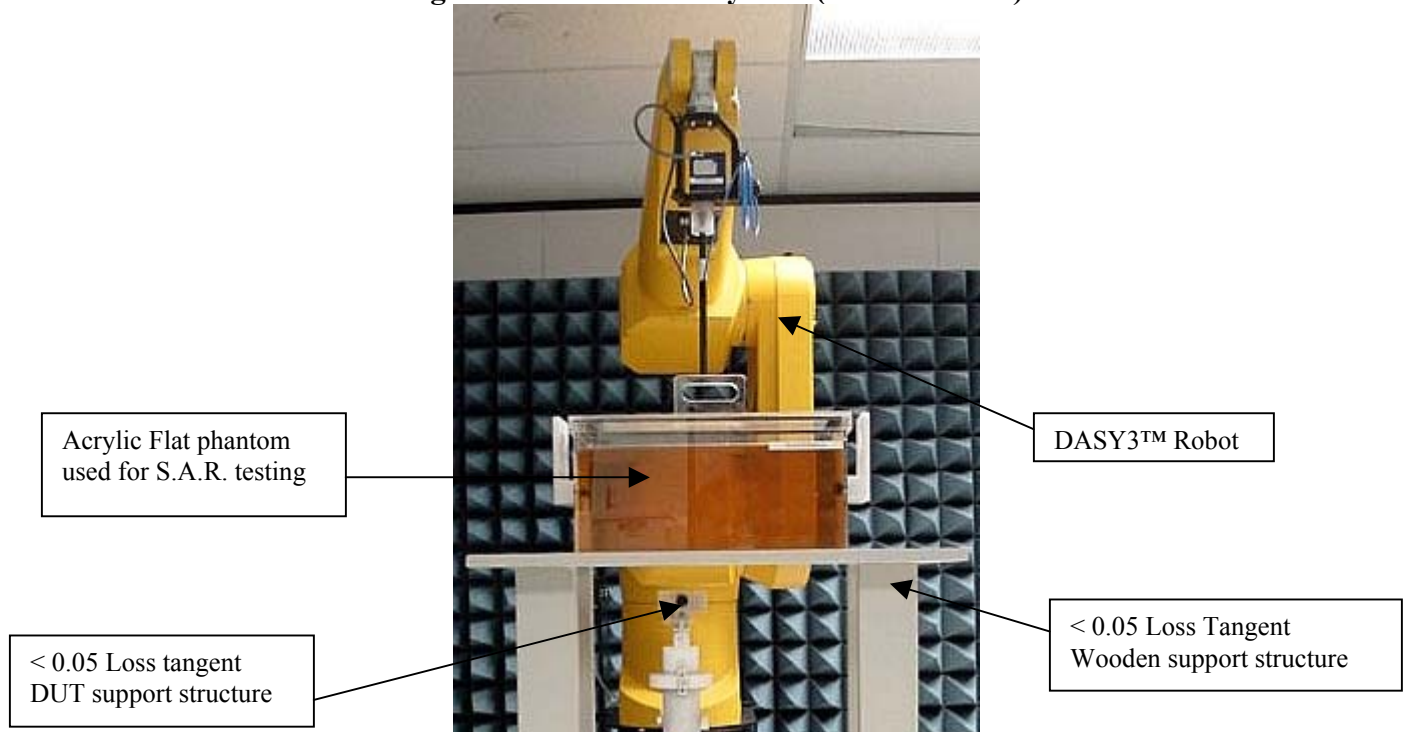
Figure 10: Robot Test System (Flat Phantom)
