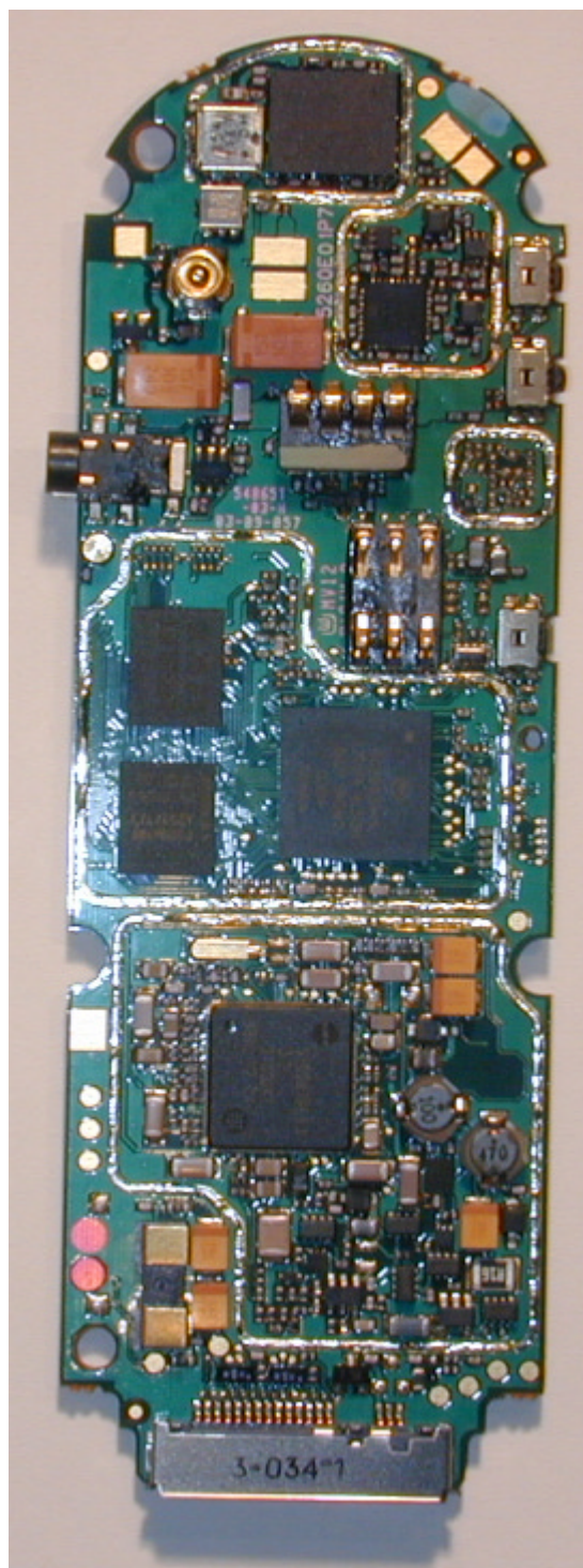
Photograph 9-4: Back side view of radio PCB without factory applied shields.
