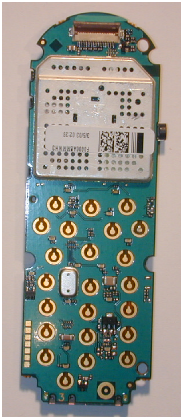
Photograph 9-1: Front side view of radio PCB.
