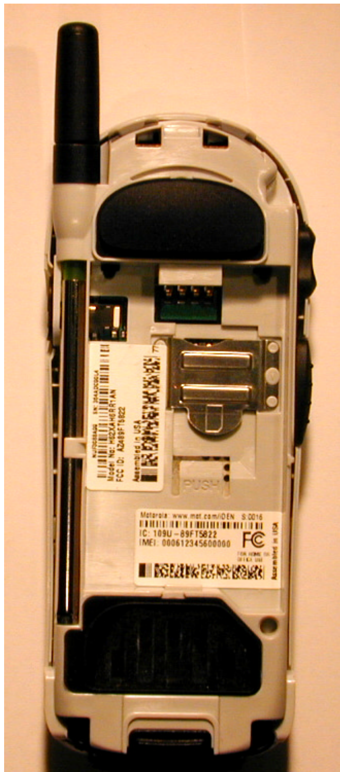
Photograph 3-6: Back view, antenna retracted, battery cover removed.
